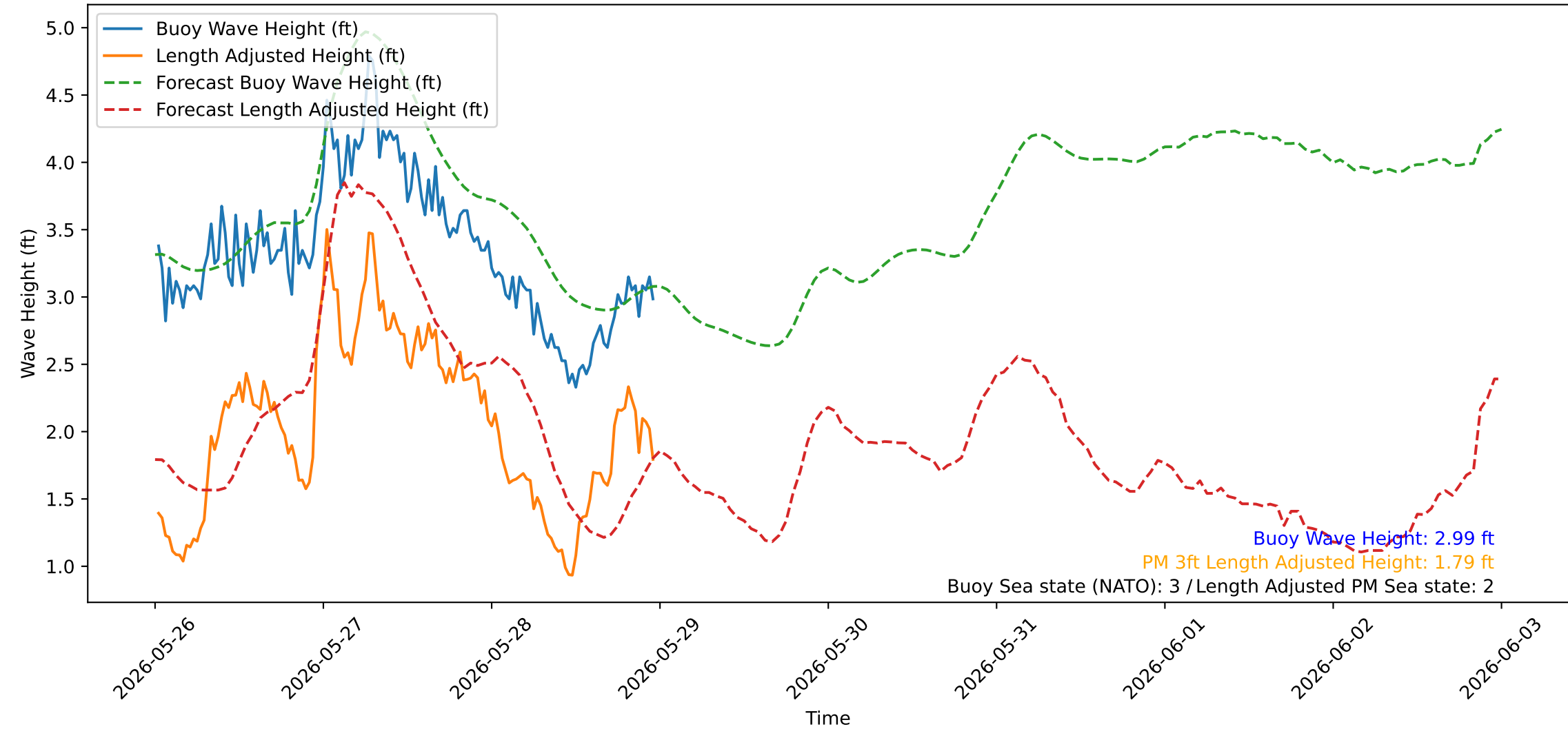
Wave Heights over Time for Red Beach at 2026-05-29 00:10:40
