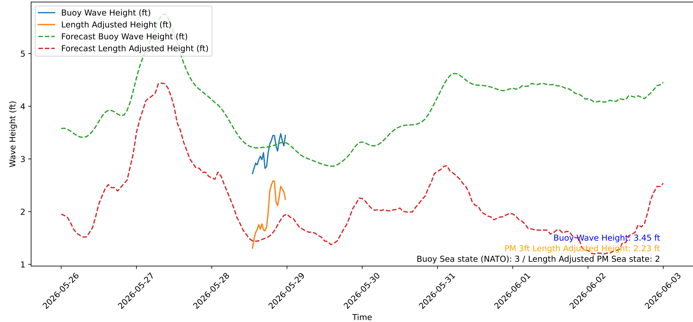
Wave Heights over Time for Oceanside Harbor at 2026-05-29 00:10:20
