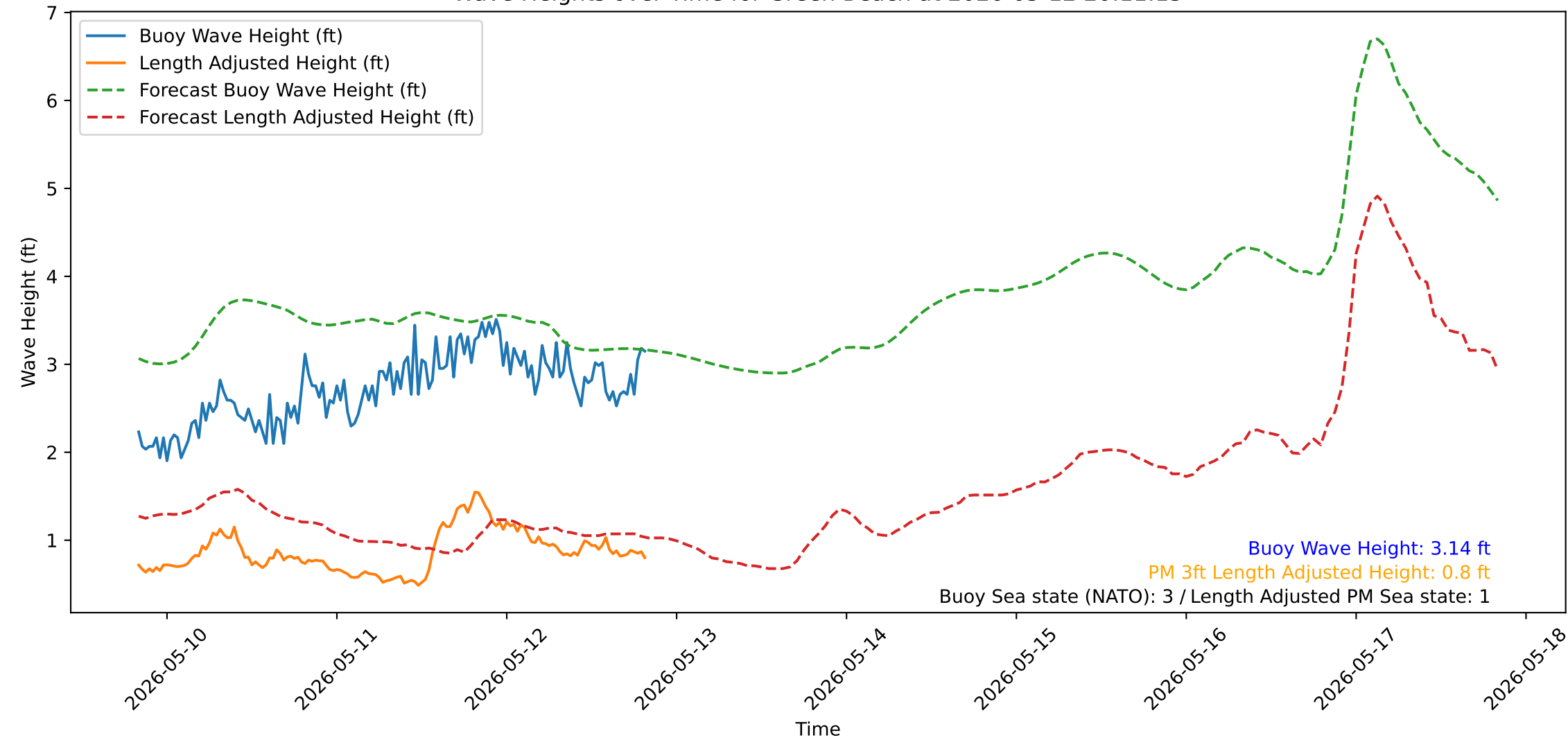
Wave Heights over Time for Green Beach at 2026-05-12 20:11:13
