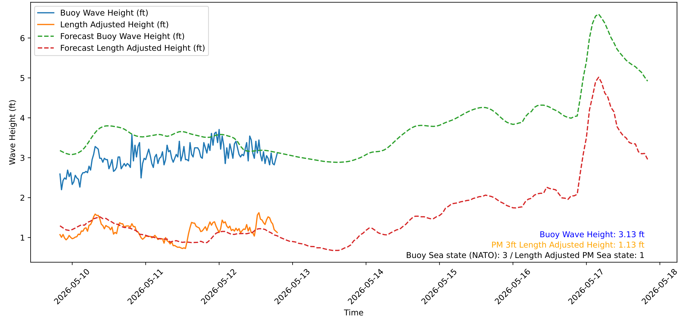
Wave Heights over Time for Oceanside Harbor at 2026-05-12 20:10:32
