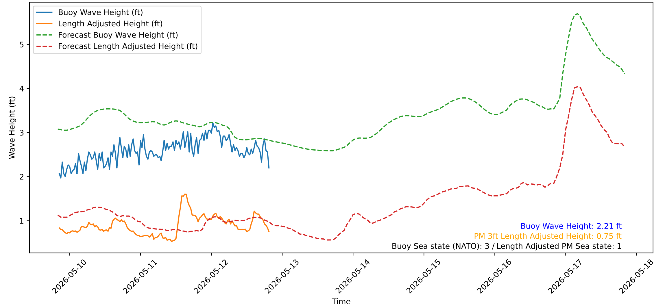
Wave Heights over Time for Red Beach at 2026-05-12 20:10:51
