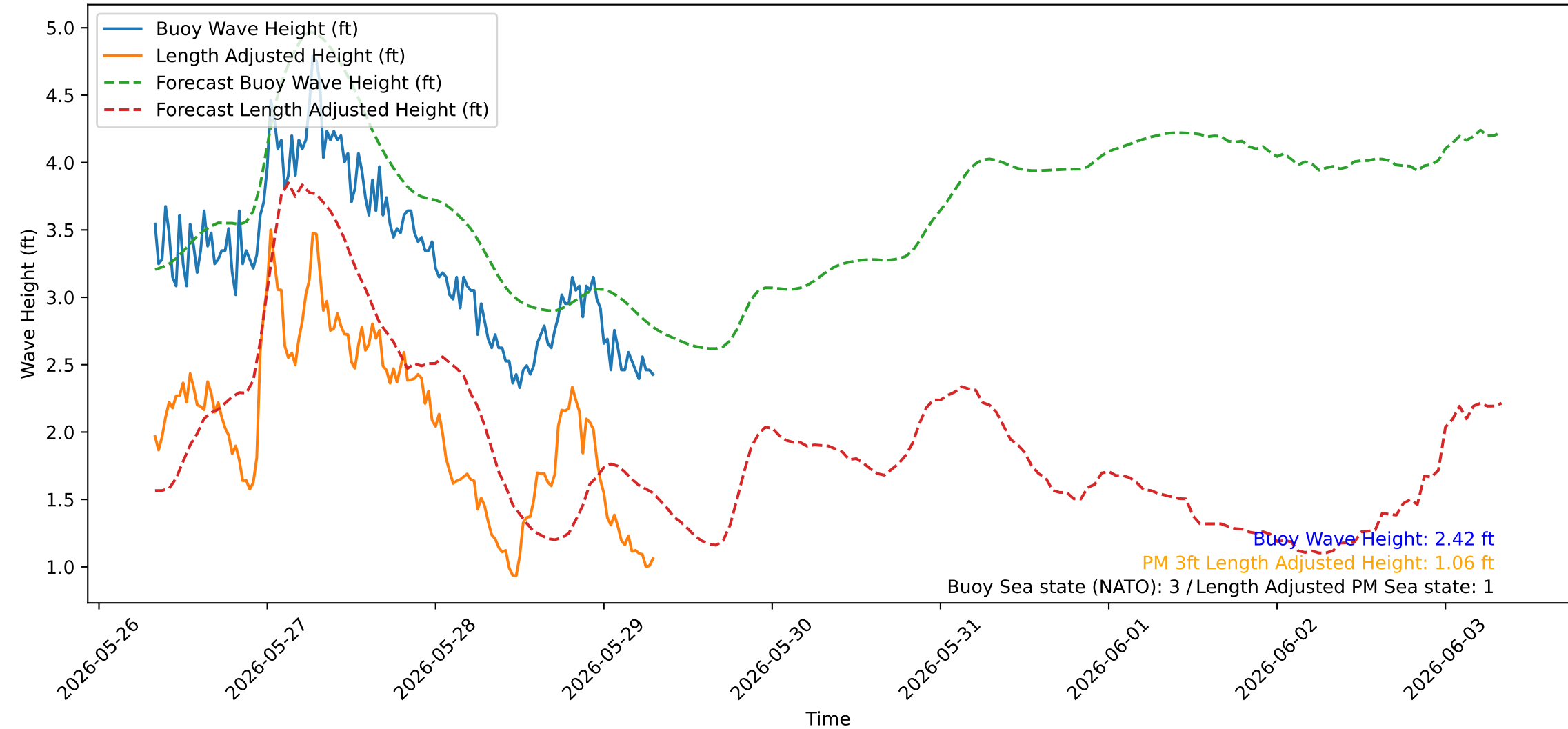
Wave Heights over Time for Red Beach at 2026-05-29 07:50:41
