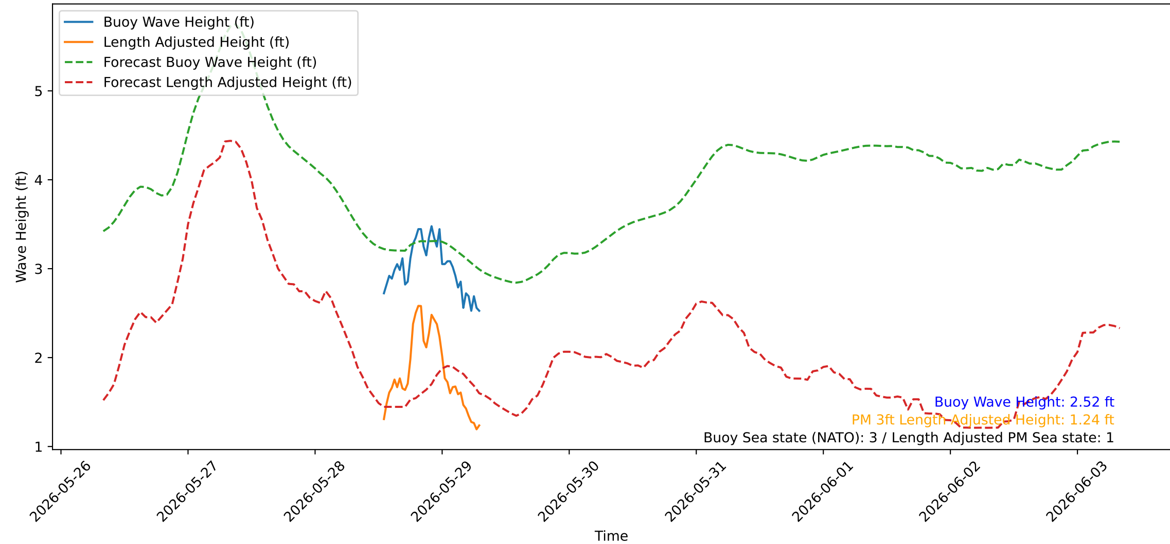
Wave Heights over Time for Oceanside Harbor at 2026-05-29 07:50:21
