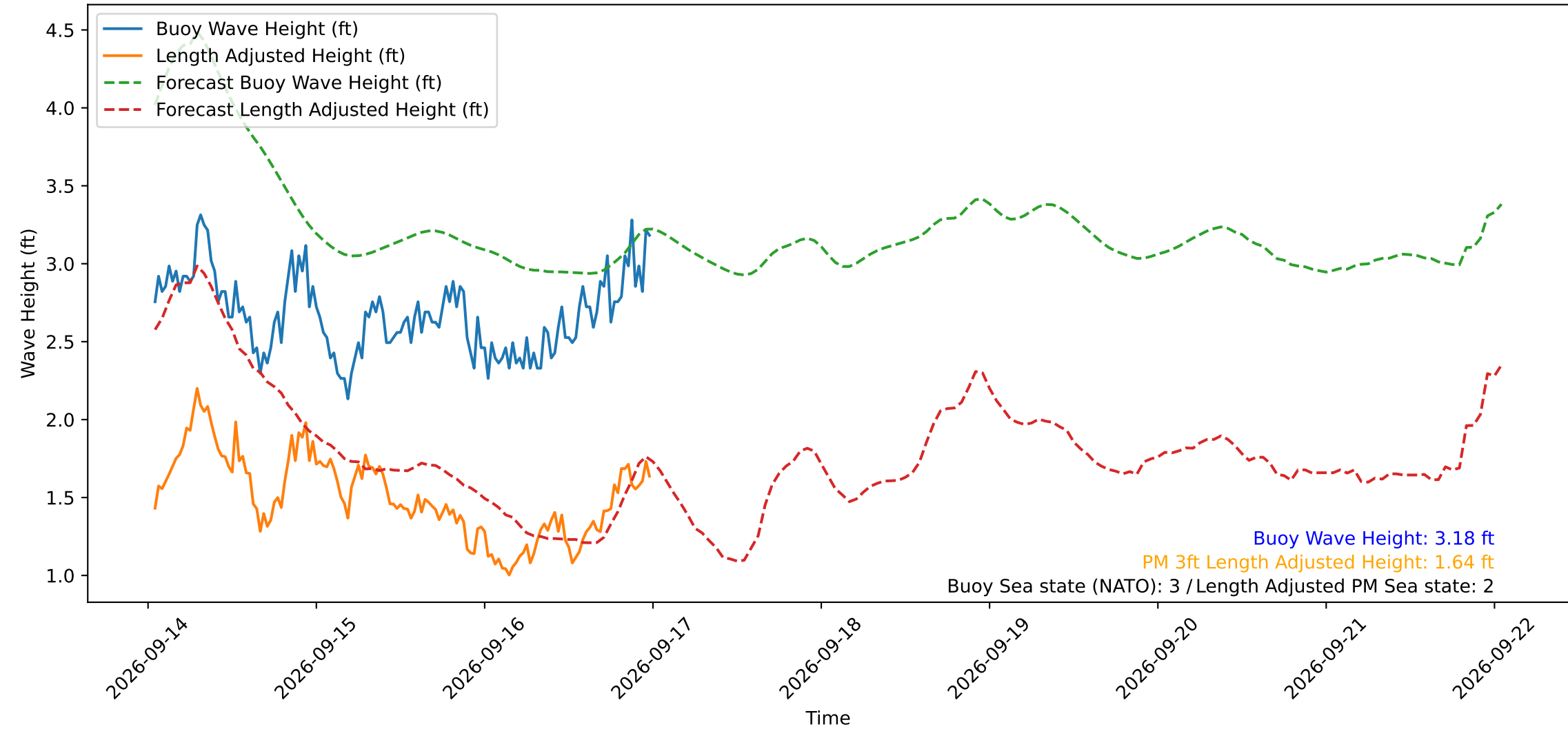
Wave Heights over Time for Green Beach at 2026-09-17 00:41:12
