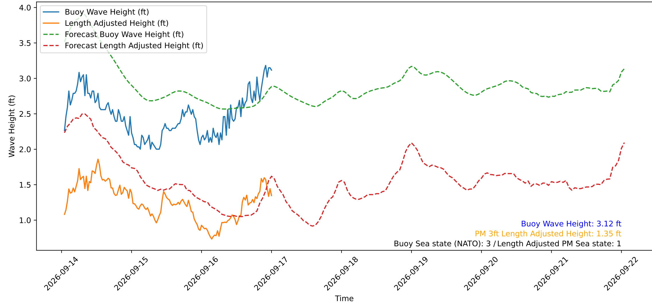
Wave Heights over Time for Red Beach at 2026-09-17 00:40:49
