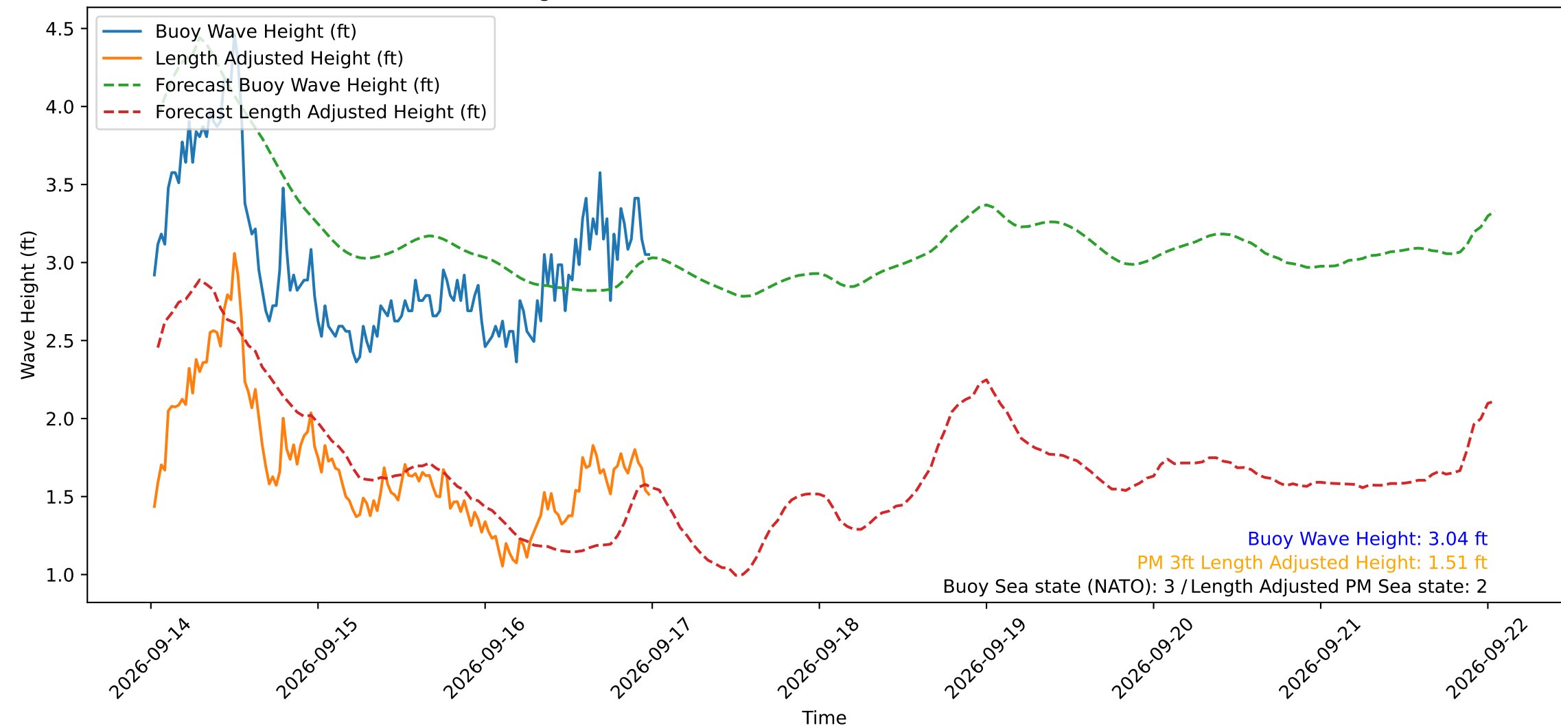
Wave Heights over Time for Oceanside Harbor at 2026-09-17 00:40:29
