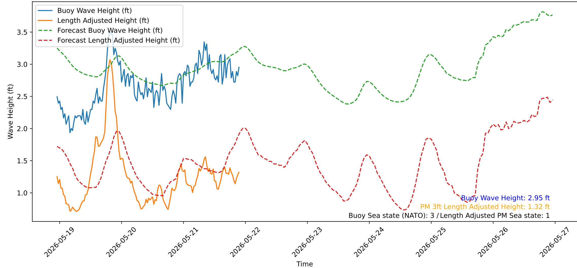
Wave Heights over Time for Red Beach at 2026-05-21 22:50:52
