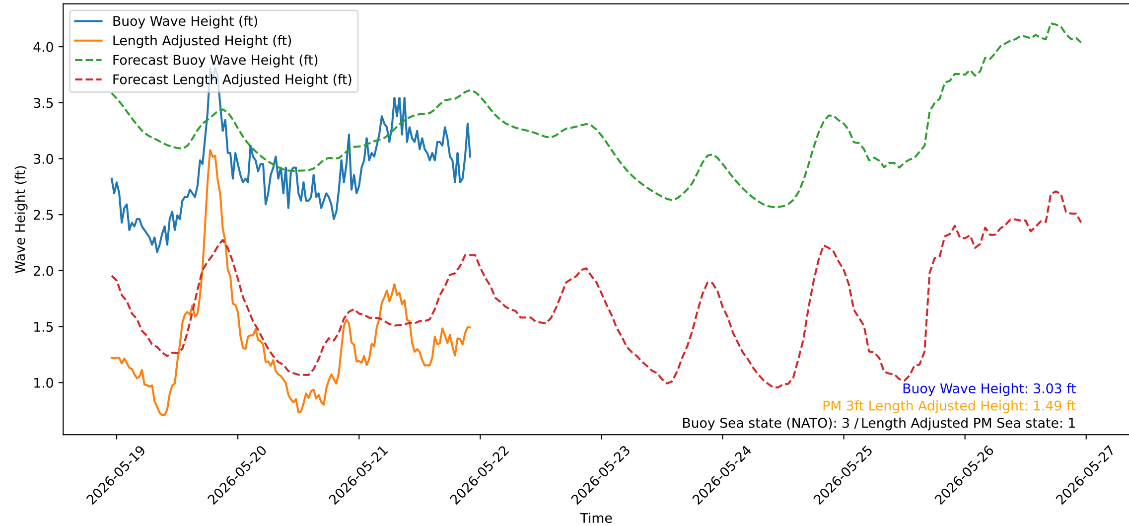
Wave Heights over Time for Green Beach at 2026-05-21 22:51:14
