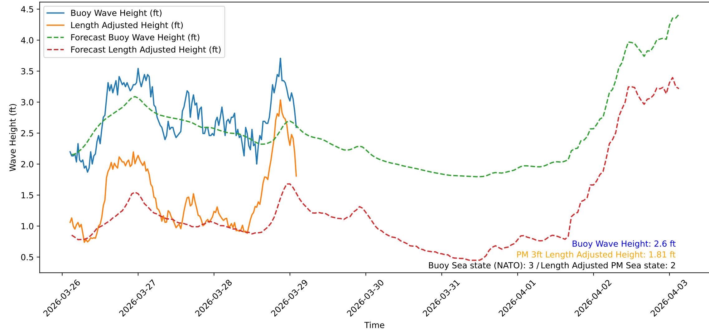
Wave Heights over Time for Green Beach at 2026-03-29 02:41:10
