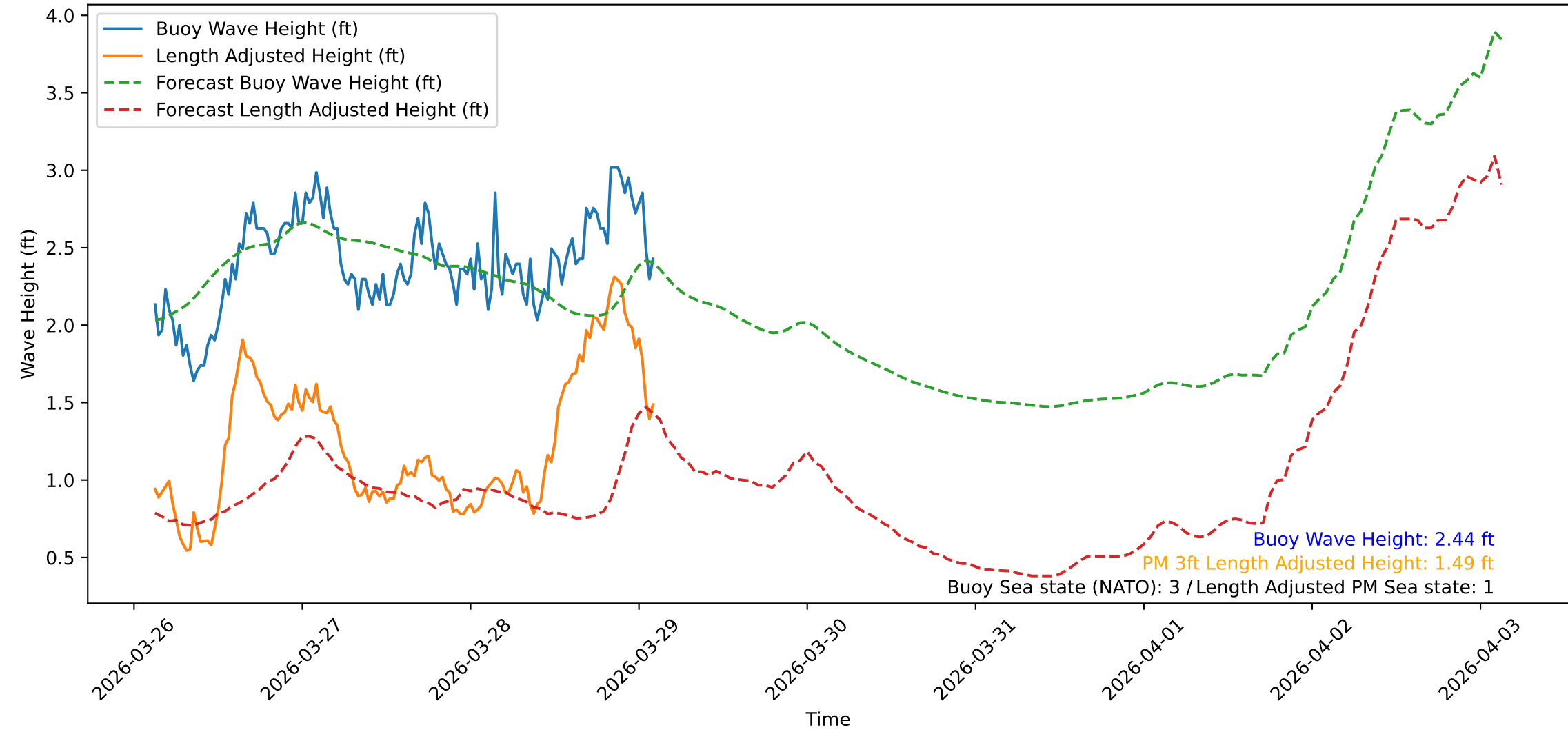
Wave Heights over Time for Red Beach at 2026-03-29 02:40:48
