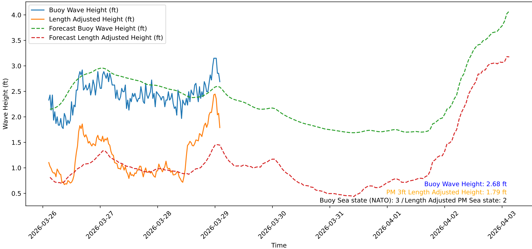
Wave Heights over Time for Oceanside Harbor at 2026-03-29 02:40:31
