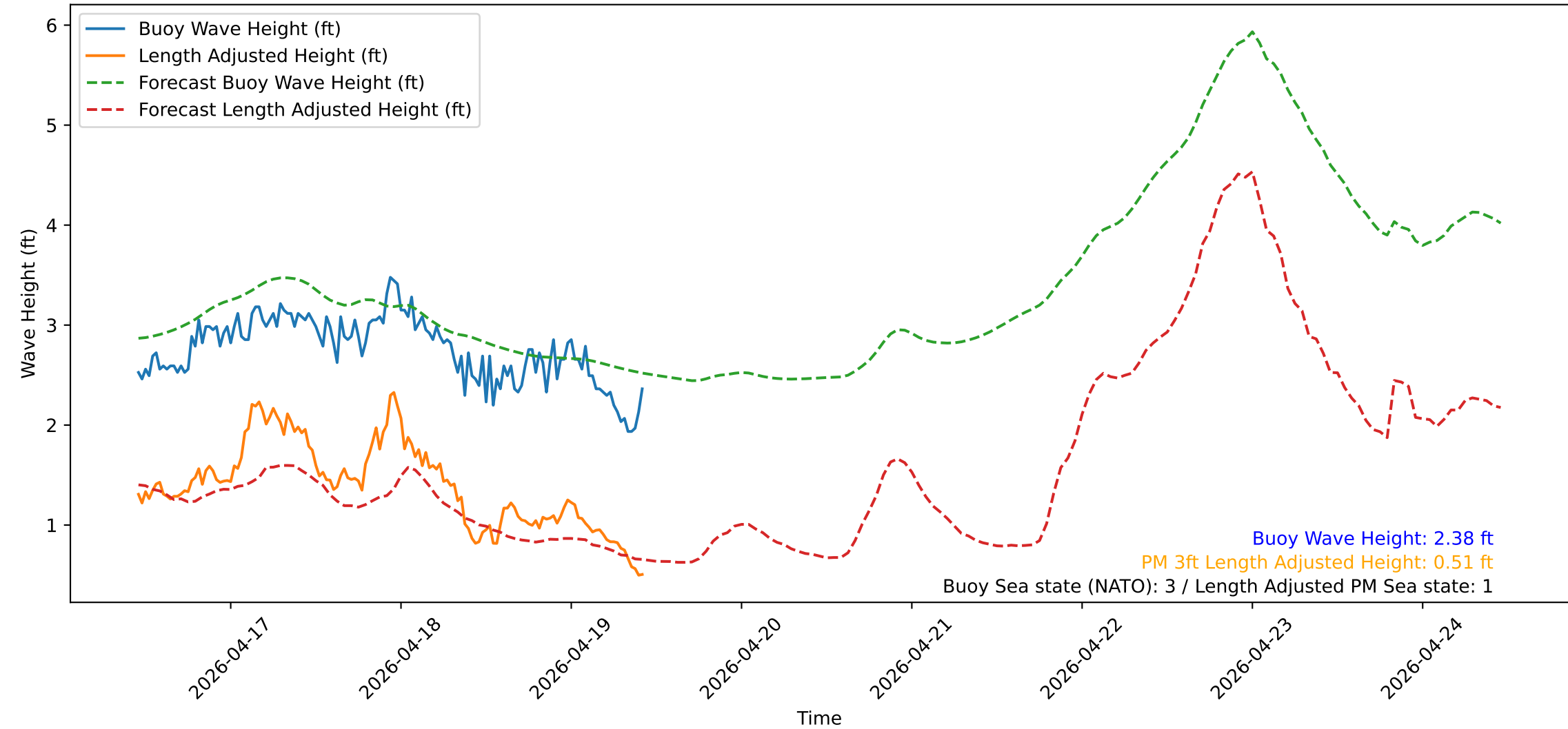
Wave Heights over Time for Green Beach at 2026-04-19 10:51:17
