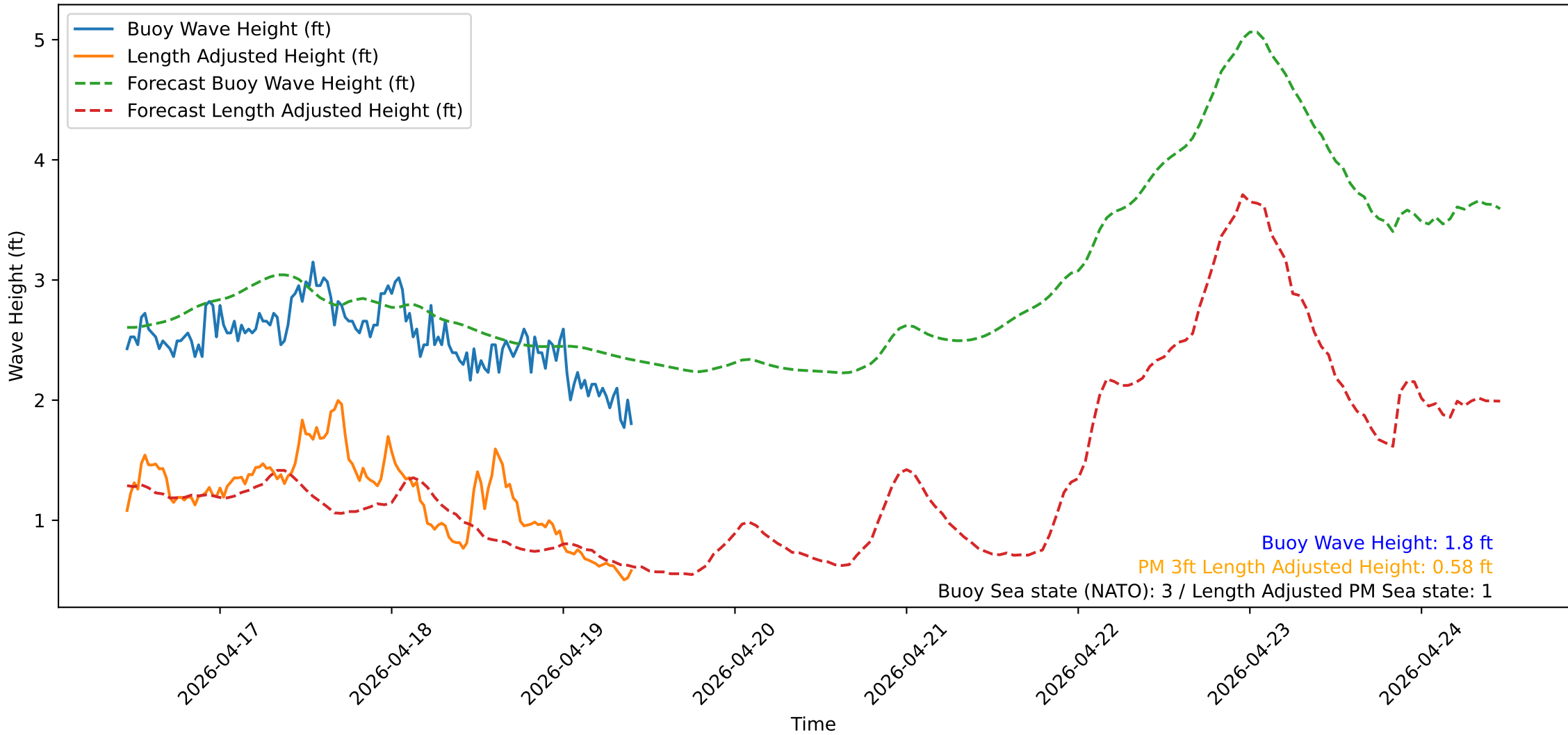
Wave Heights over Time for Red Beach at 2026-04-19 10:50:55
