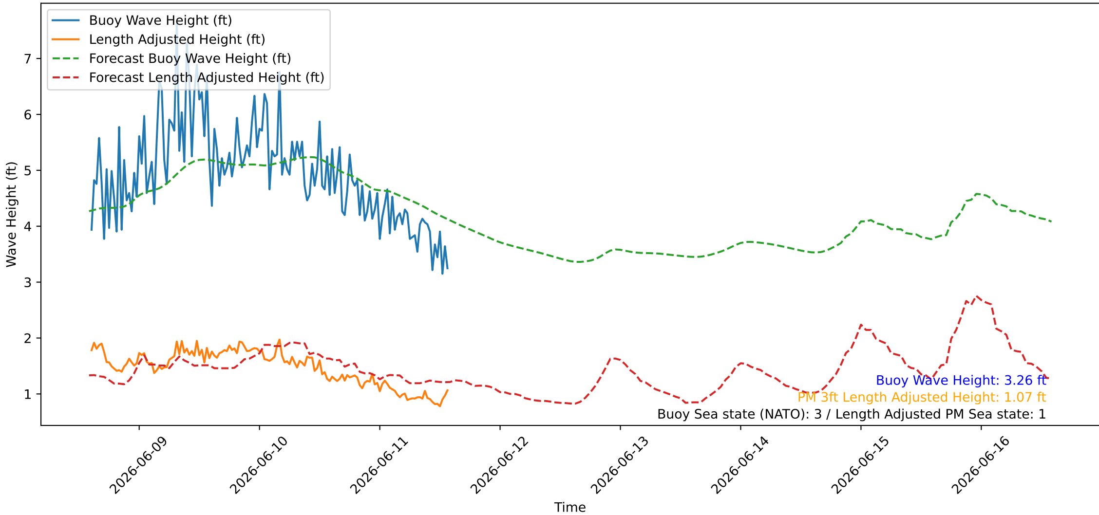
Wave Heights over Time for Red Beach at 2026-06-11 14:10:45
