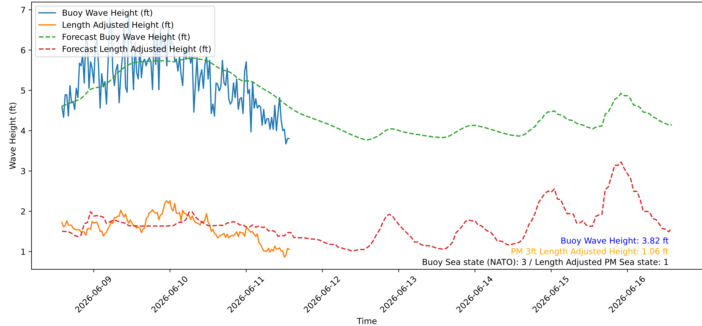
Wave Heights over Time for Green Beach at 2026-06-11 14:11:08
