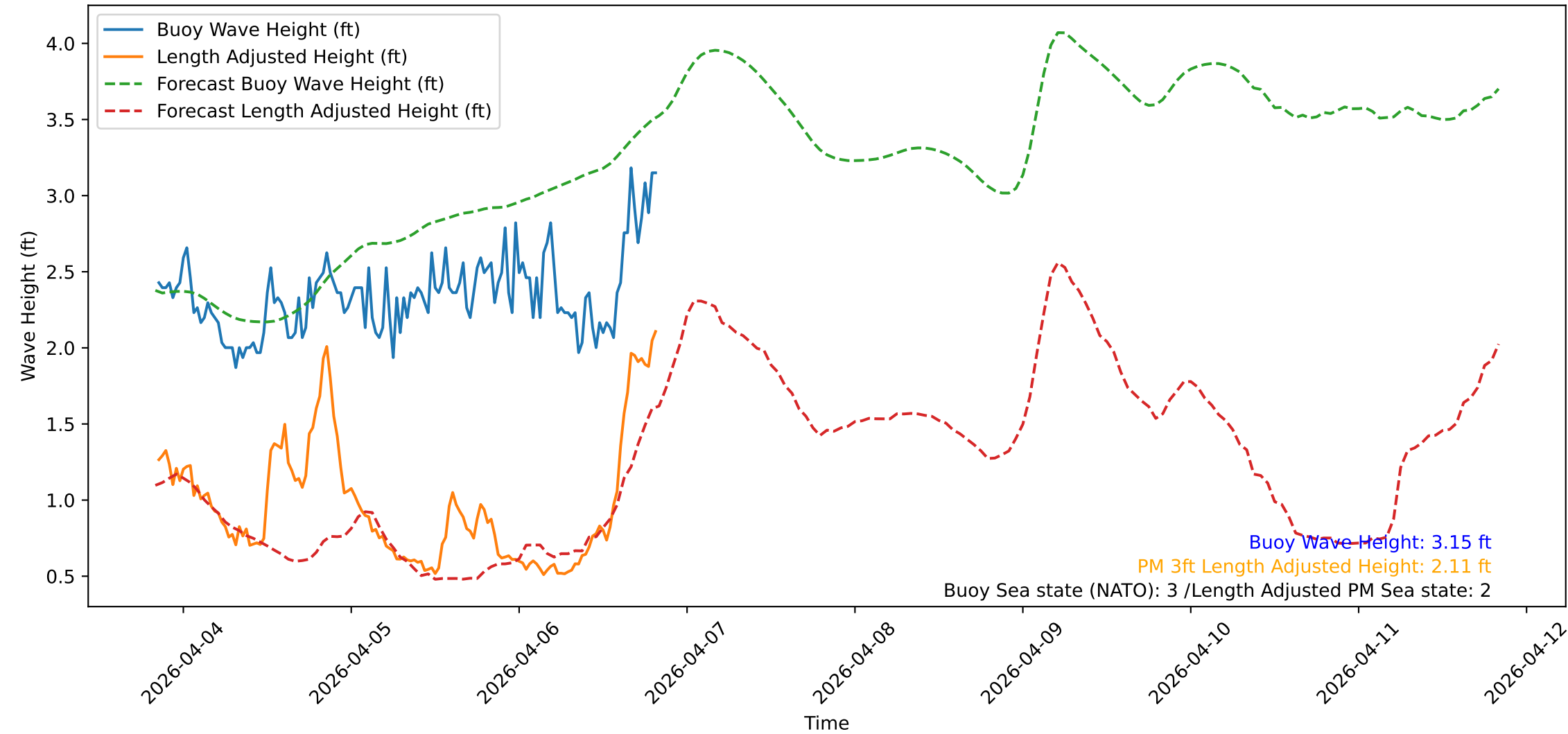
Wave Heights over Time for Red Beach at 2026-04-06 20:10:48
