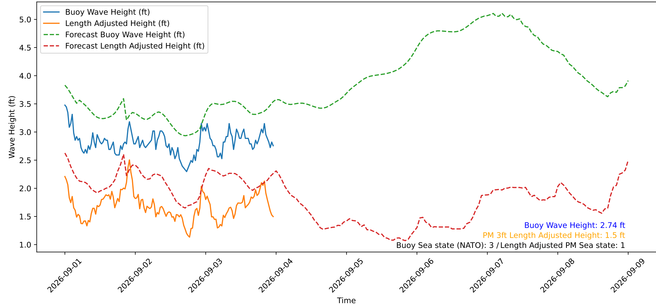
Wave Heights over Time for Red Beach at 2026-09-03 23:50:50
