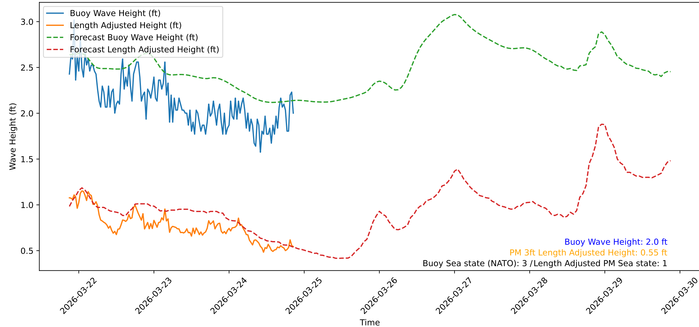
Wave Heights over Time for Oceanside Harbor at 2026-03-24 21:10:31
