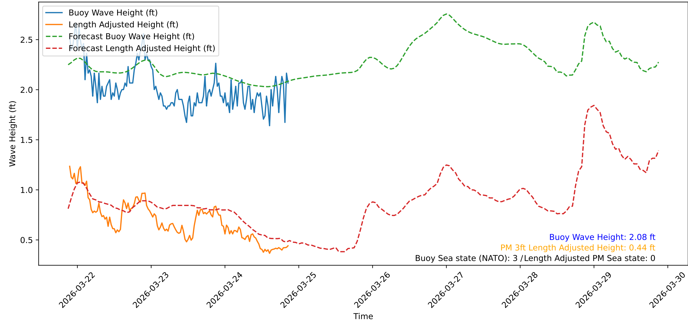
Wave Heights over Time for Red Beach at 2026-03-24 21:10:47
