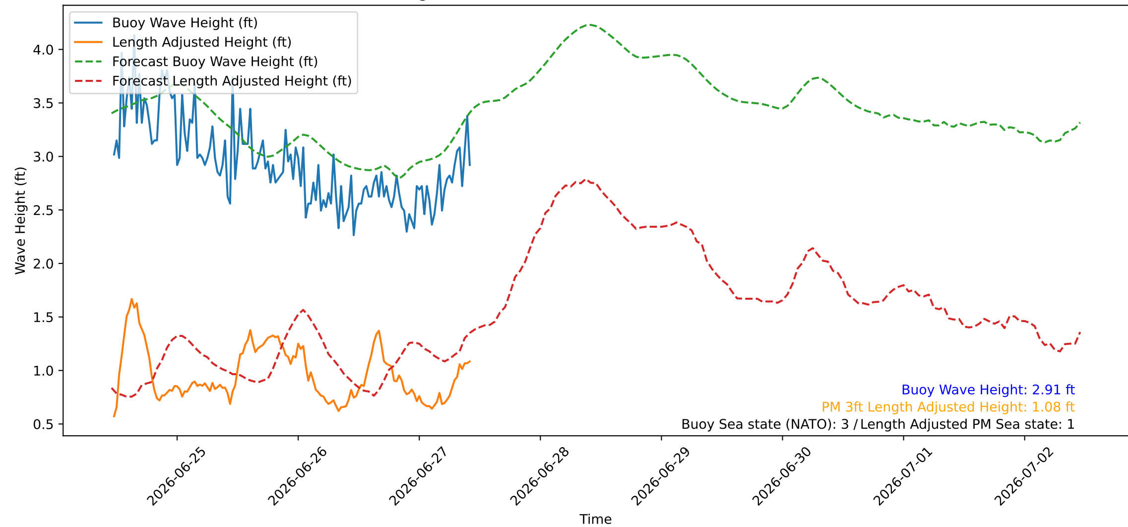
Wave Heights over Time for Red Beach at 2026-06-27 11:00:45
