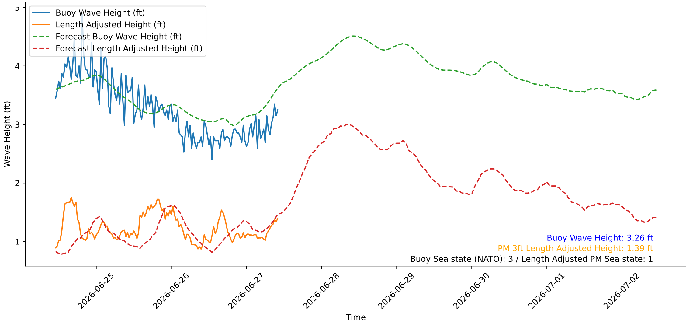
Wave Heights over Time for Oceanside Harbor at 2026-06-27 11:00:26
