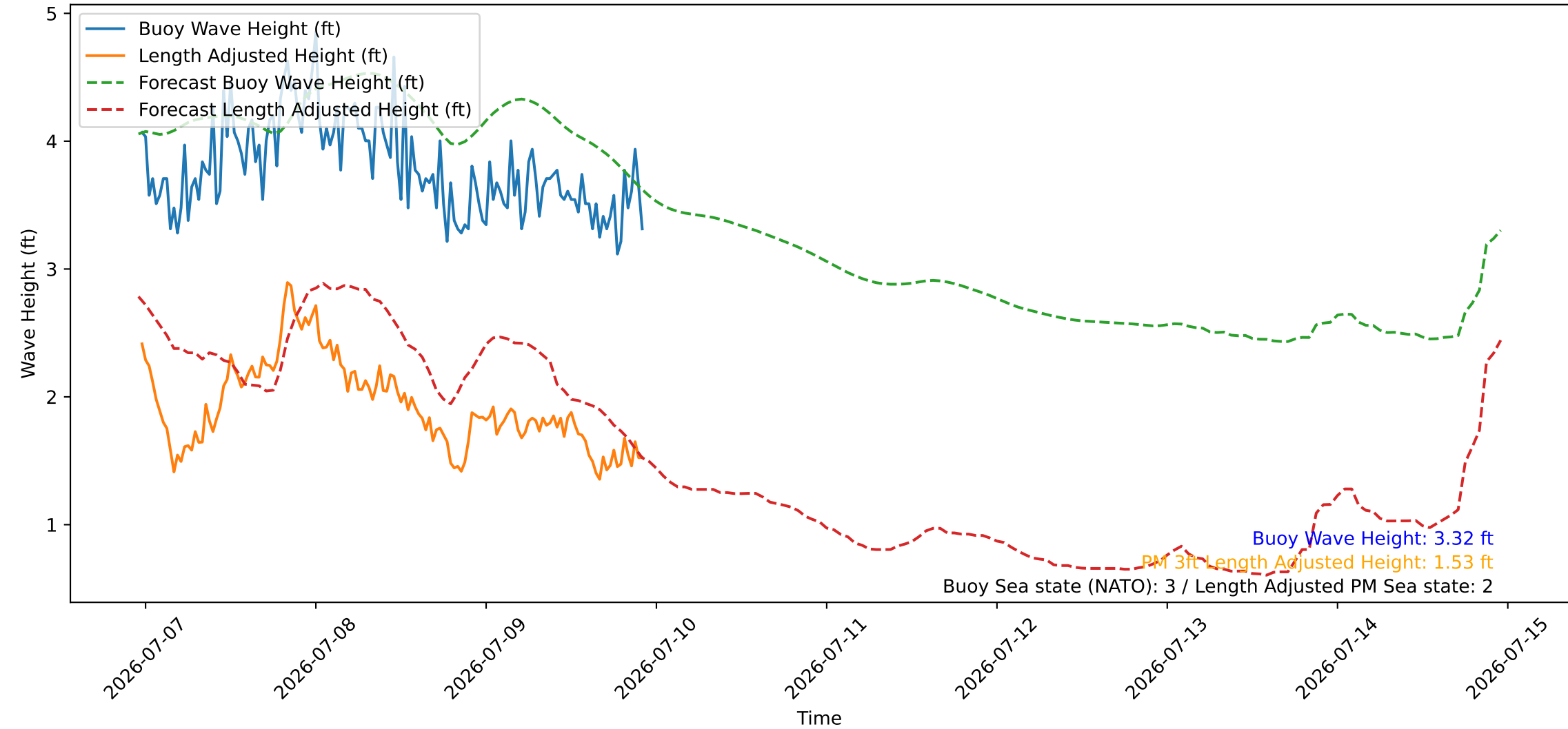
Wave Heights over Time for Red Beach at 2026-07-09 23:00:46
