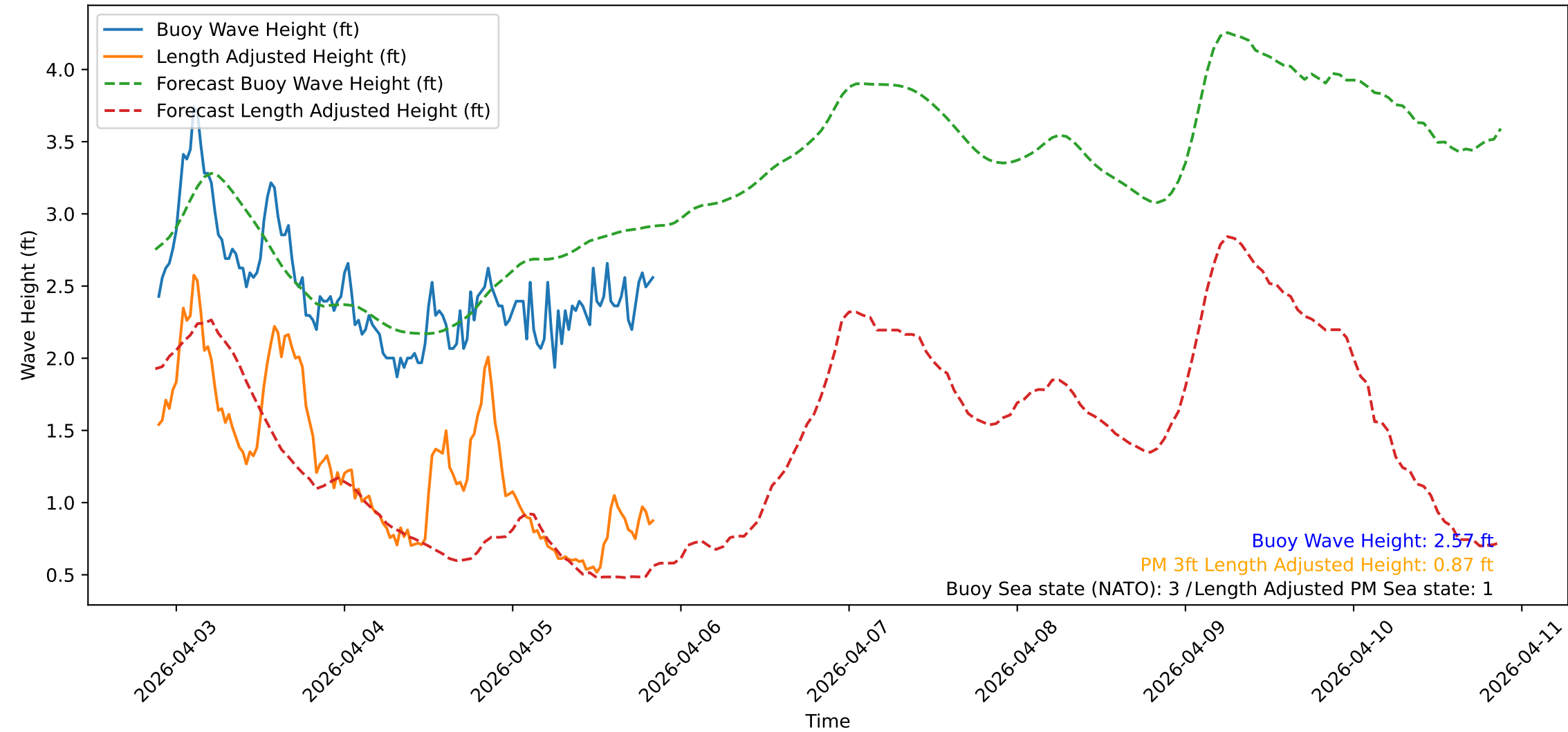
Wave Heights over Time for Red Beach at 2026-04-05 21:00:56
