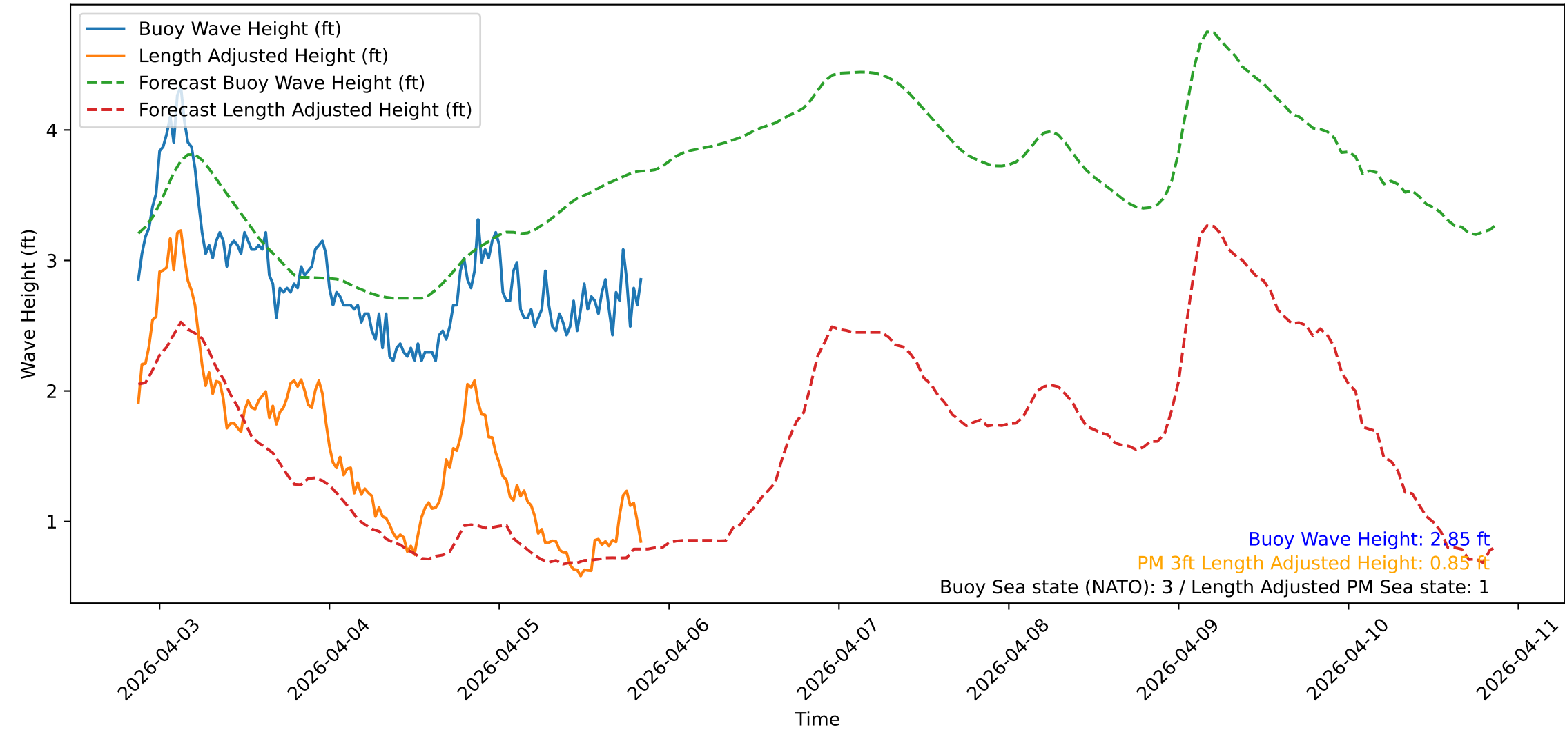
Wave Heights over Time for Green Beach at 2026-04-05 21:01:25
