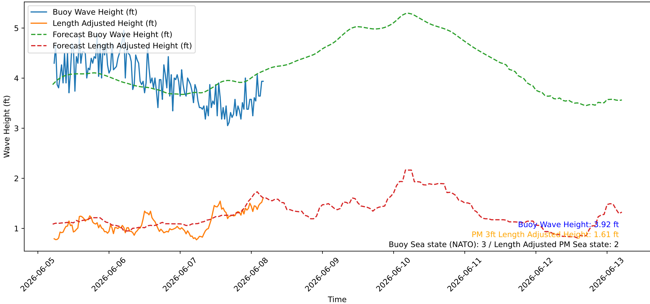
Wave Heights over Time for Red Beach at 2026-06-08 05:00:45
