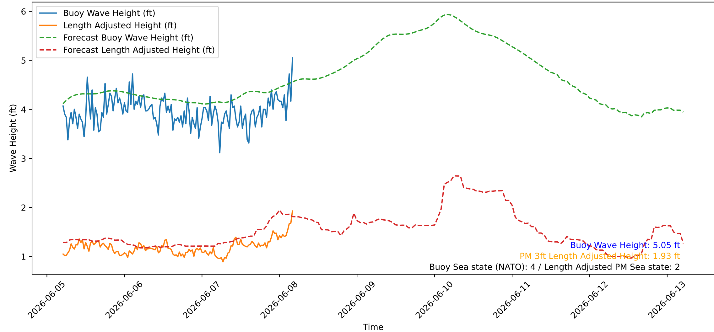
Wave Heights over Time for Green Beach at 2026-06-08 05:01:08
