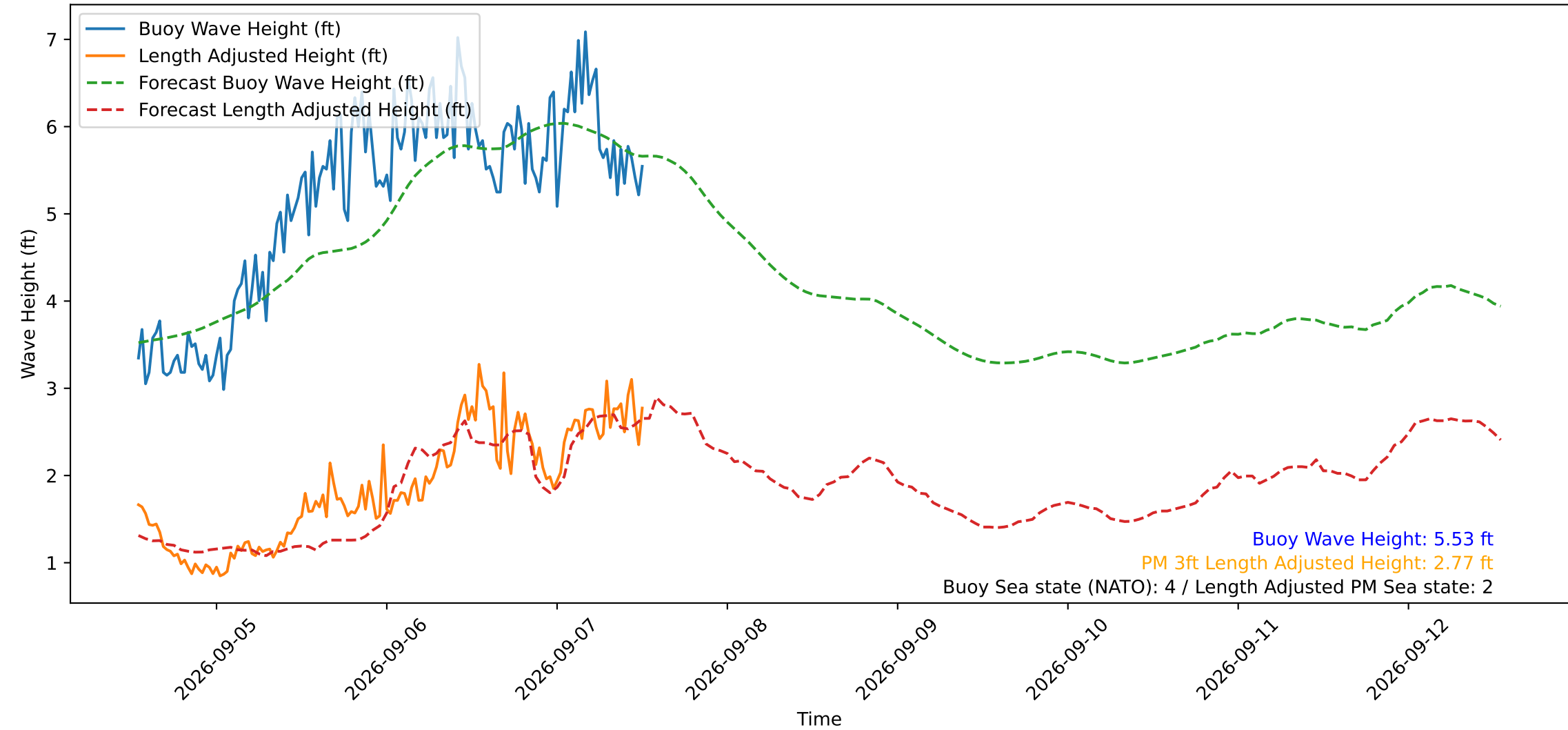
Wave Heights over Time for Oceanside Harbor at 2026-09-07 12:50:29
