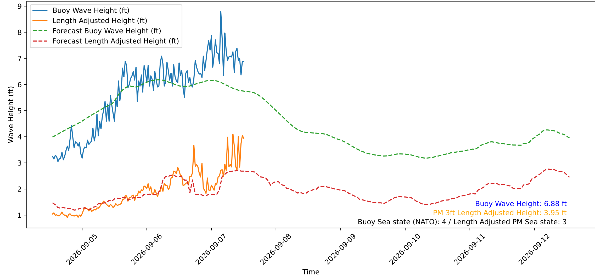
Wave Heights over Time for Green Beach at 2026-09-07 12:51:15
