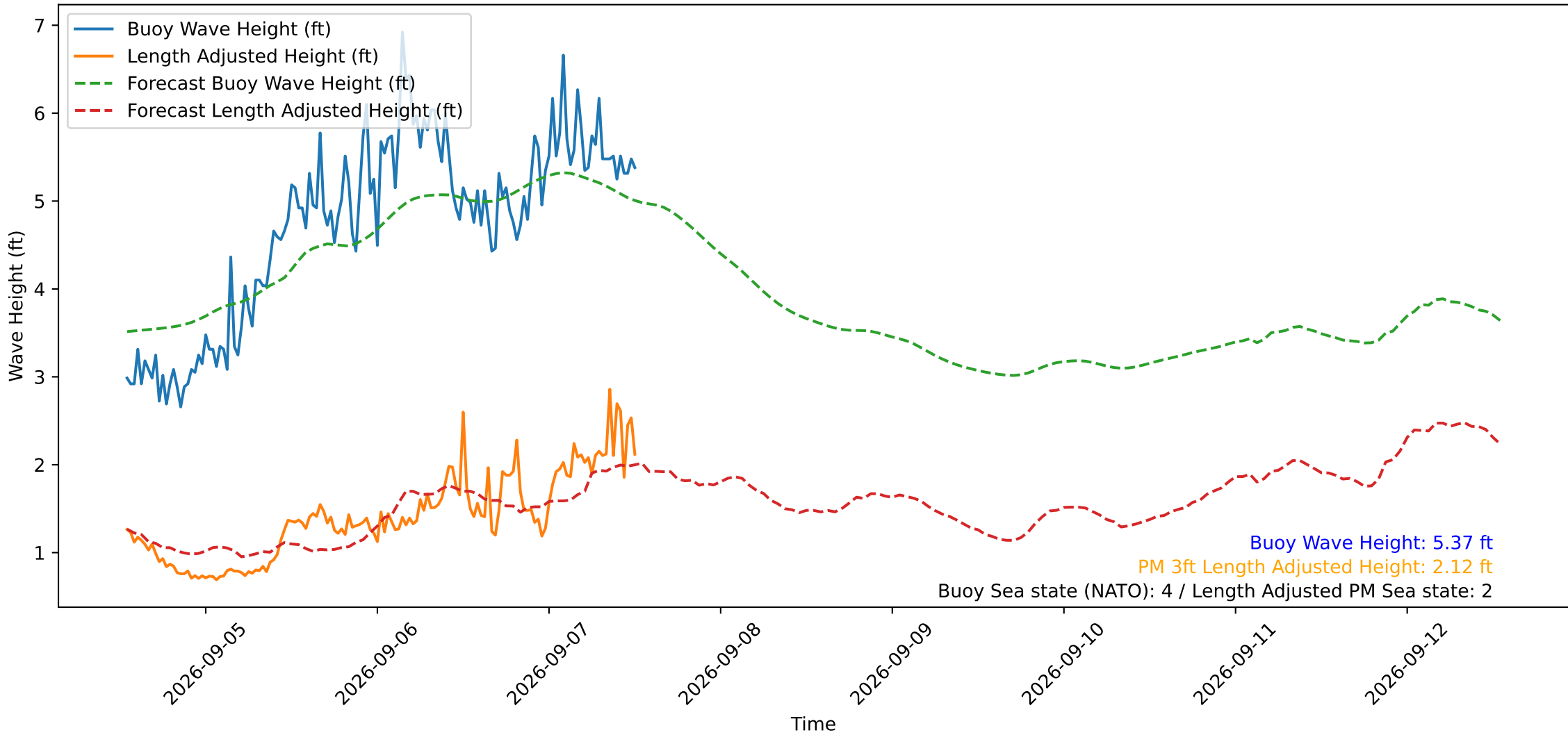
Wave Heights over Time for Red Beach at 2026-09-07 12:50:51
