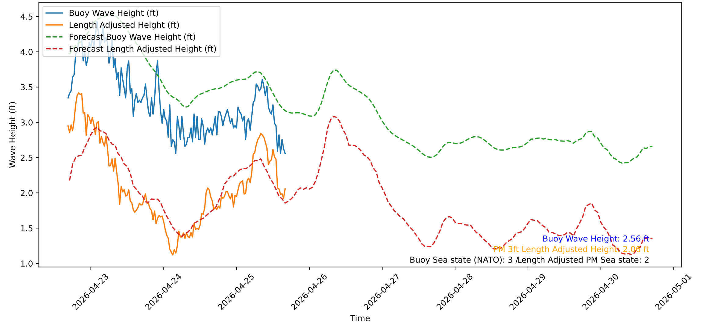
Wave Heights over Time for Oceanside Harbor at 2026-04-25 16:30:31
