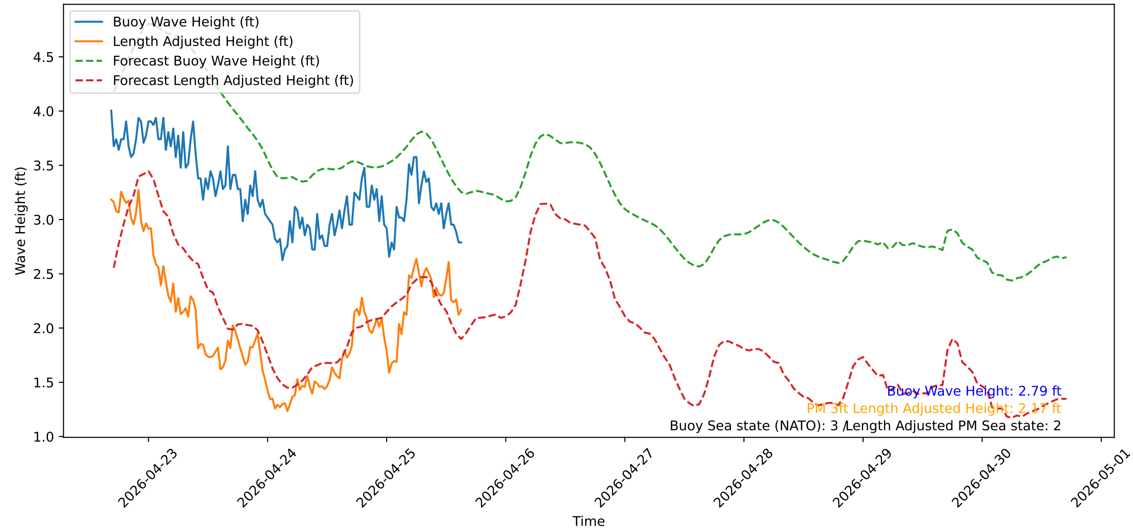
Wave Heights over Time for Green Beach at 2026-04-25 16:31:11
