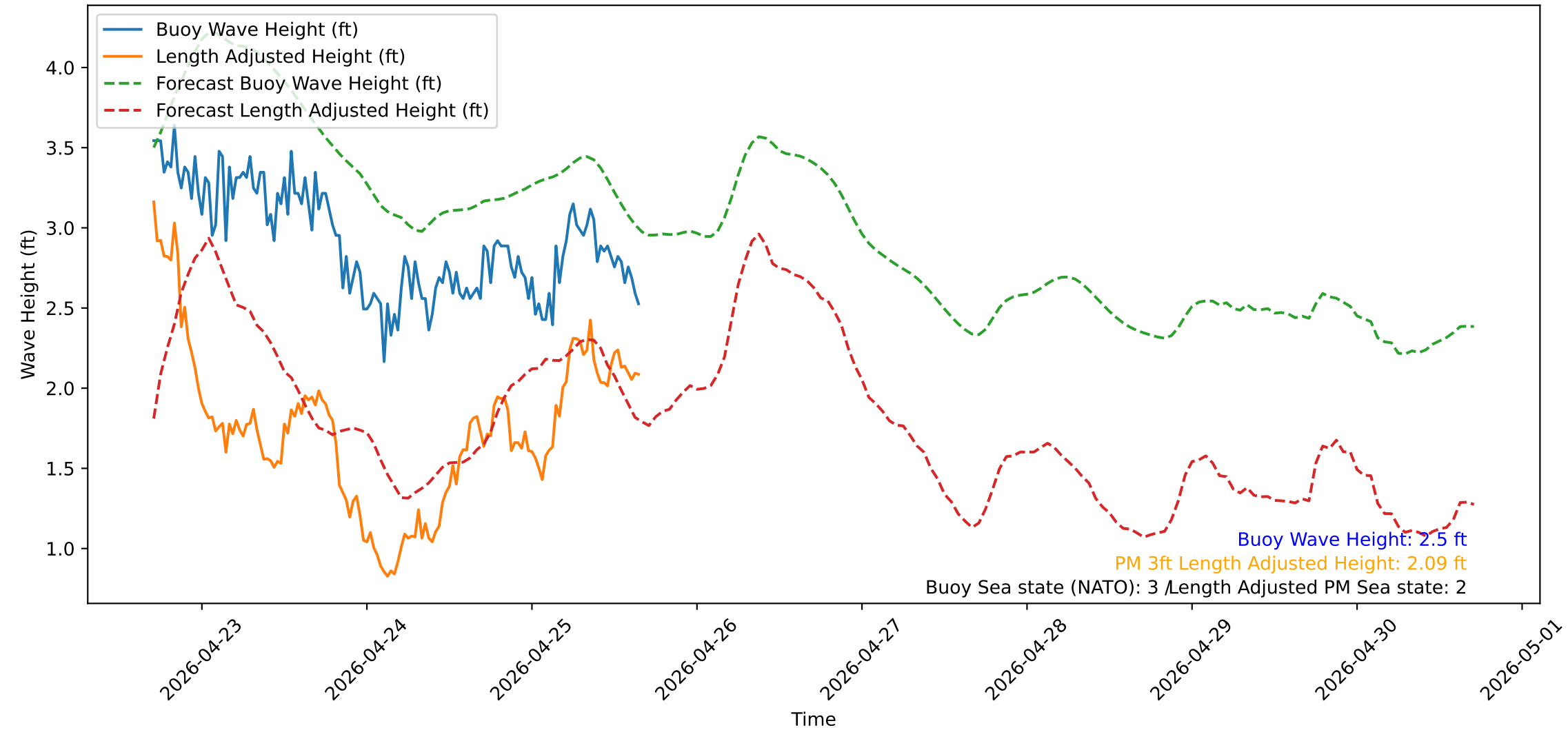
Wave Heights over Time for Red Beach at 2026-04-25 16:30:49
