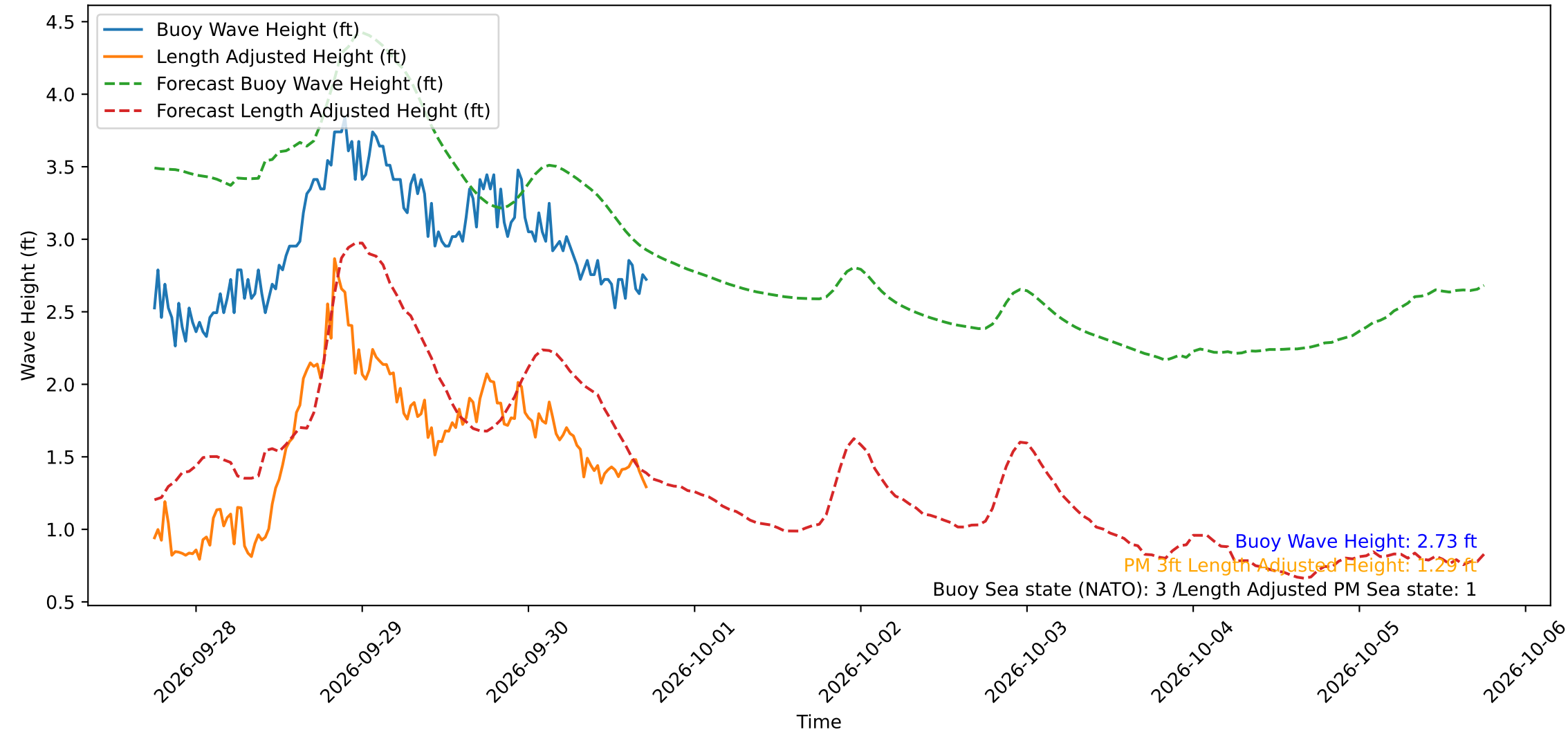
Wave Heights over Time for Red Beach at 2026-09-30 17:40:49
