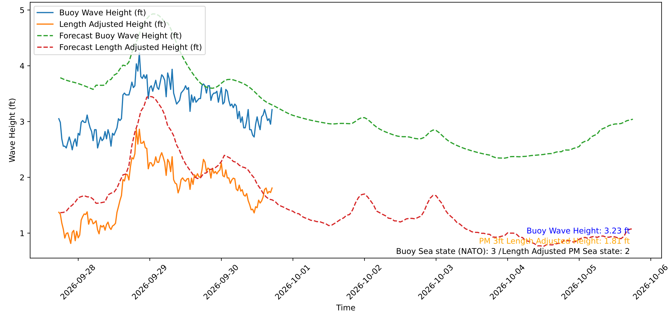
Wave Heights over Time for Oceanside Harbor at 2026-09-30 17:40:29
