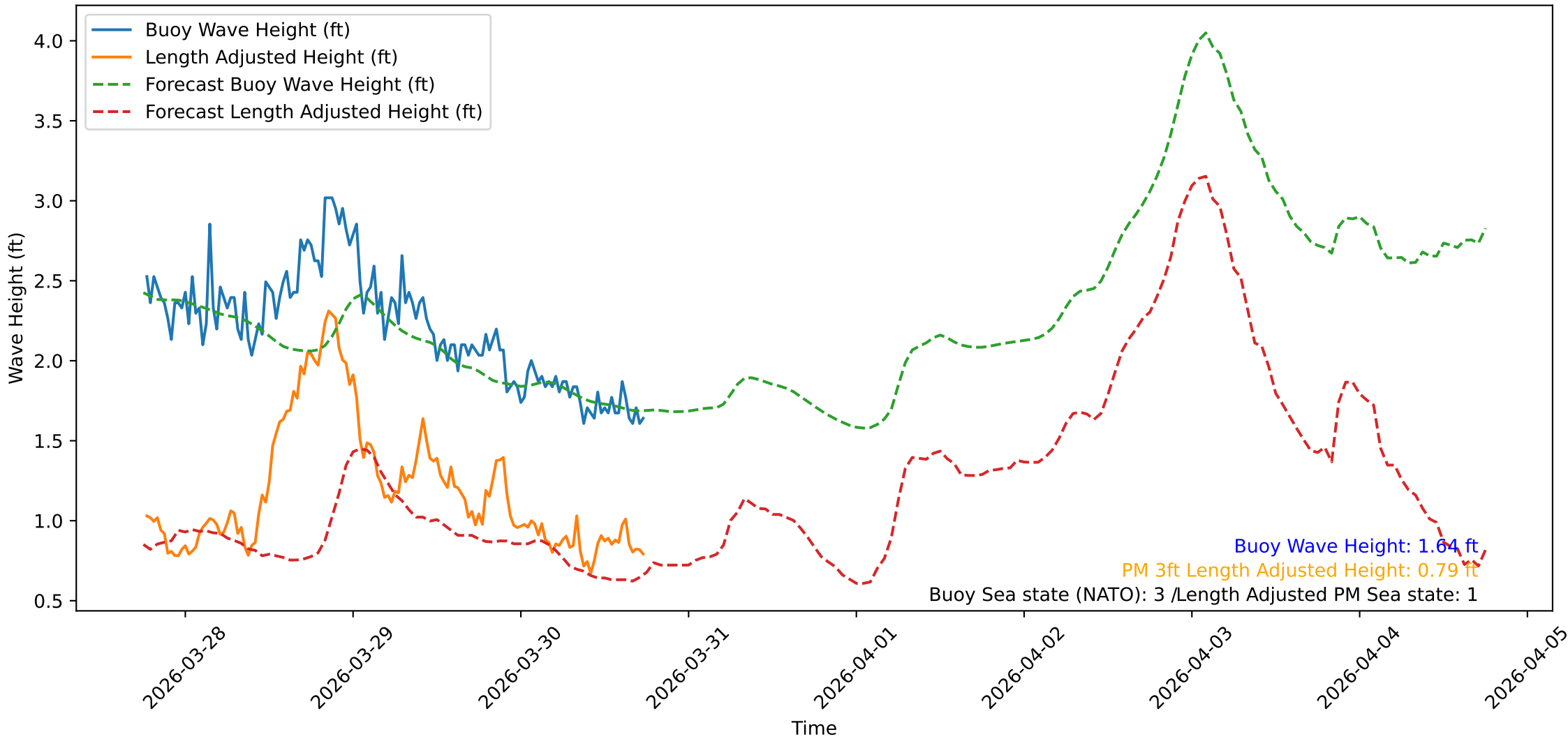
Wave Heights over Time for Red Beach at 2026-03-30 18:20:47
