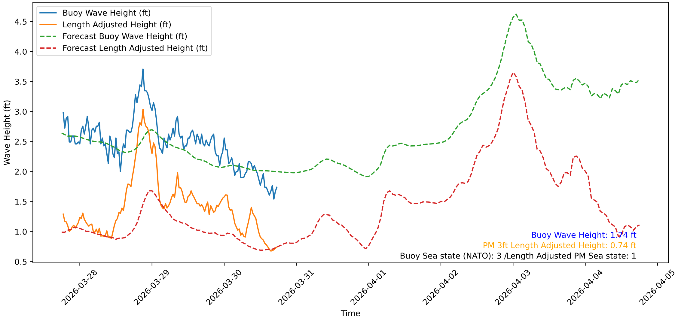
Wave Heights over Time for Green Beach at 2026-03-30 18:21:10
