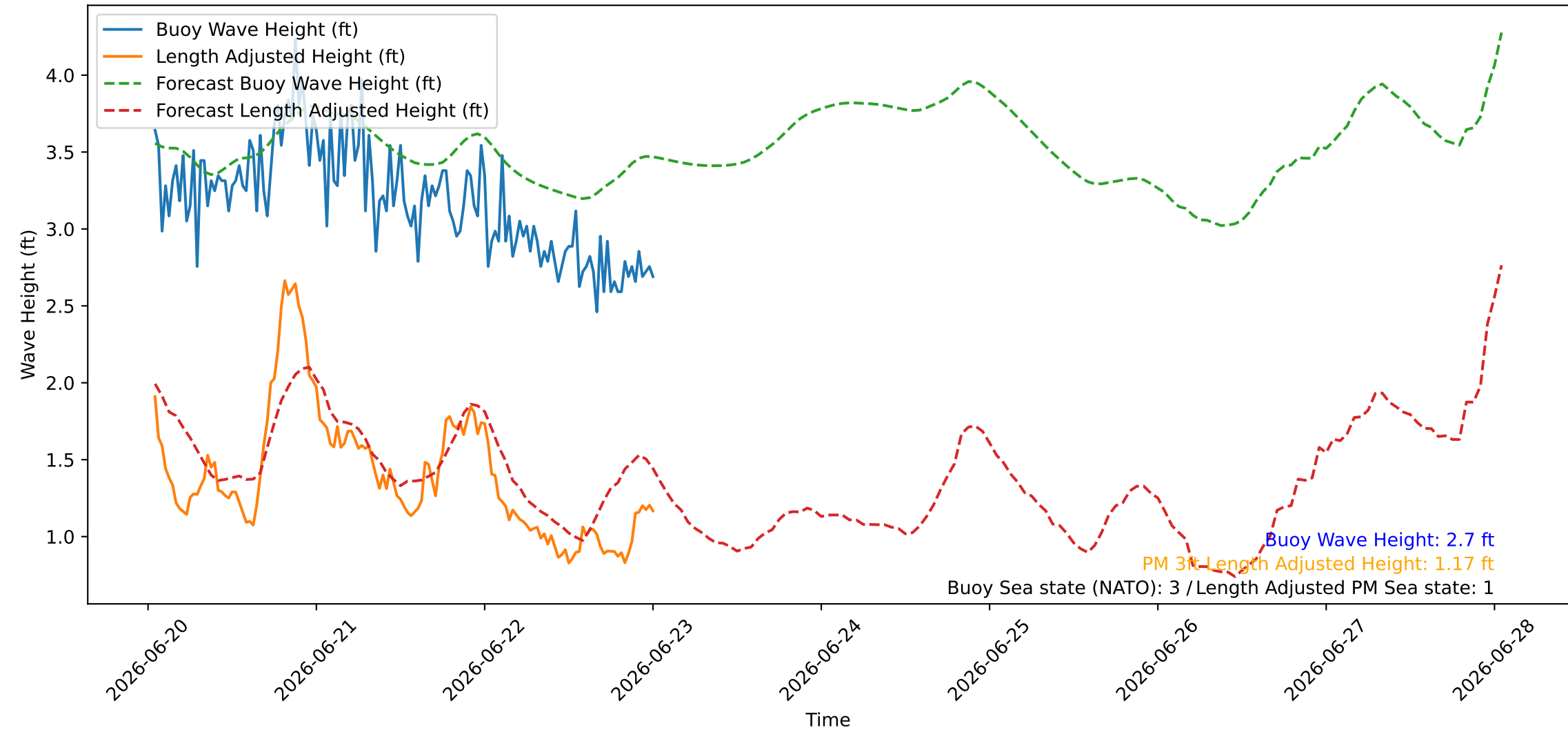
Wave Heights over Time for Green Beach at 2026-06-23 01:01:07
