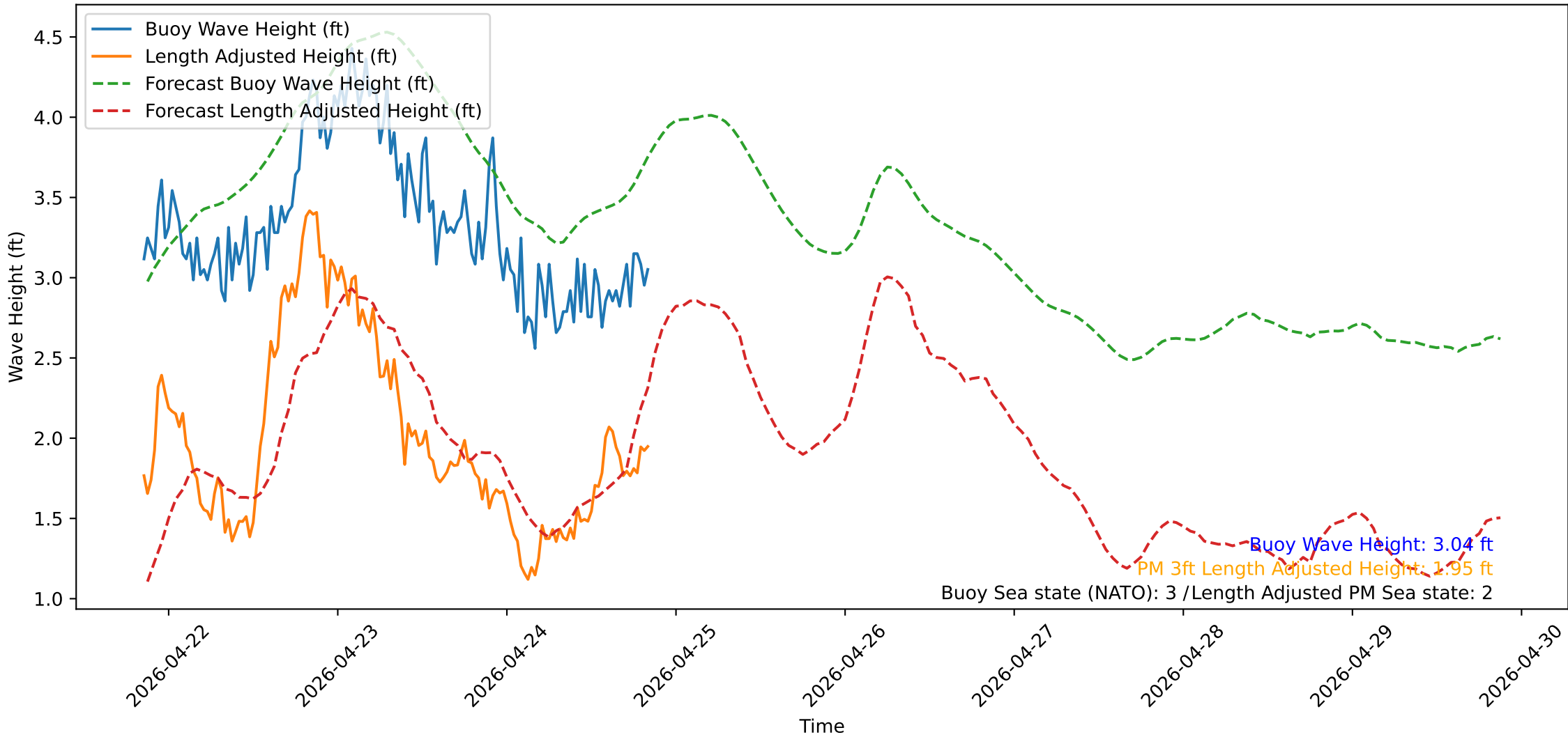
Wave Heights over Time for Oceanside Harbor at 2026-04-24 20:40:31
