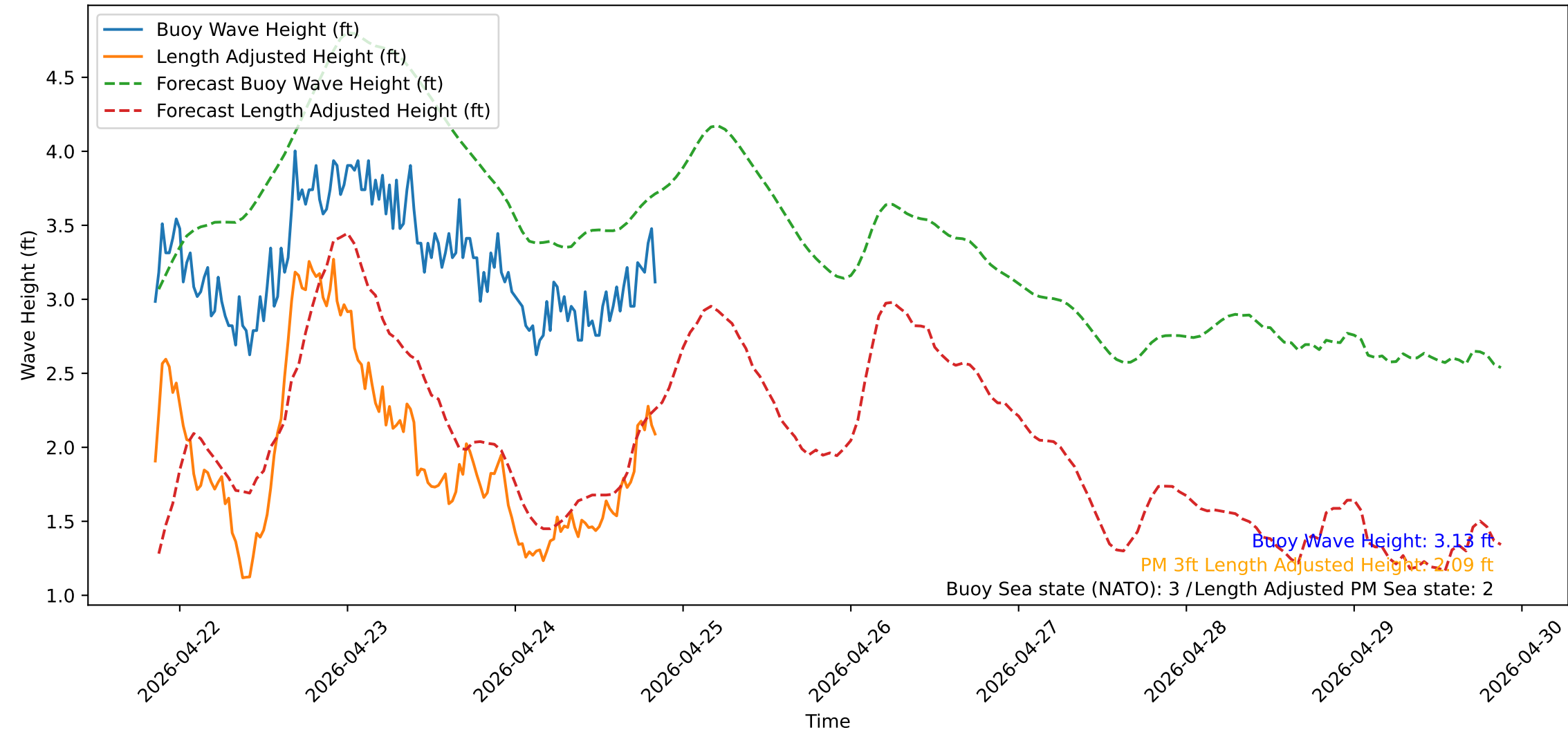
Wave Heights over Time for Green Beach at 2026-04-24 20:41:12
