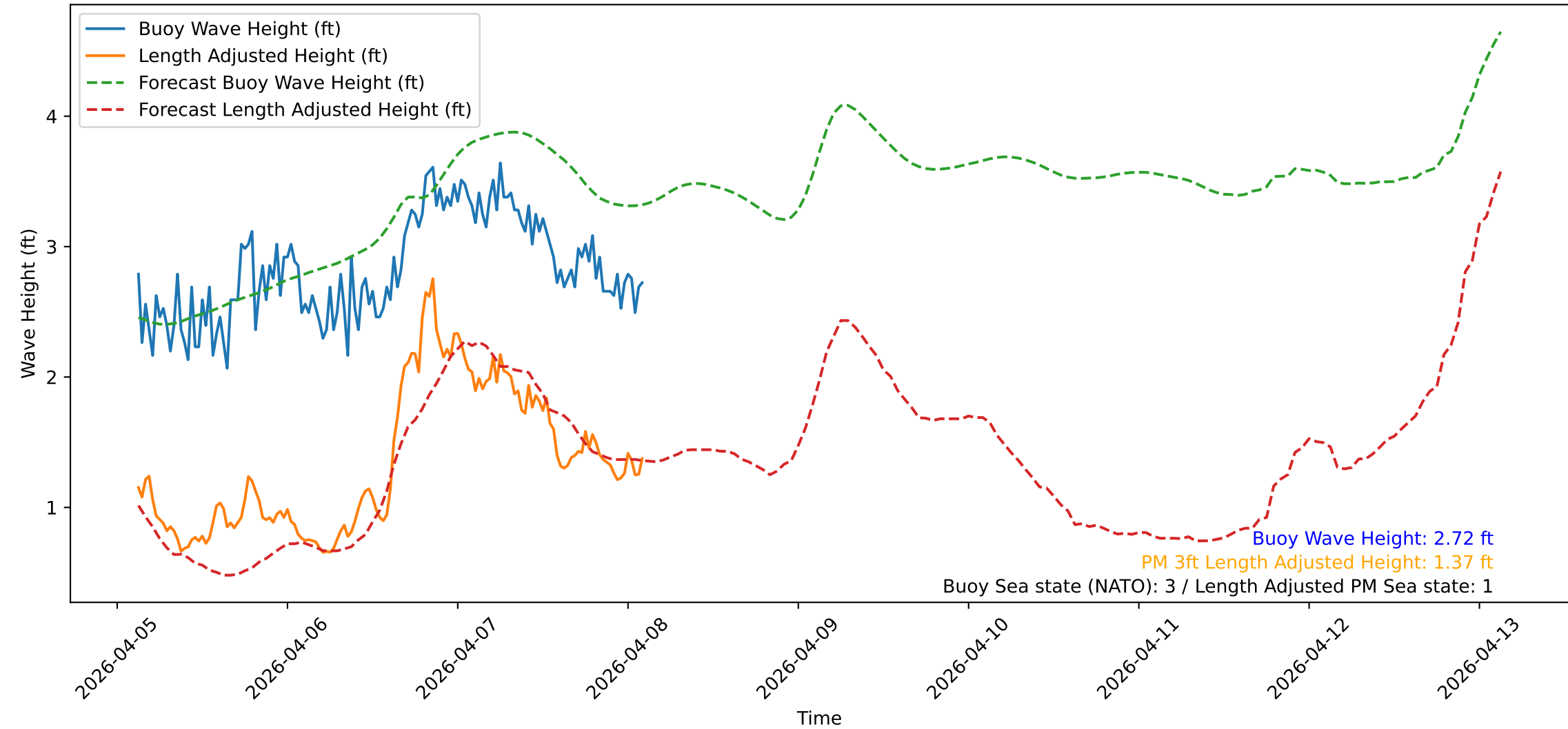
Wave Heights over Time for Oceanside Harbor at 2026-04-08 03:10:31
