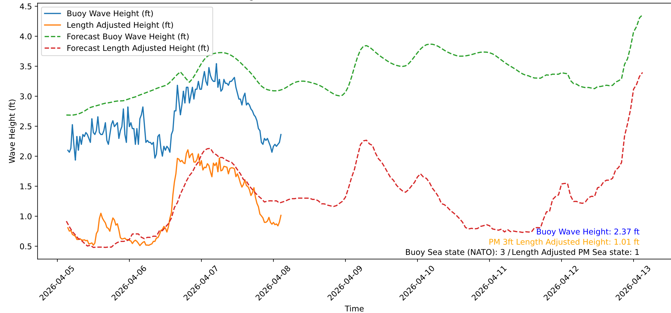
Wave Heights over Time for Red Beach at 2026-04-08 03:10:48
