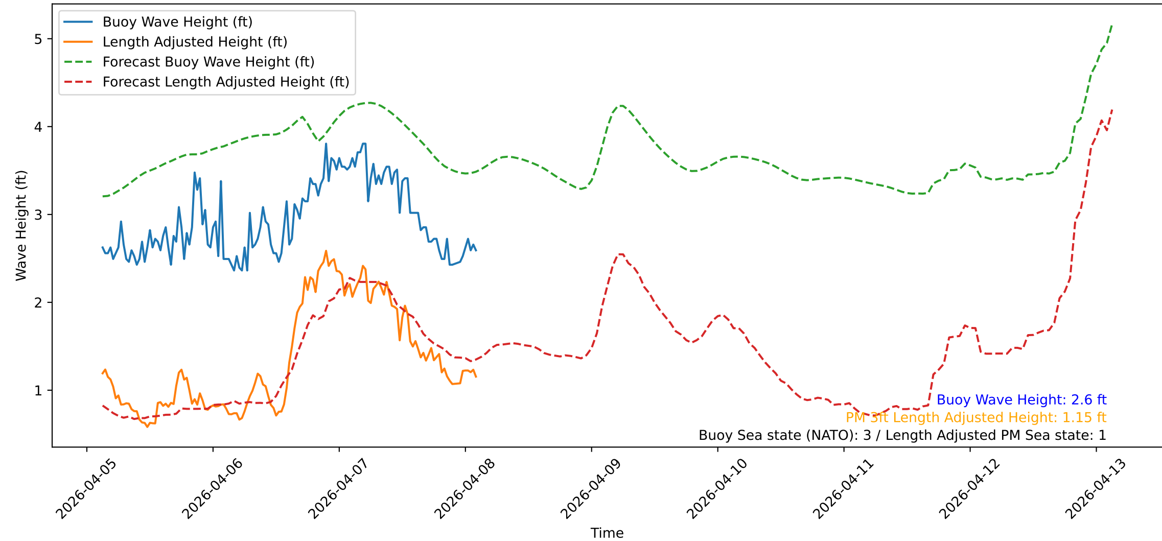
Wave Heights over Time for Green Beach at 2026-04-08 03:11:10
