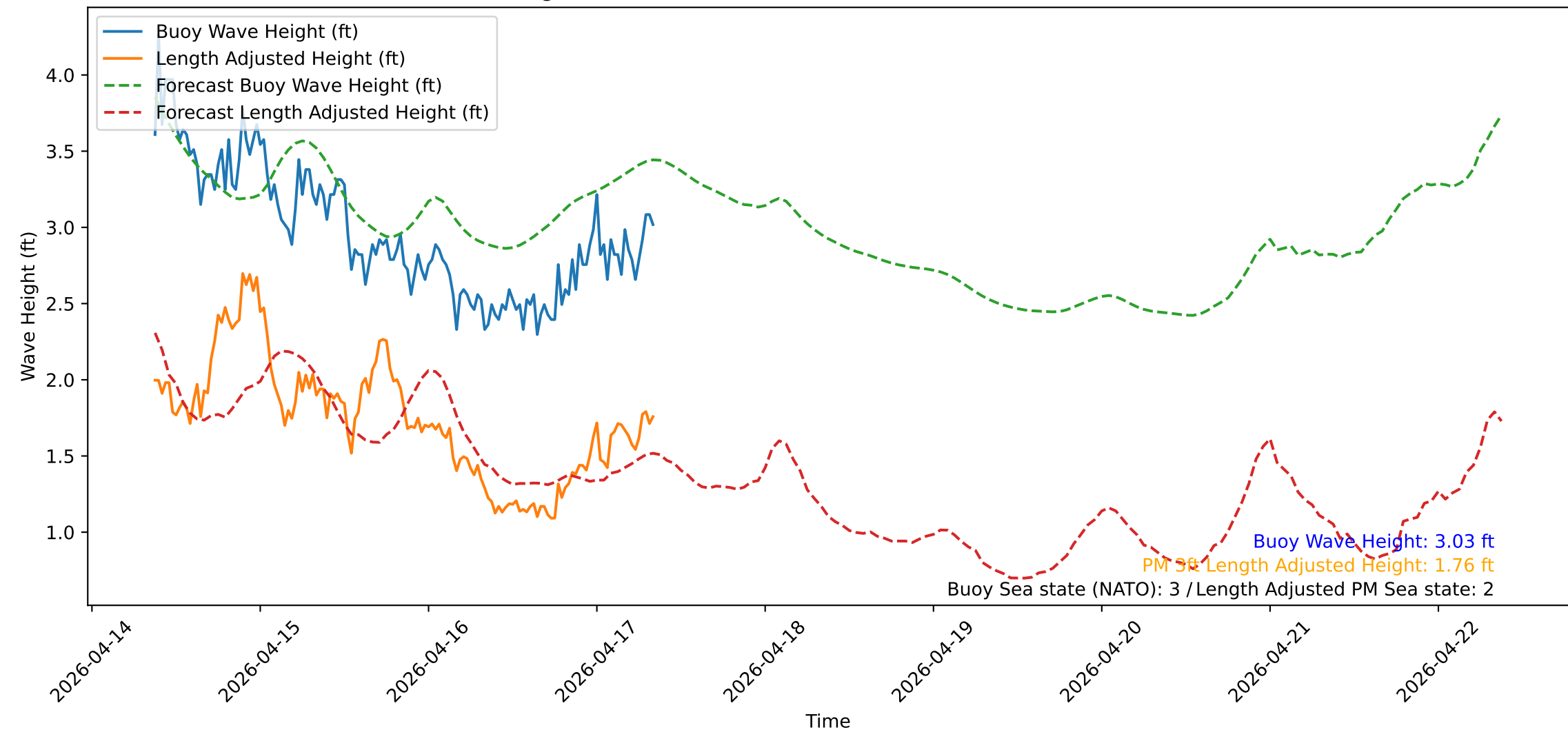
Wave Heights over Time for Oceanside Harbor at 2026-04-17 08:50:32
