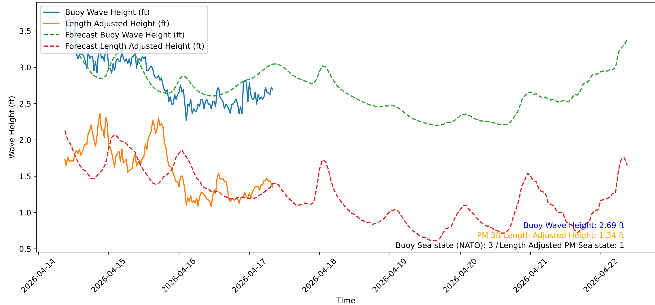
Wave Heights over Time for Red Beach at 2026-04-17 08:50:53
