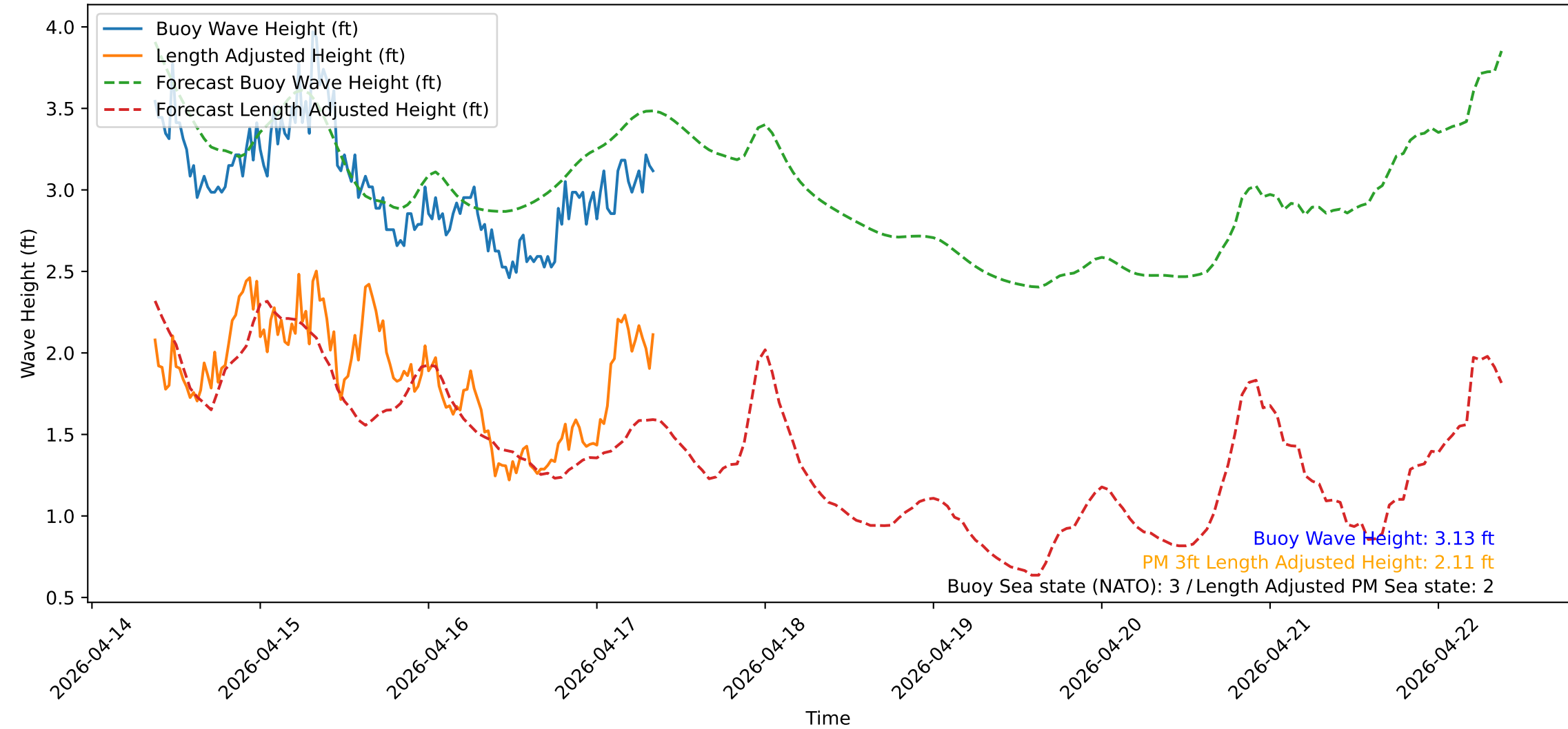
Wave Heights over Time for Green Beach at 2026-04-17 08:51:15
