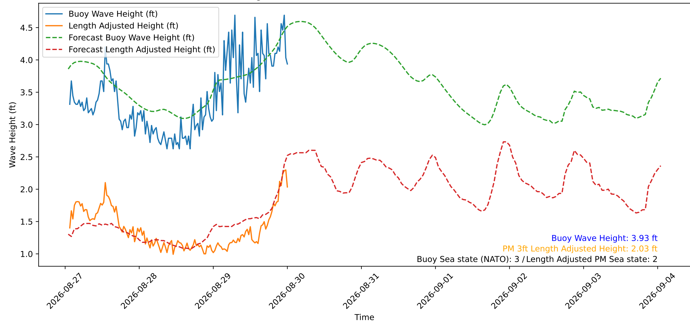
Wave Heights over Time for Red Beach at 2026-08-30 01:00:49
