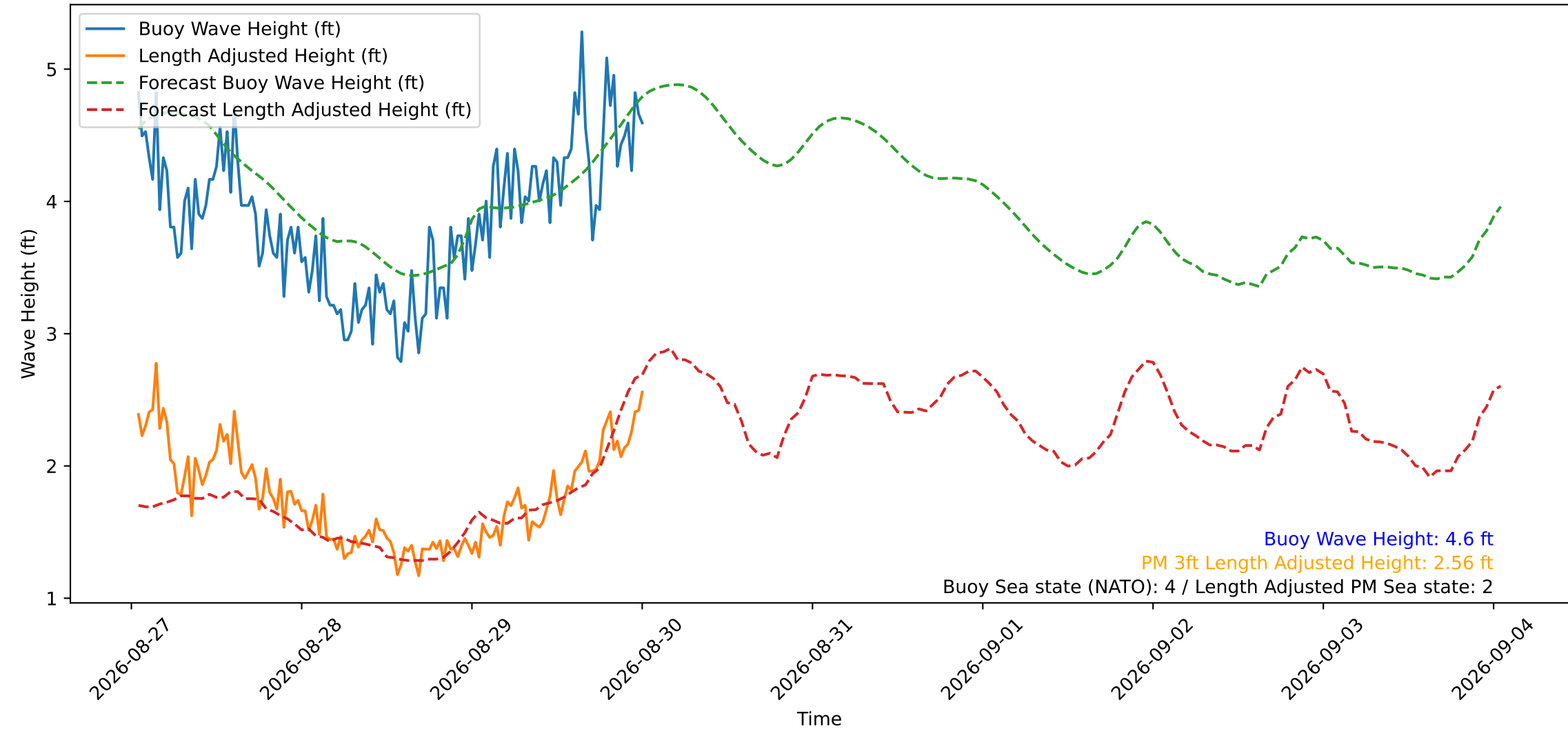
Wave Heights over Time for Oceanside Harbor at 2026-08-30 01:00:29
