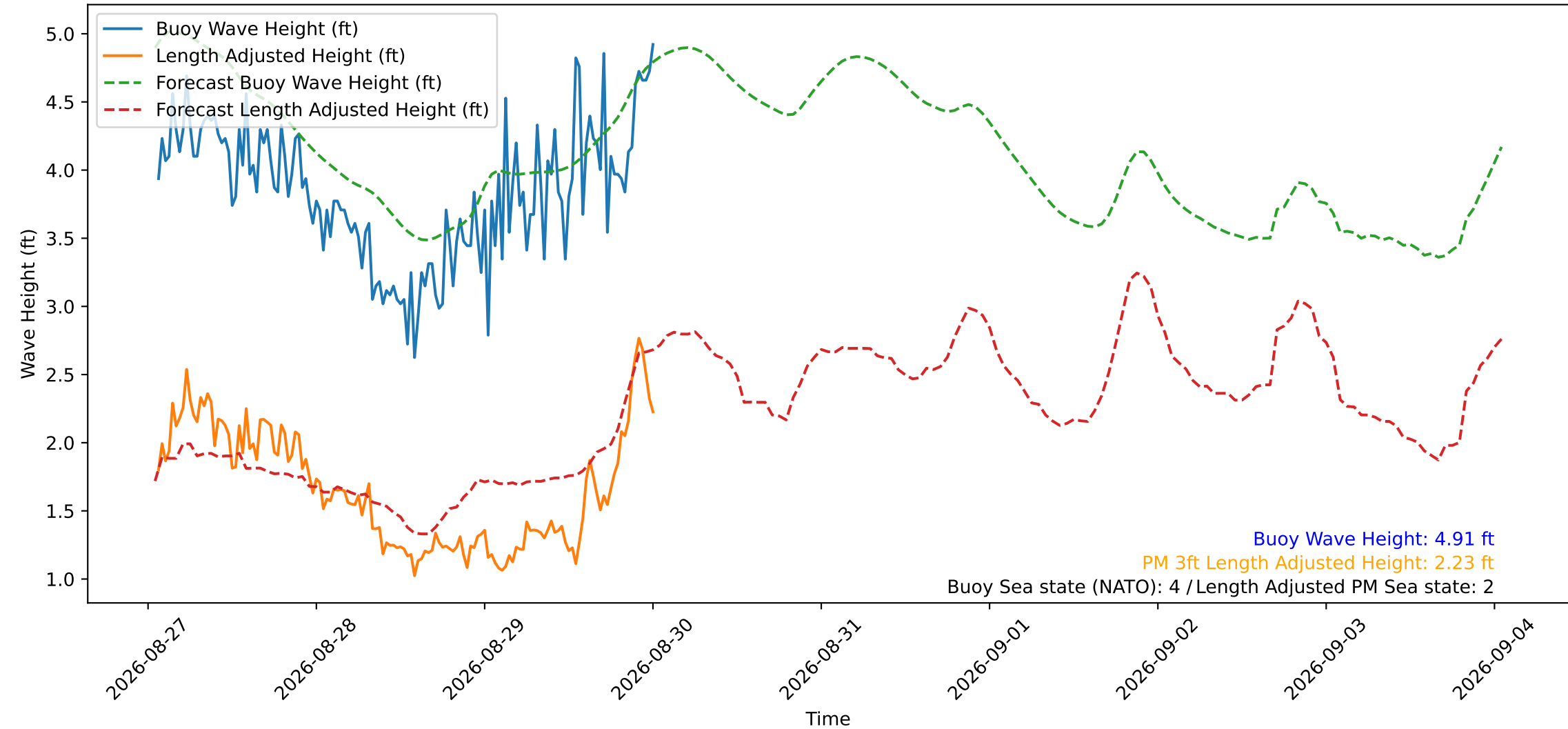
Wave Heights over Time for Green Beach at 2026-08-30 01:01:11
