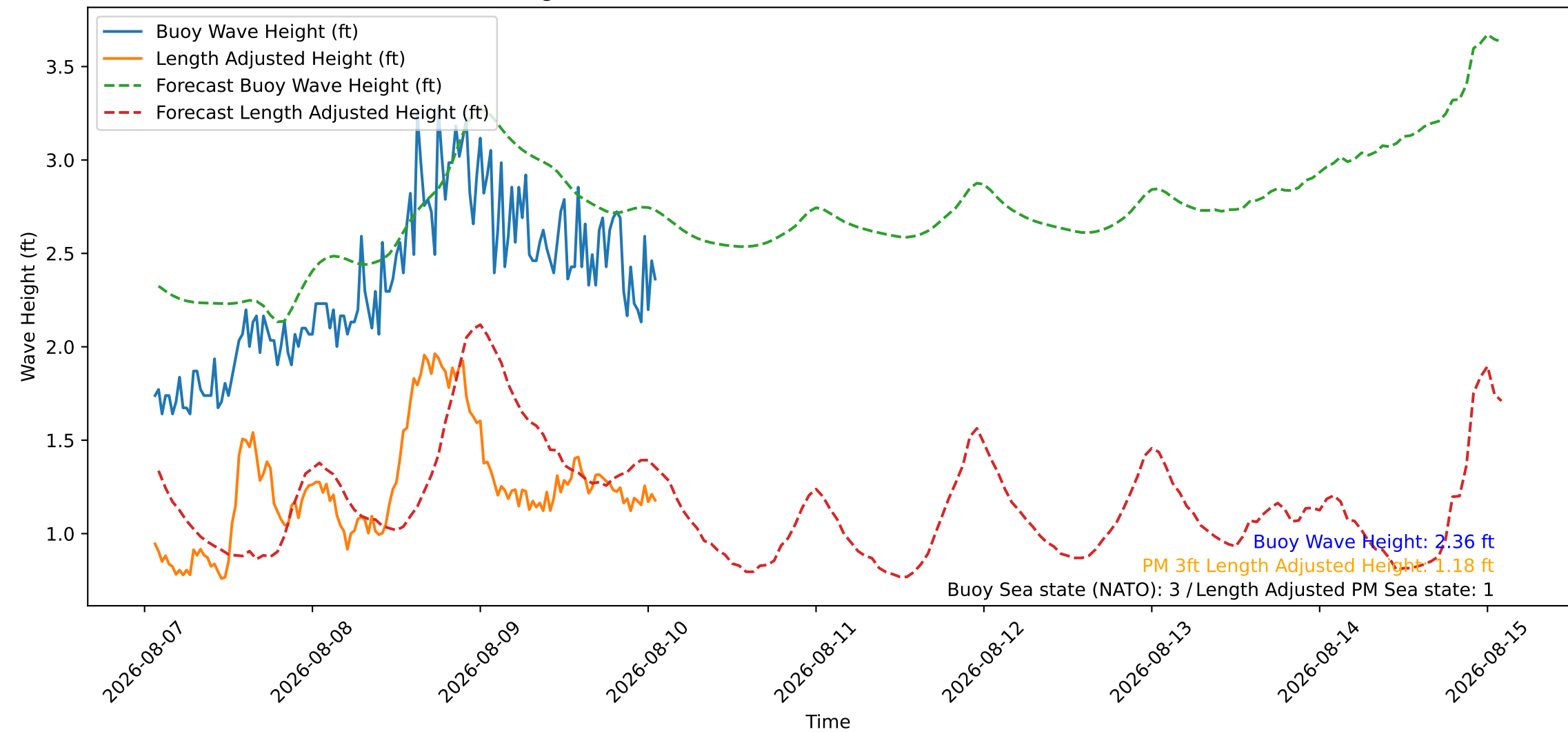
Wave Heights over Time for Oceanside Harbor at 2026-08-10 01:40:27
