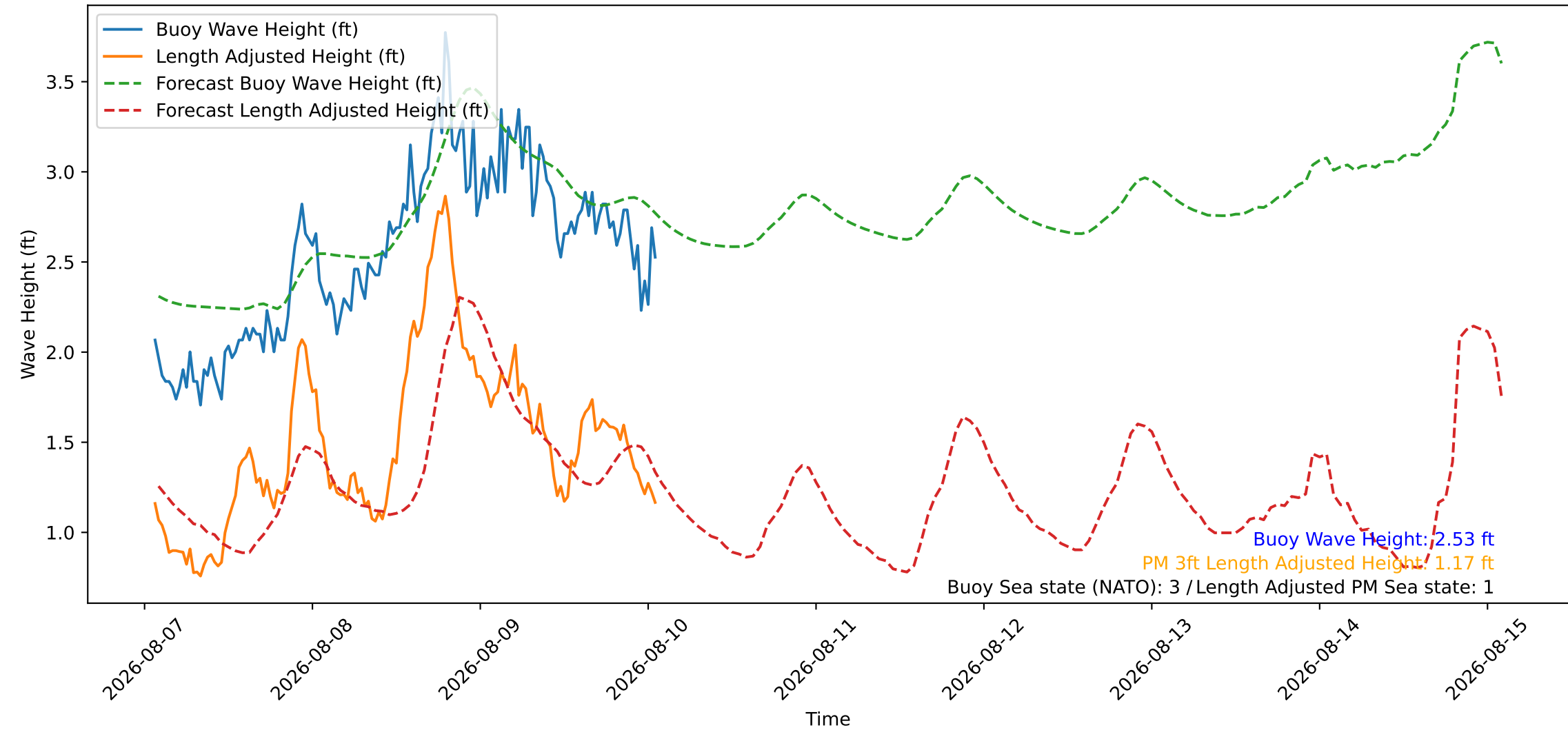
Wave Heights over Time for Green Beach at 2026-08-10 01:41:10
