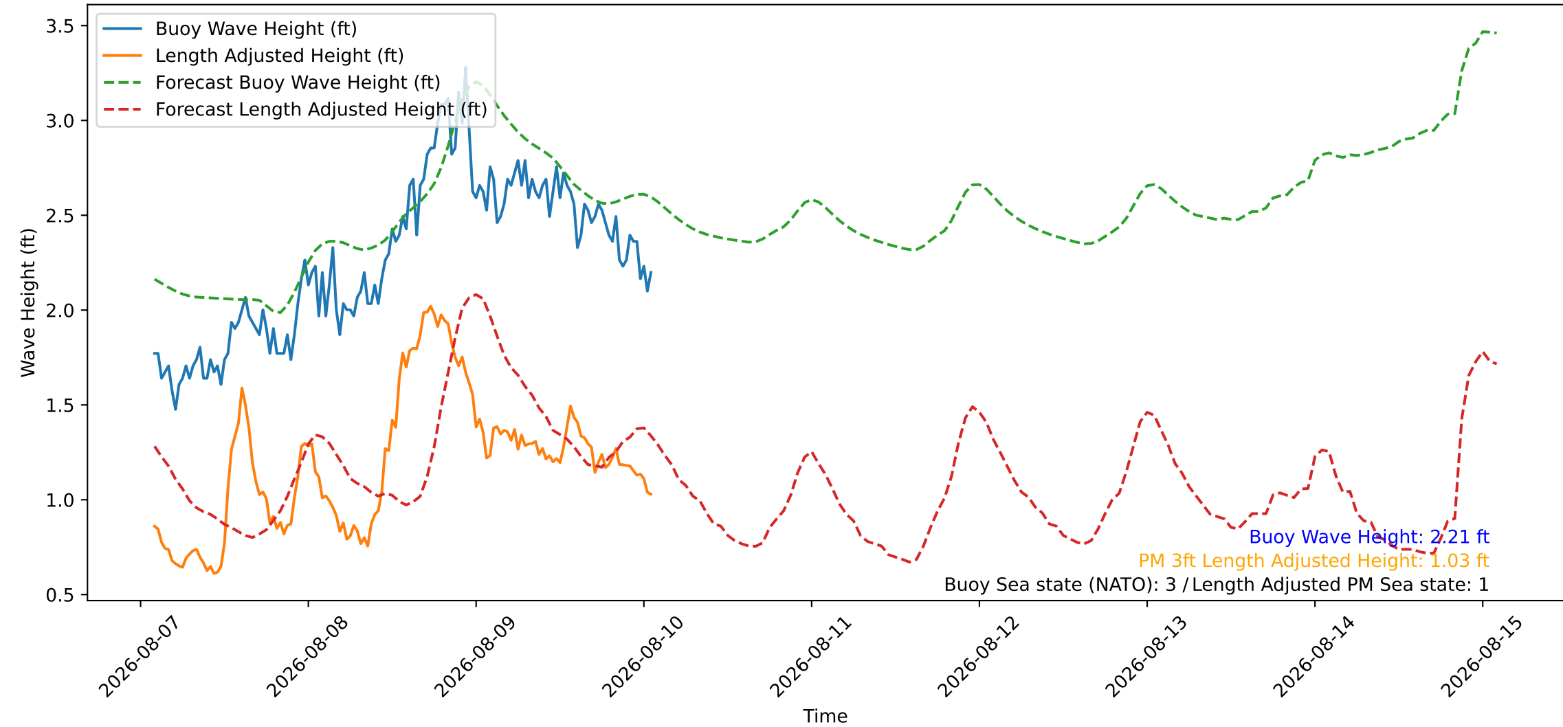
Wave Heights over Time for Red Beach at 2026-08-10 01:40:47
