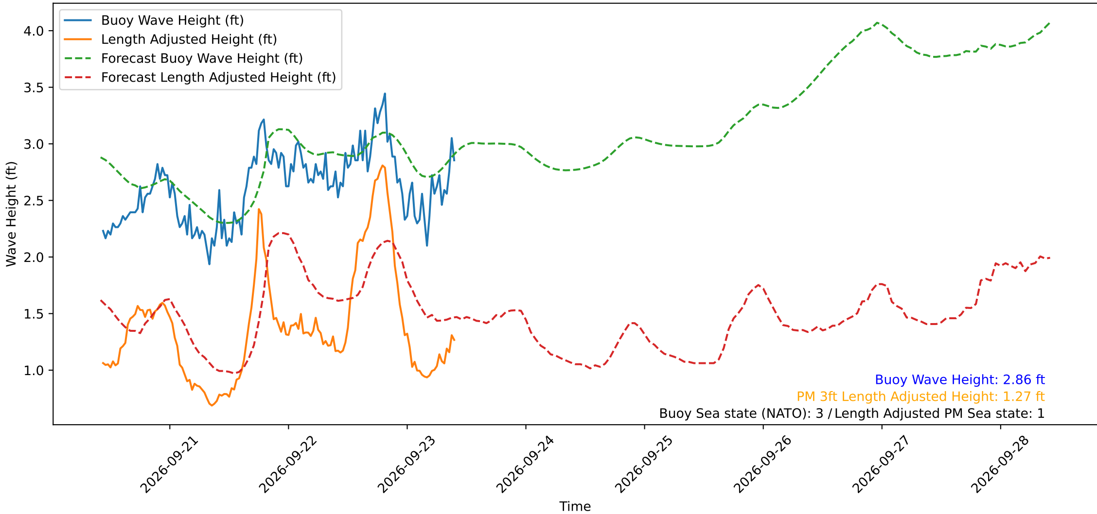
Wave Heights over Time for Green Beach at 2026-09-23 10:21:15
