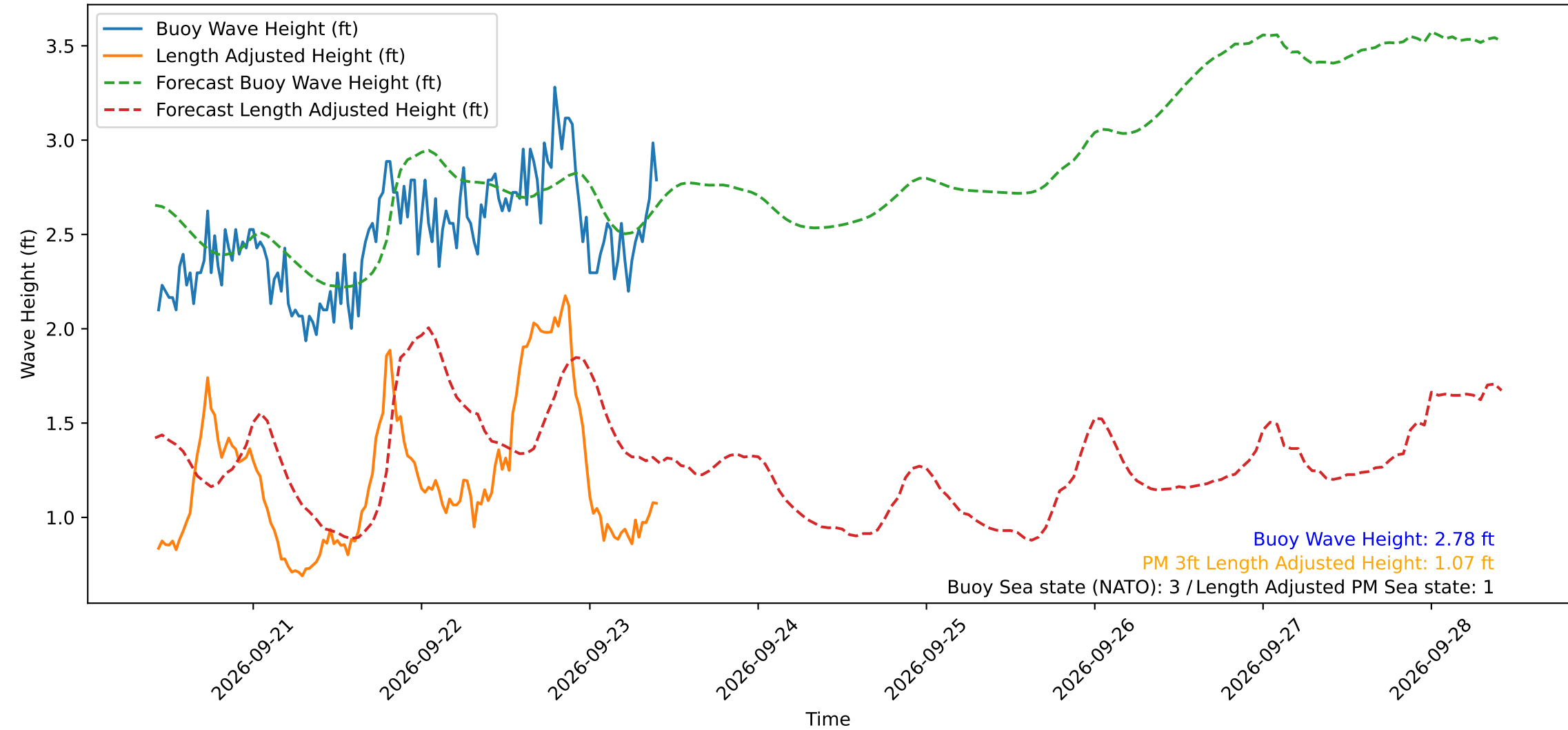
Wave Heights over Time for Red Beach at 2026-09-23 10:20:52
