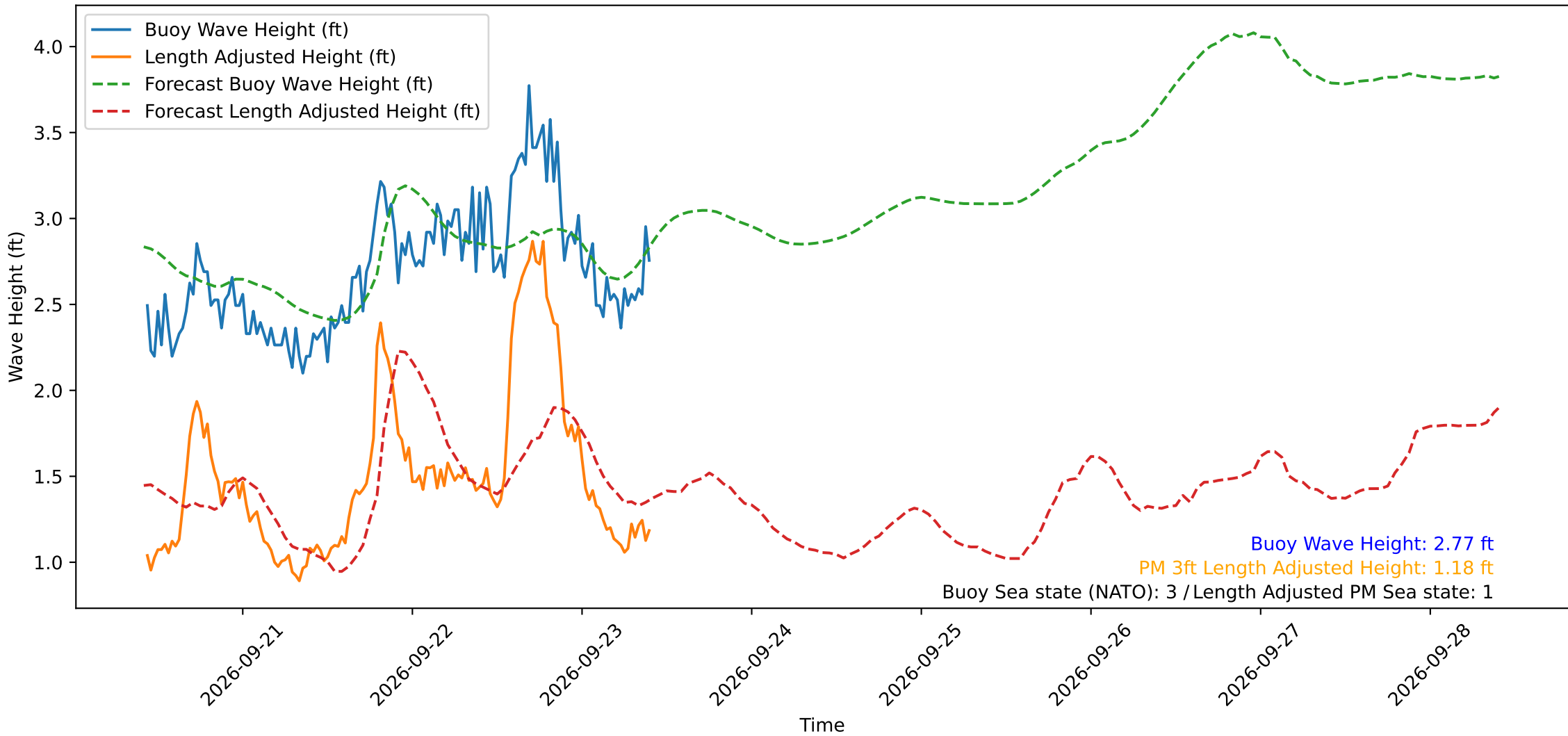
Wave Heights over Time for Oceanside Harbor at 2026-09-23 10:20:30
