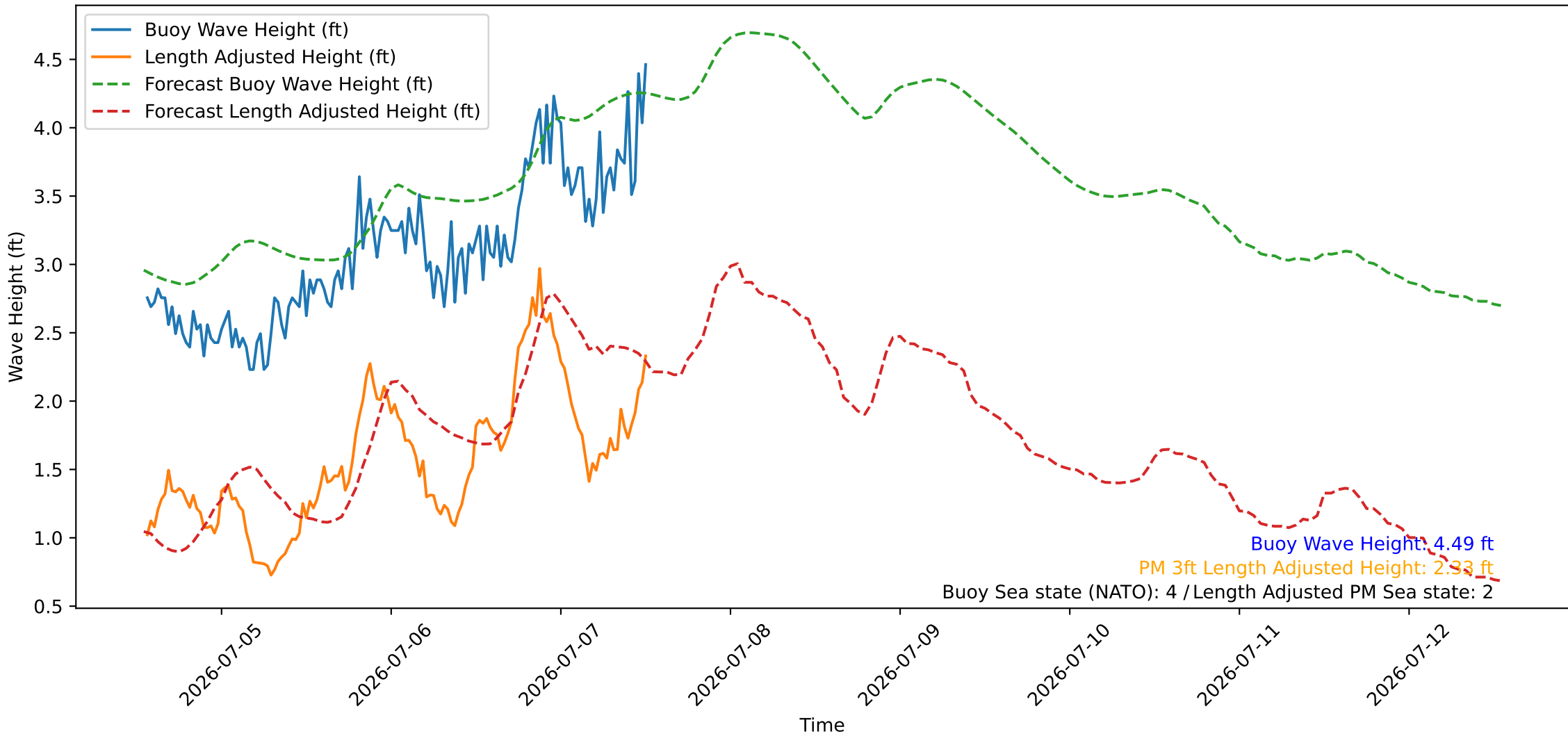
Wave Heights over Time for Red Beach at 2026-07-07 13:10:45
