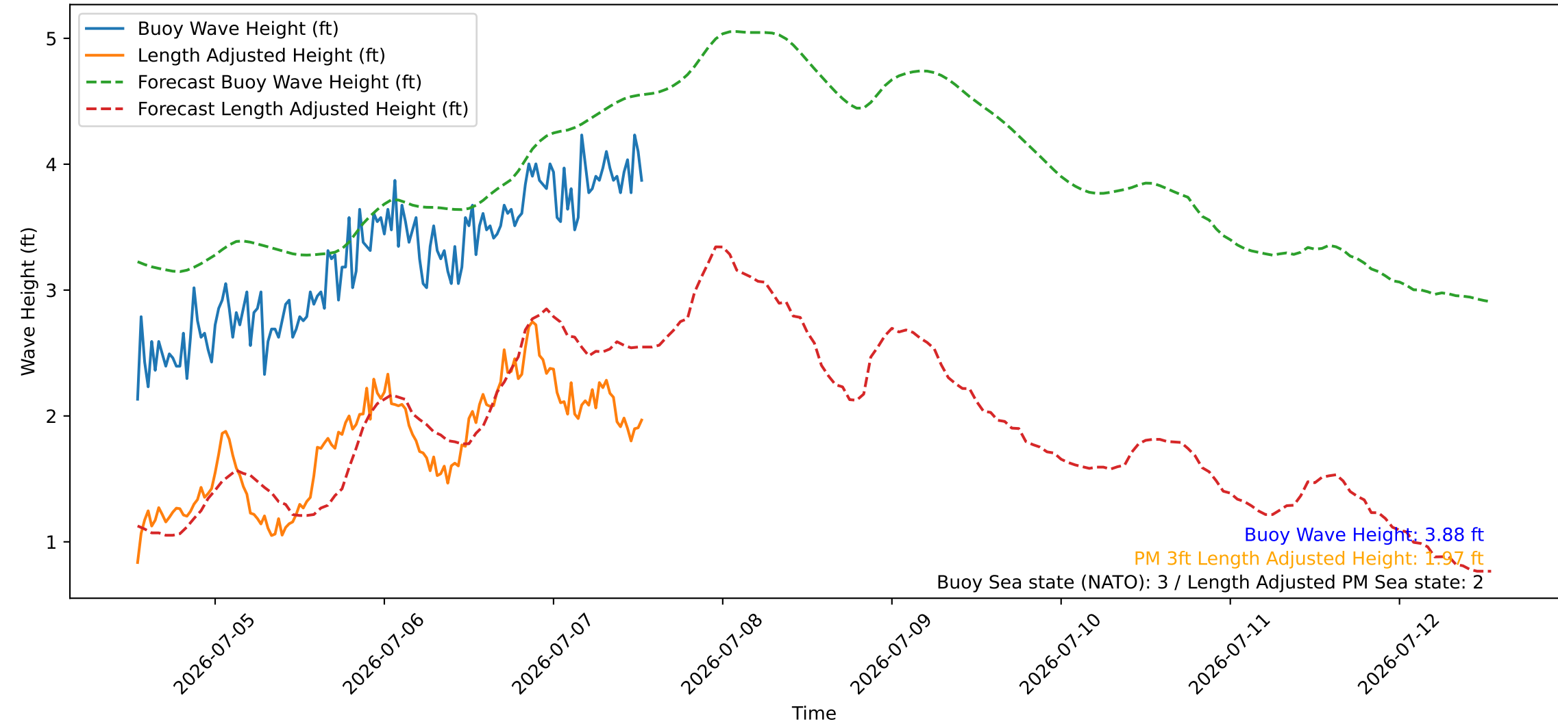
Wave Heights over Time for Oceanside Harbor at 2026-07-07 13:10:26
