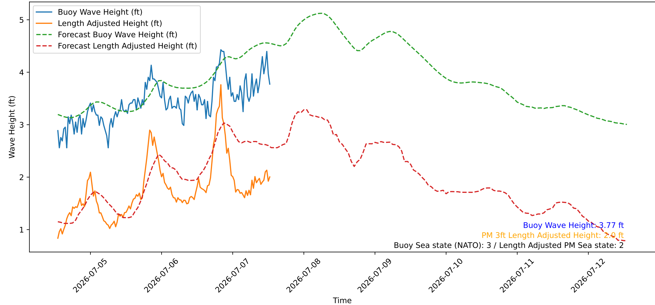
Wave Heights over Time for Green Beach at 2026-07-07 13:11:08
