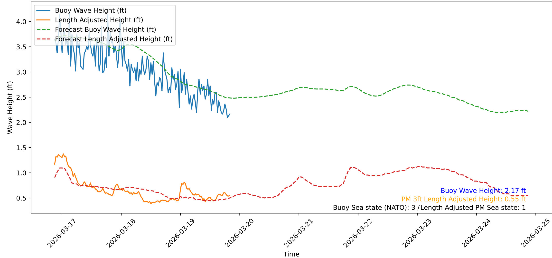
Wave Heights over Time for Green Beach at 2026-03-19 20:51:13
