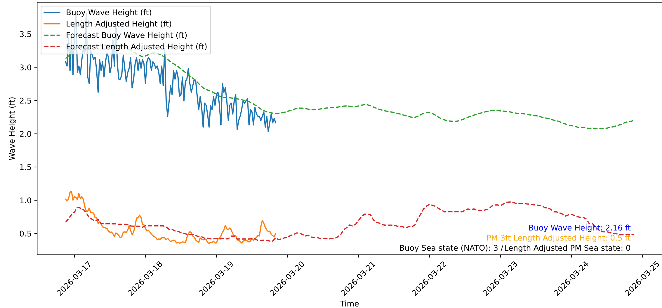
Wave Heights over Time for Red Beach at 2026-03-19 20:50:50
