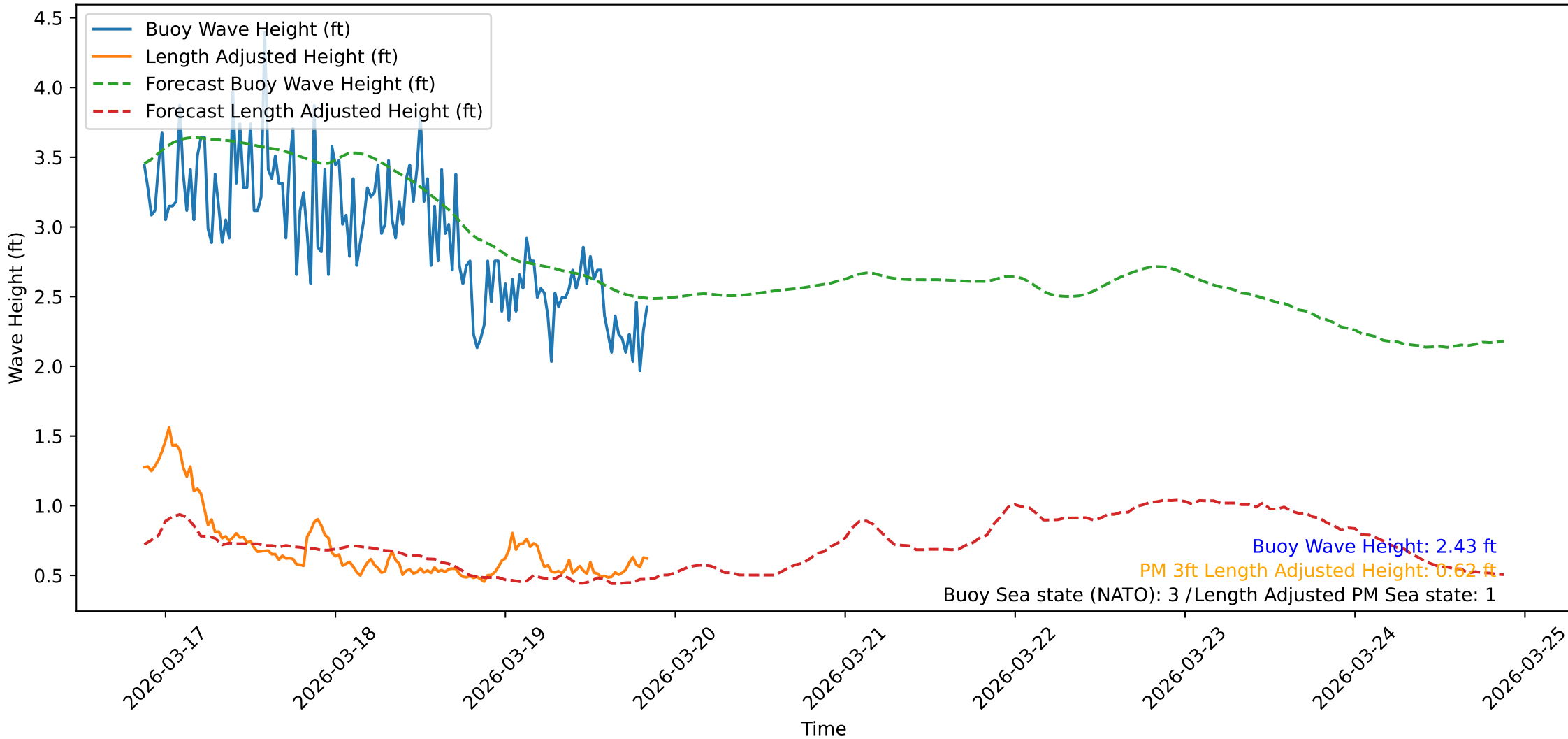
Wave Heights over Time for Oceanside Harbor at 2026-03-19 20:50:34
