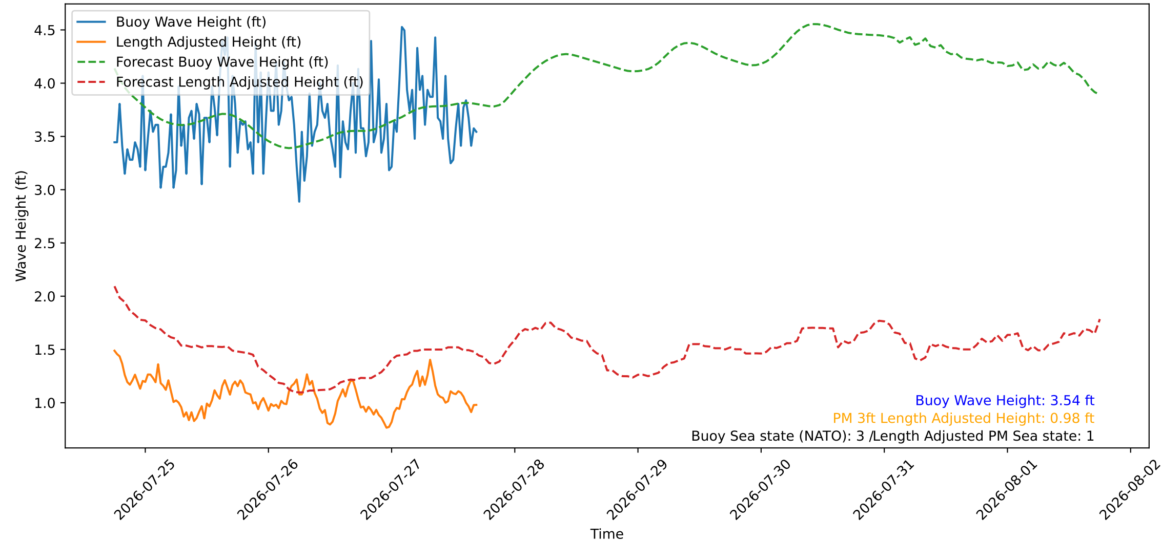
Wave Heights over Time for Red Beach at 2026-07-27 17:30:46
