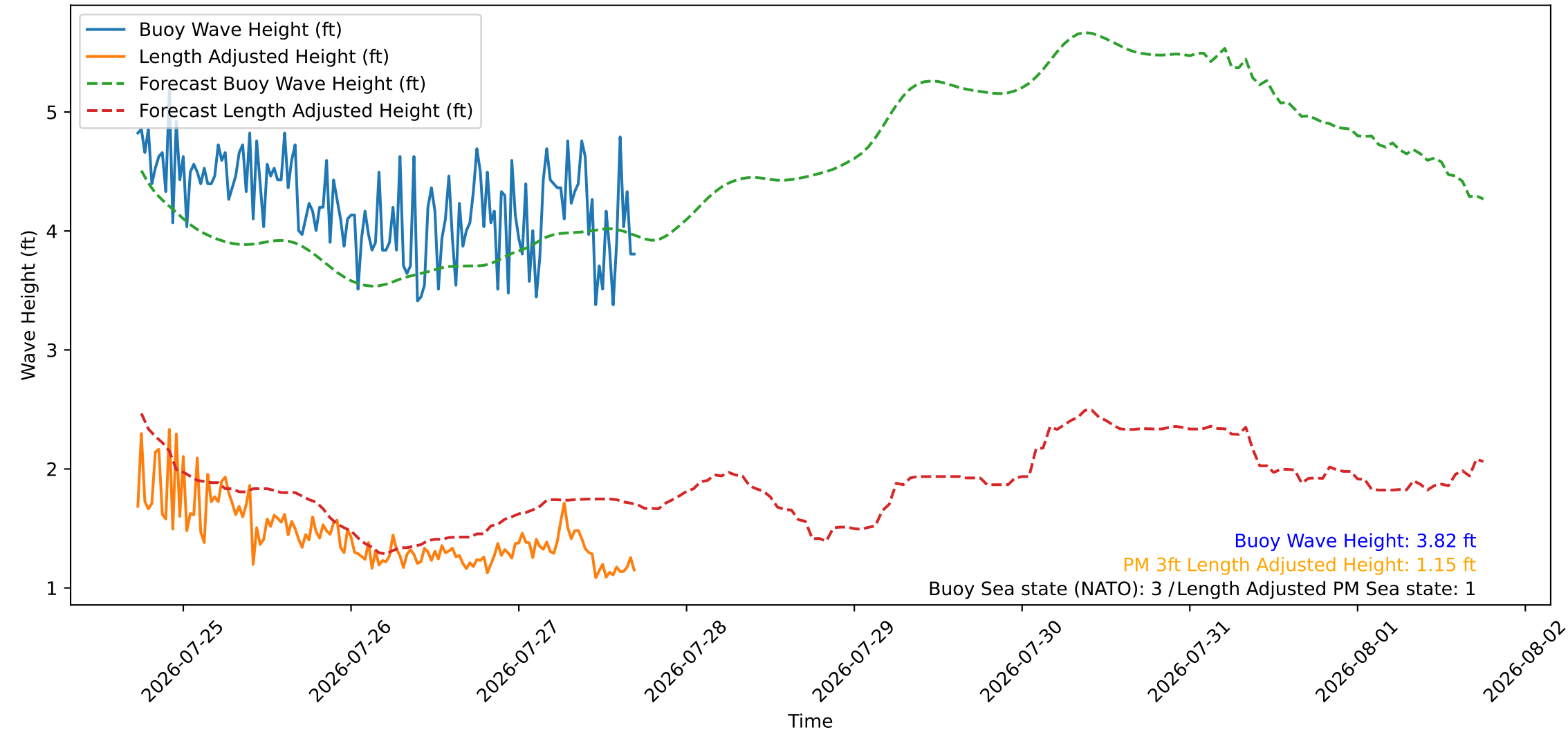
Wave Heights over Time for Green Beach at 2026-07-27 17:31:08
