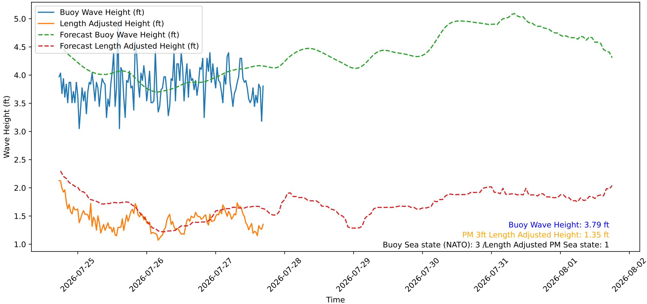
Wave Heights over Time for Oceanside Harbor at 2026-07-27 17:30:26
