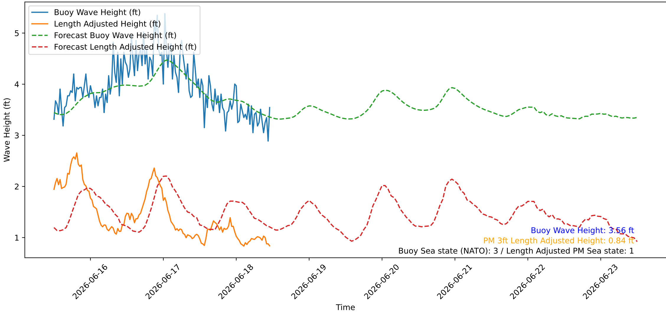
Wave Heights over Time for Red Beach at 2026-06-18 11:40:47
