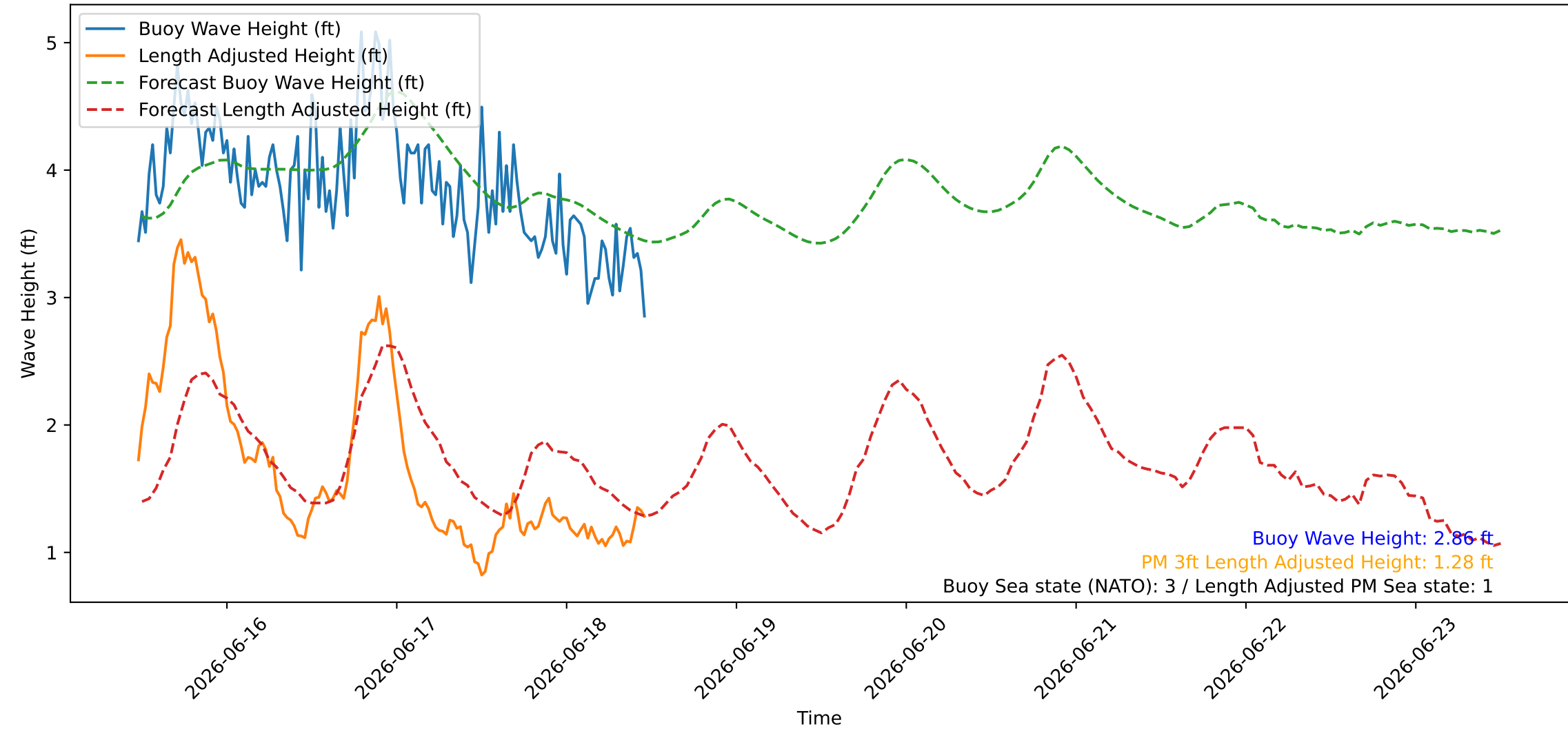
Wave Heights over Time for Green Beach at 2026-06-18 11:41:10
