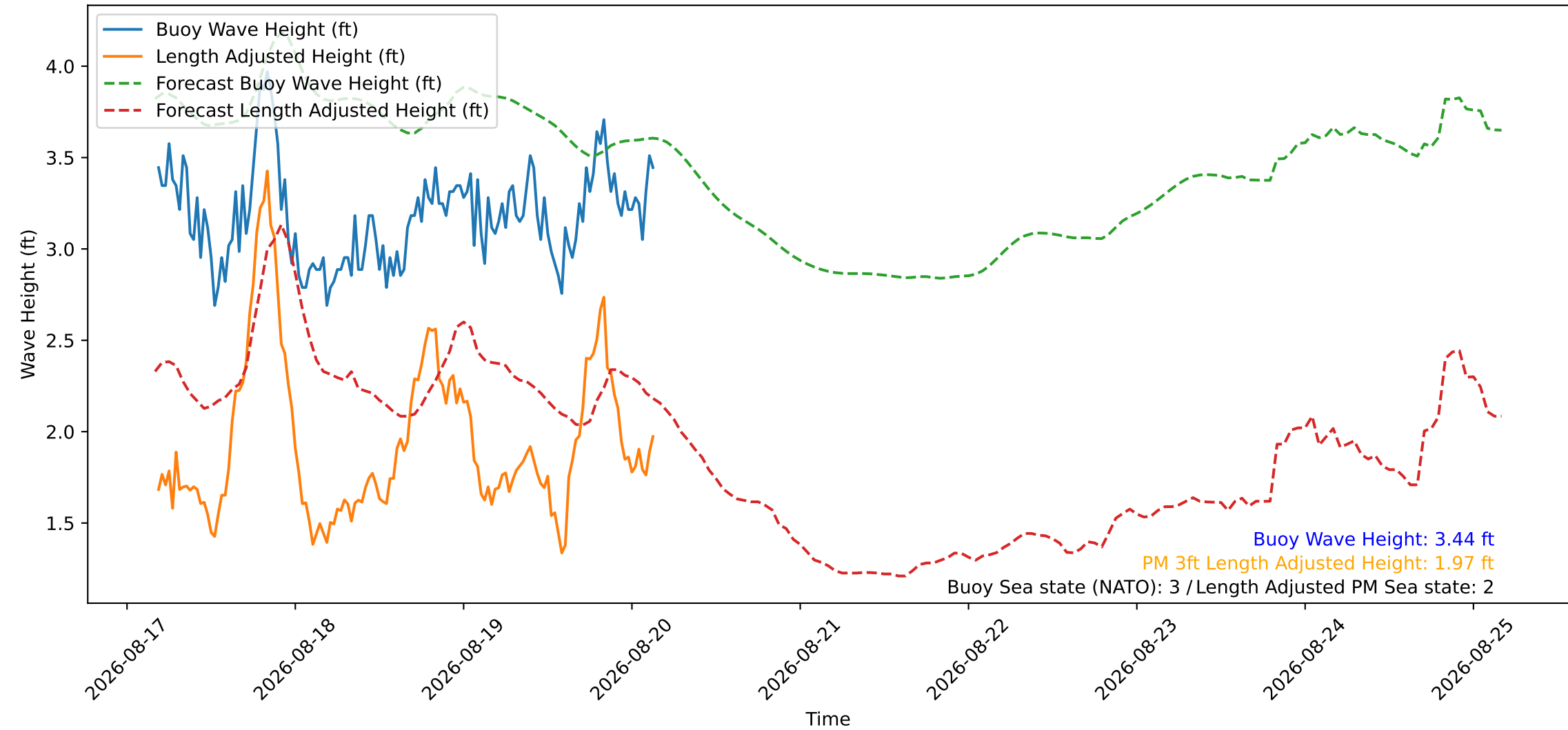
Wave Heights over Time for Green Beach at 2026-08-20 04:01:08
