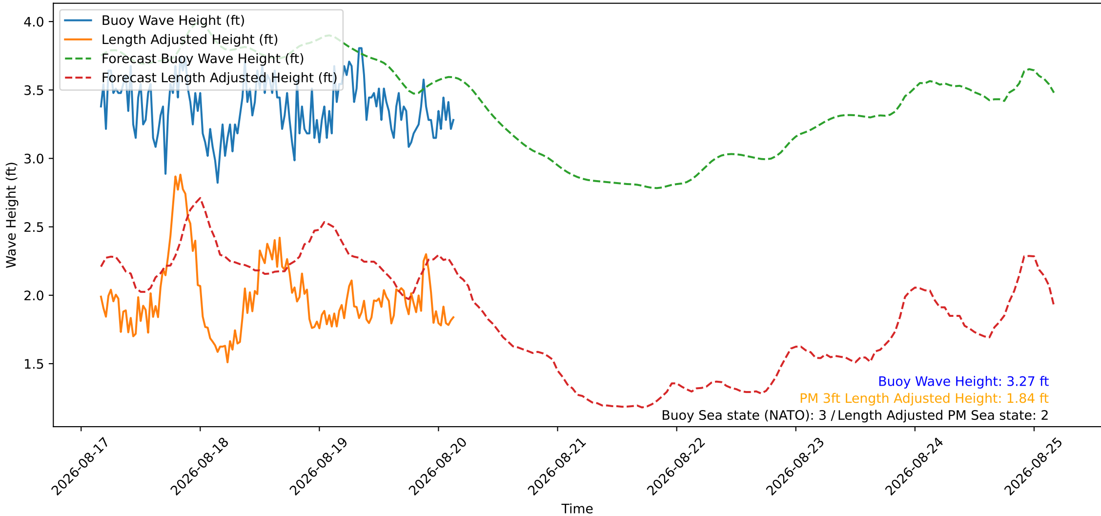
Wave Heights over Time for Oceanside Harbor at 2026-08-20 04:00:26
