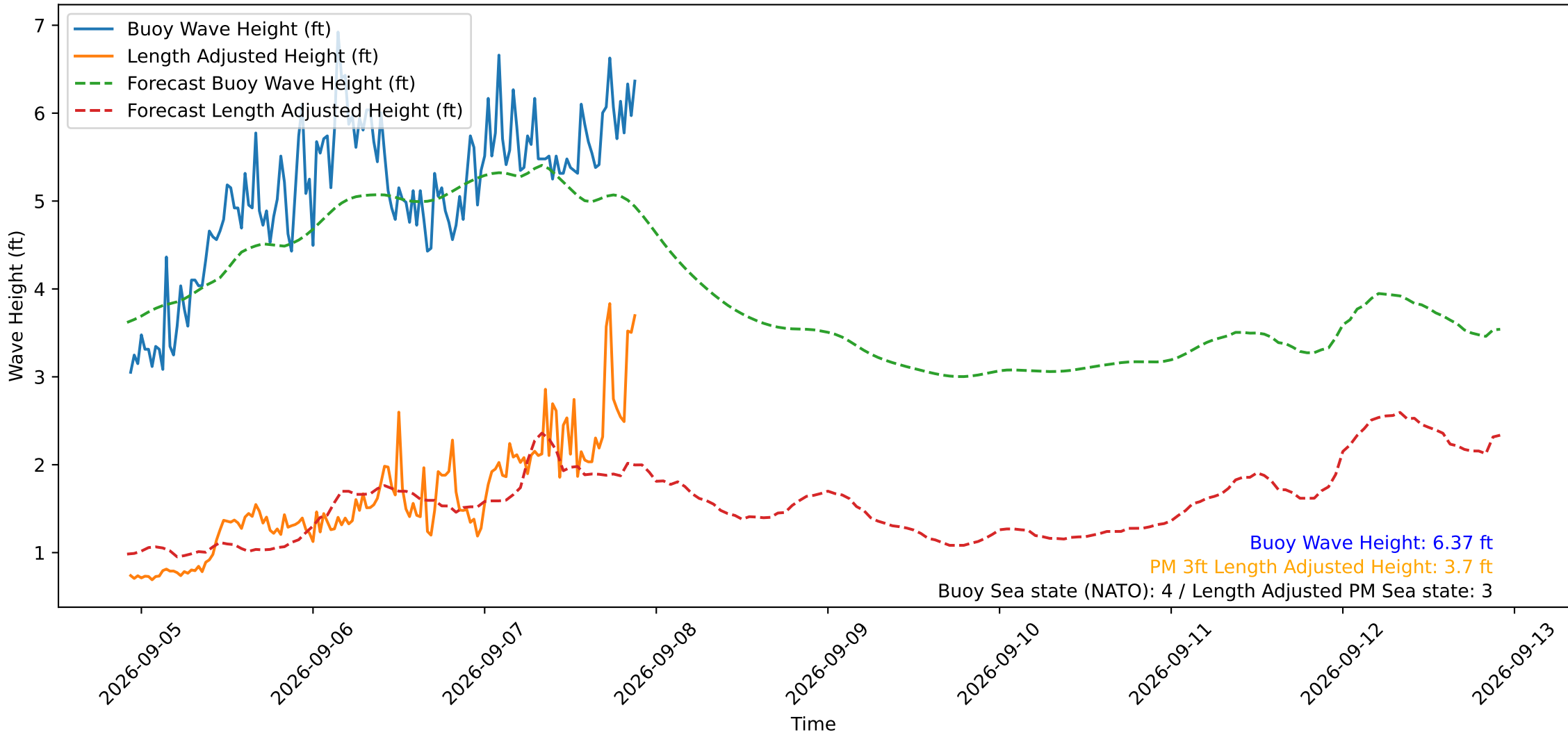
Wave Heights over Time for Red Beach at 2026-09-07 22:00:50
