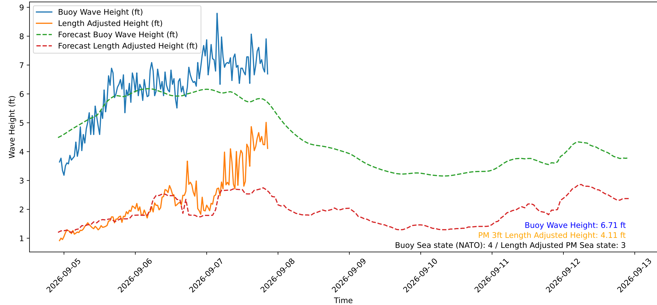
Wave Heights over Time for Green Beach at 2026-09-07 22:01:12
