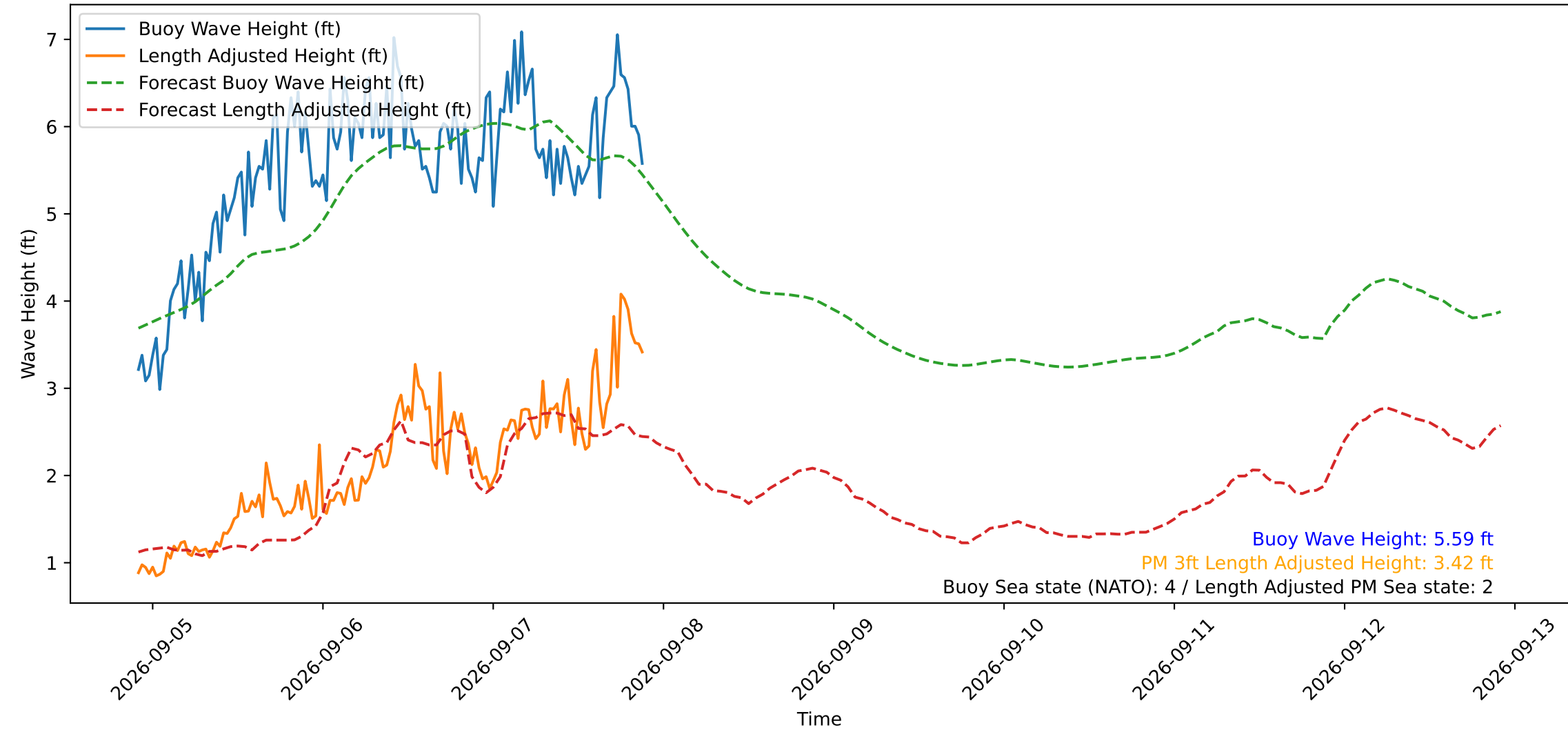
Wave Heights over Time for Oceanside Harbor at 2026-09-07 22:00:30
