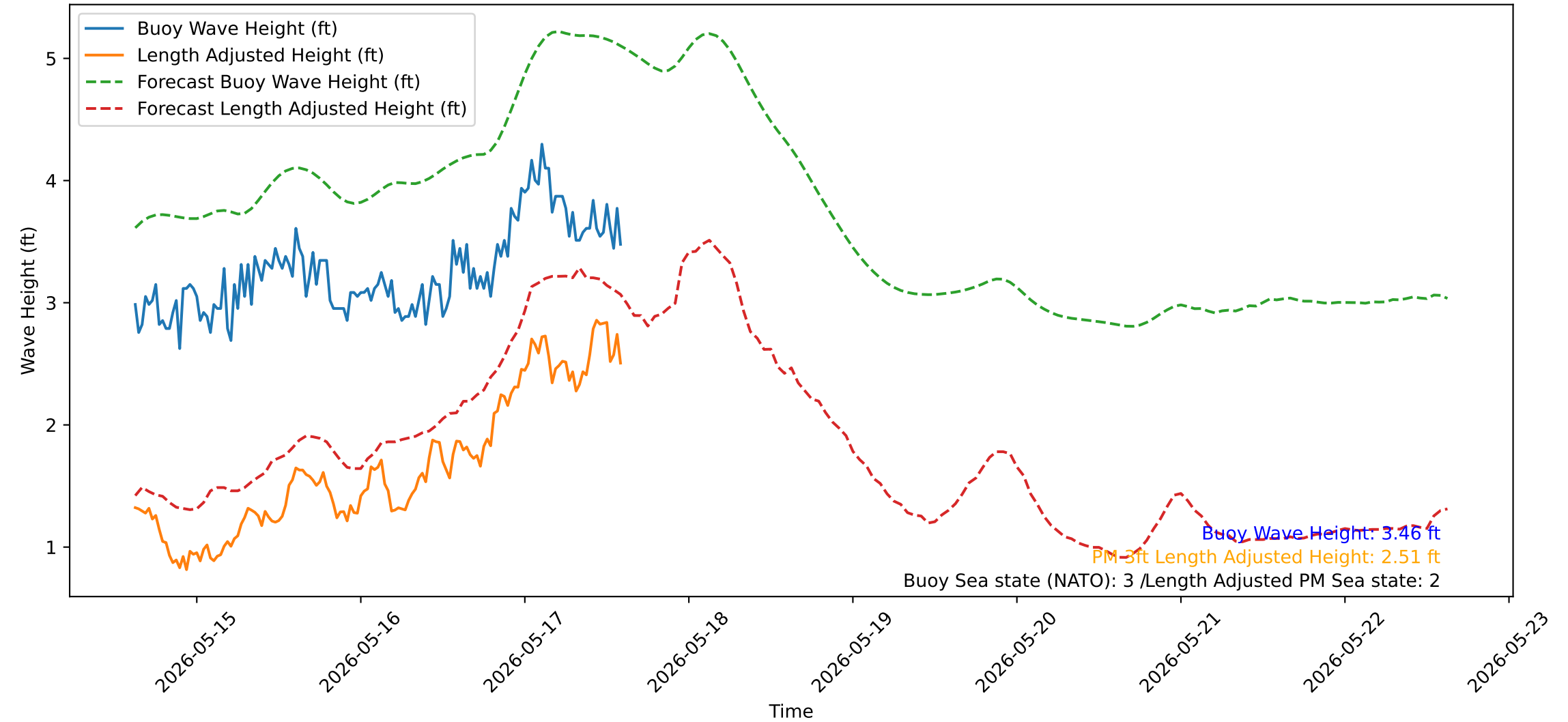
Wave Heights over Time for Oceanside Harbor at 2026-05-17 14:50:32
