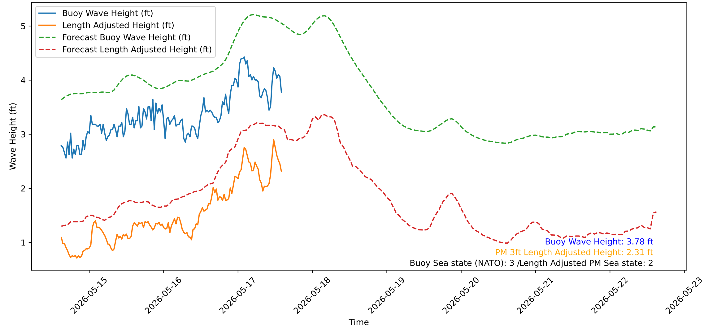
Wave Heights over Time for Green Beach at 2026-05-17 14:51:15
