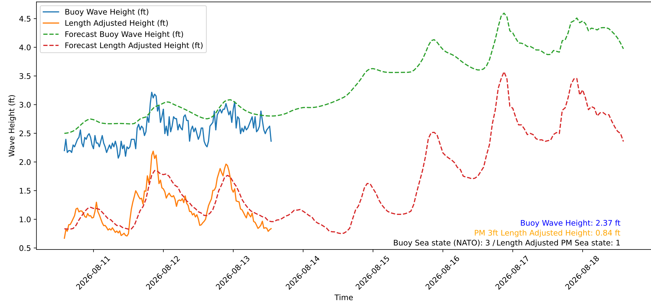
Wave Heights over Time for Green Beach at 2026-08-13 13:51:09
