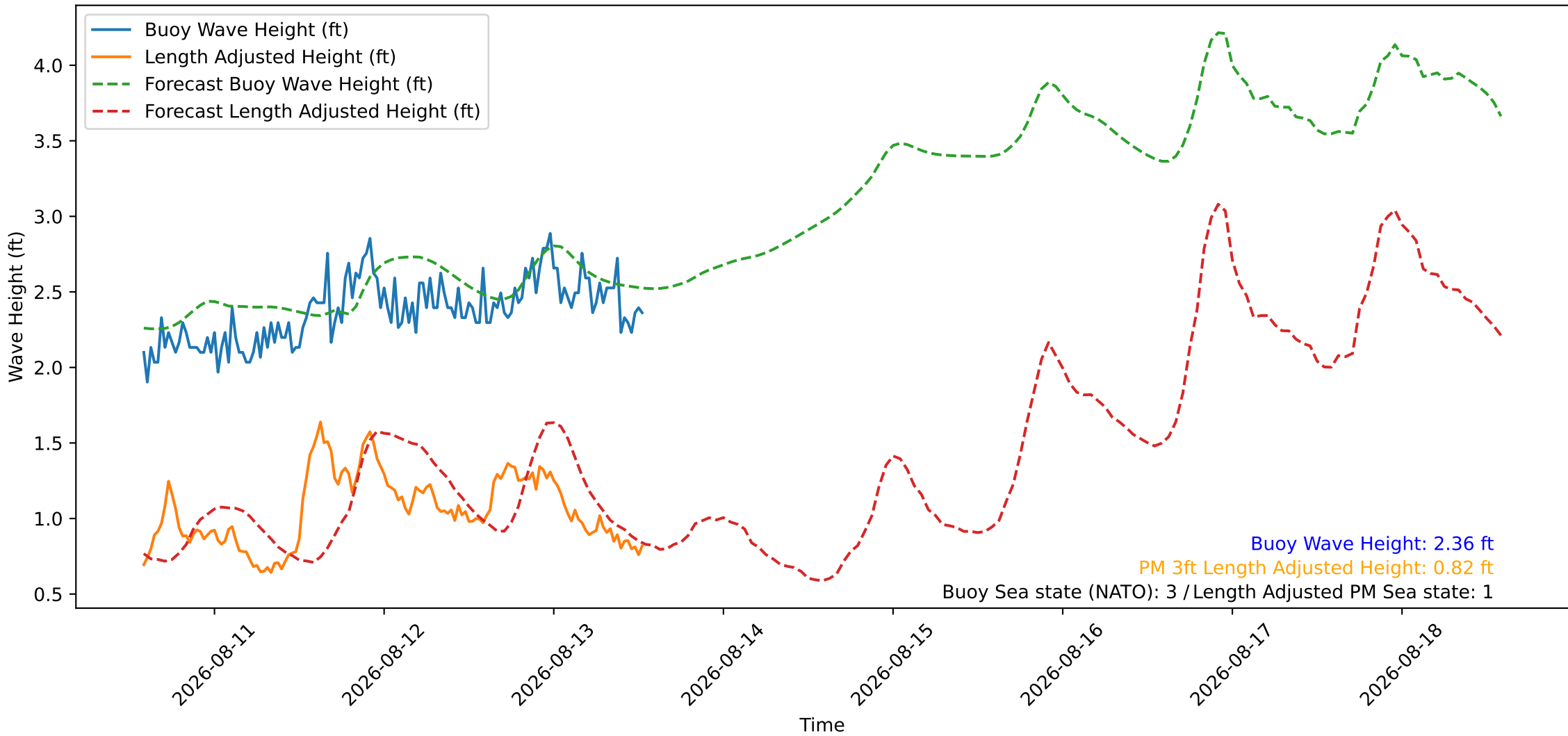
Wave Heights over Time for Red Beach at 2026-08-13 13:50:46
