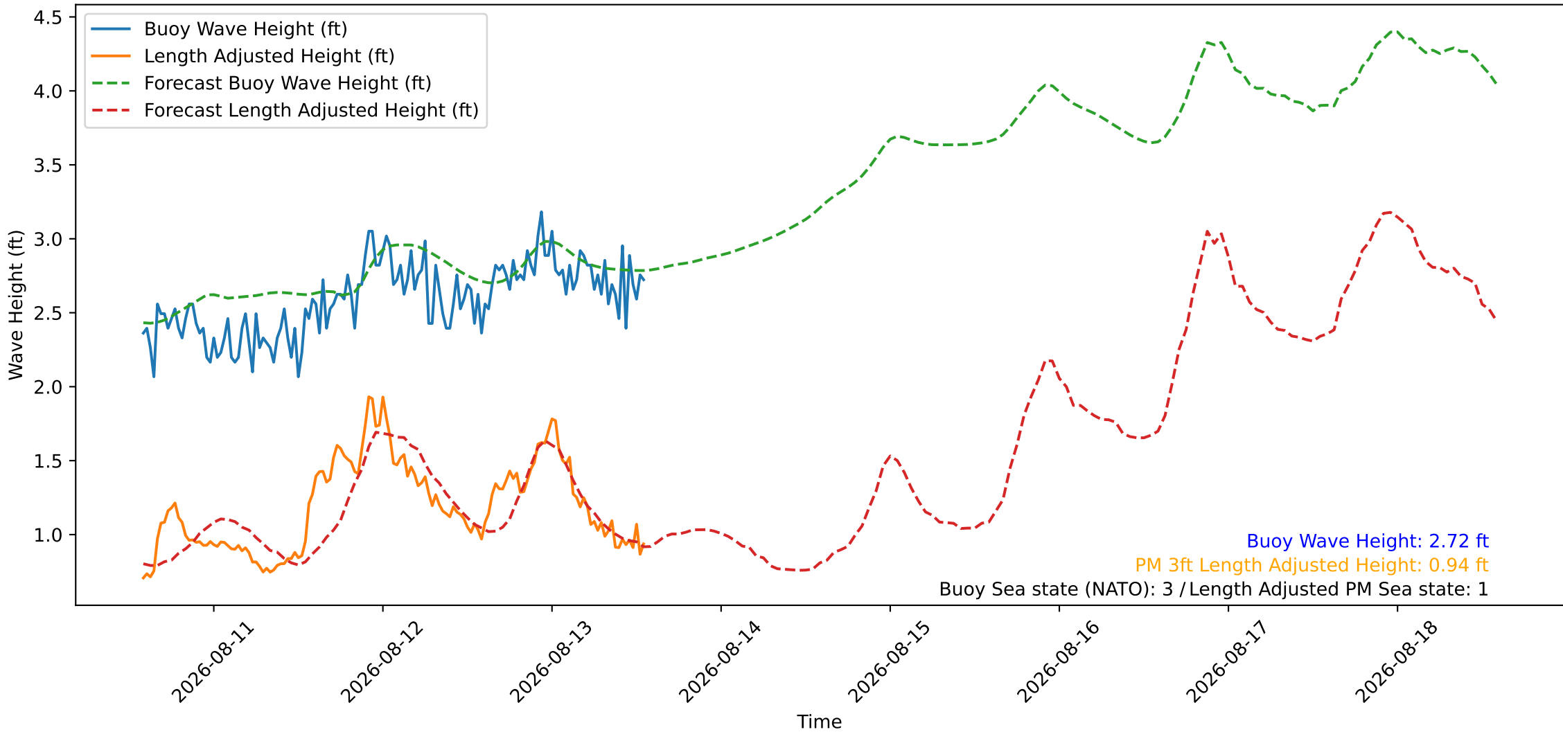
Wave Heights over Time for Oceanside Harbor at 2026-08-13 13:50:26
