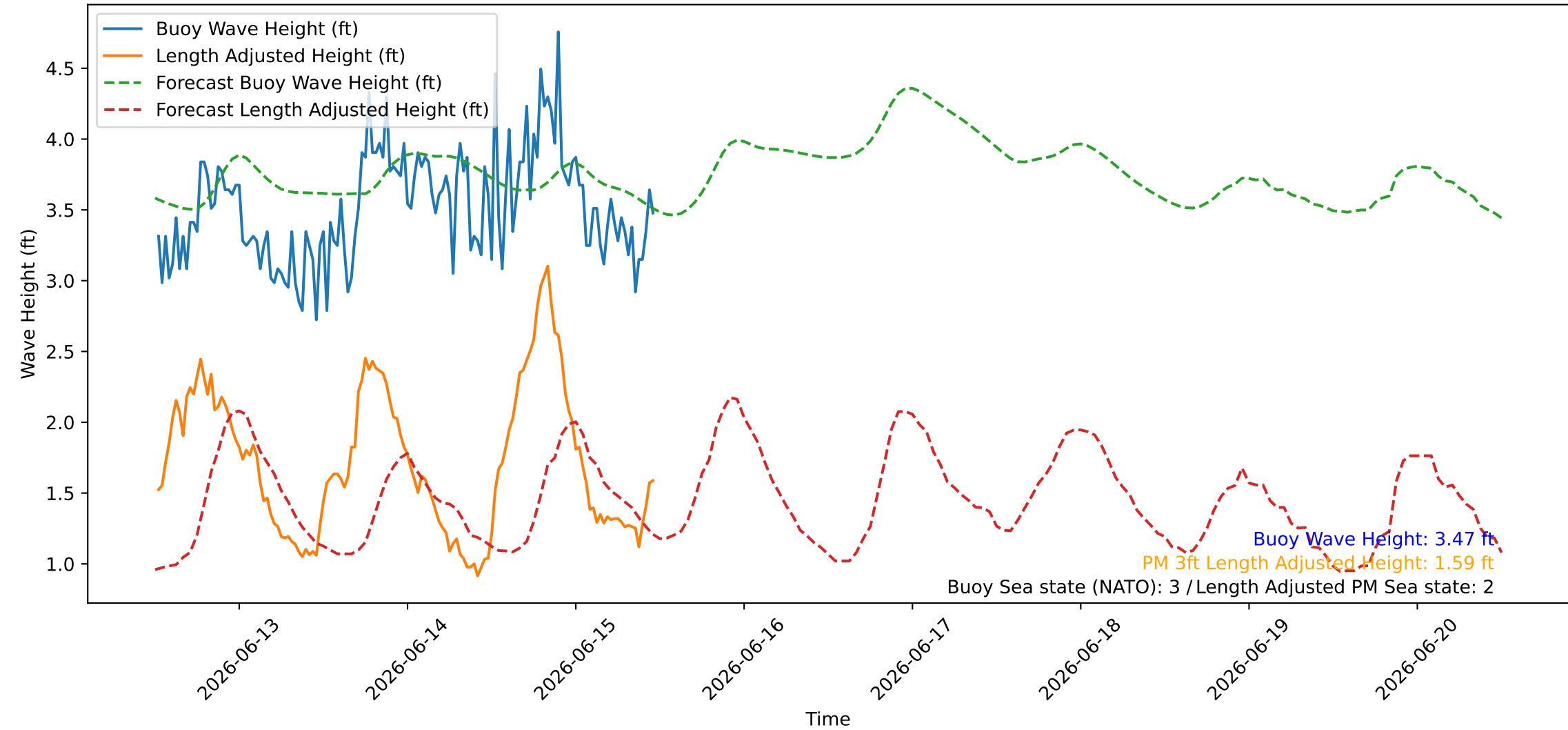
Wave Heights over Time for Red Beach at 2026-06-15 12:00:45
