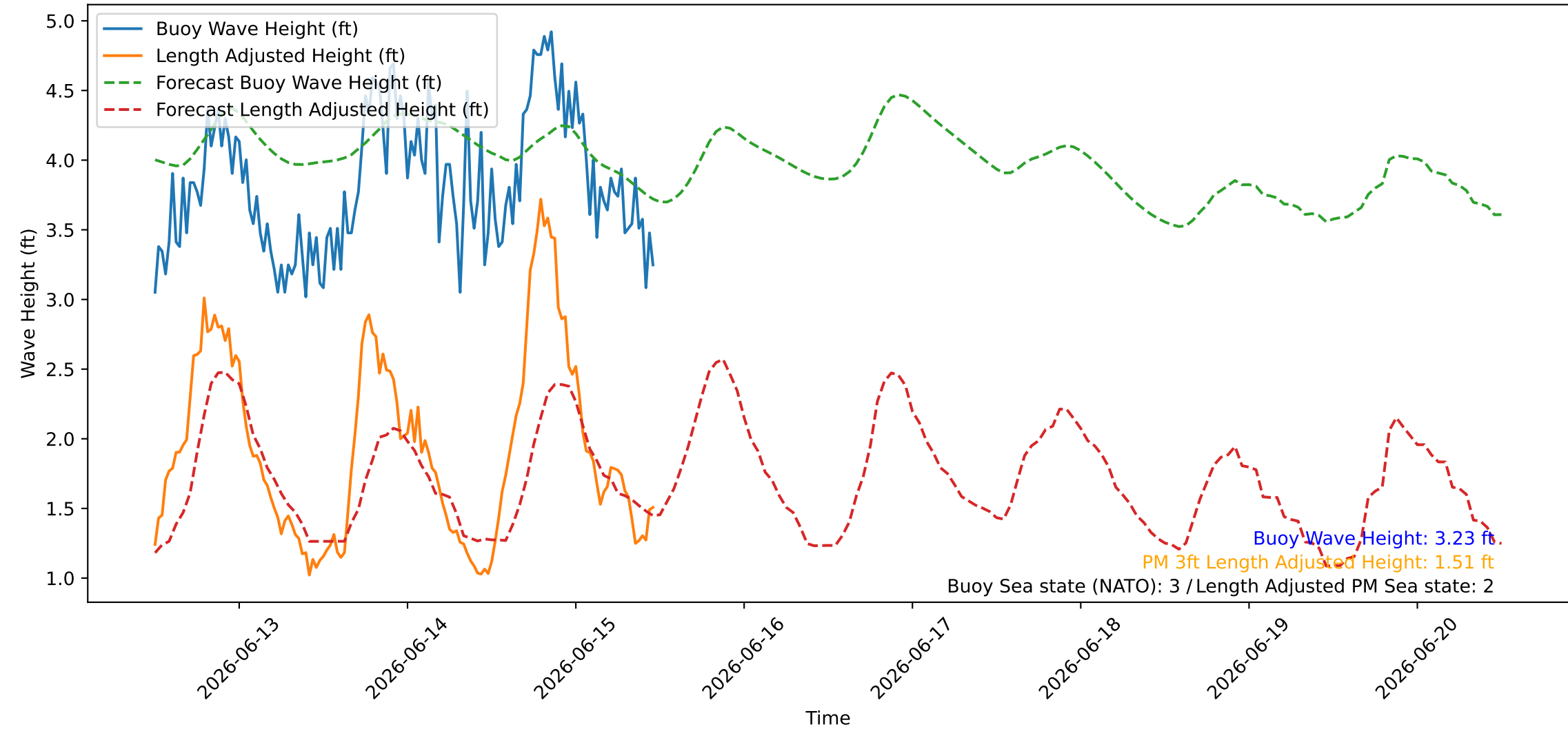
Wave Heights over Time for Green Beach at 2026-06-15 12:01:08
