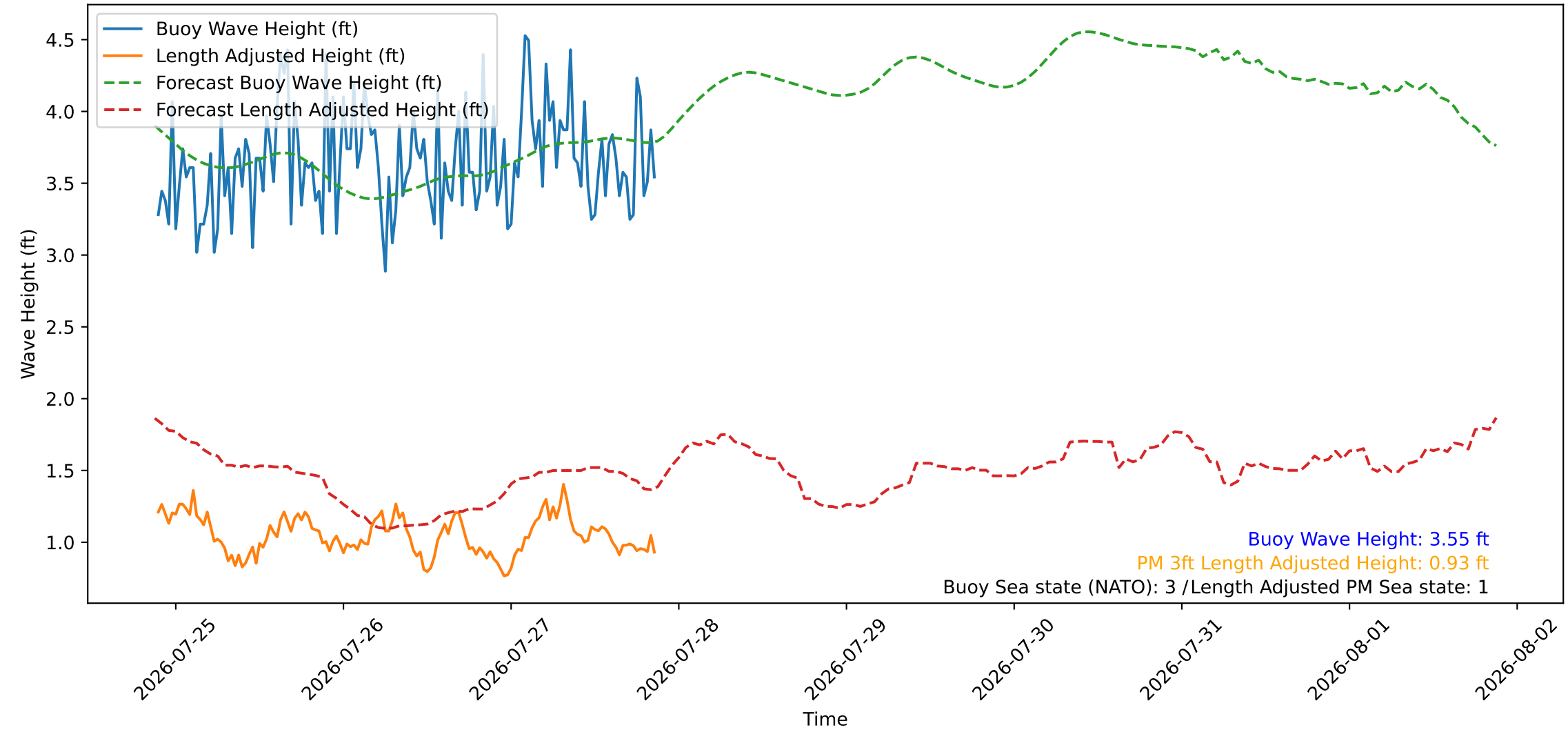
Wave Heights over Time for Red Beach at 2026-07-27 21:20:47
