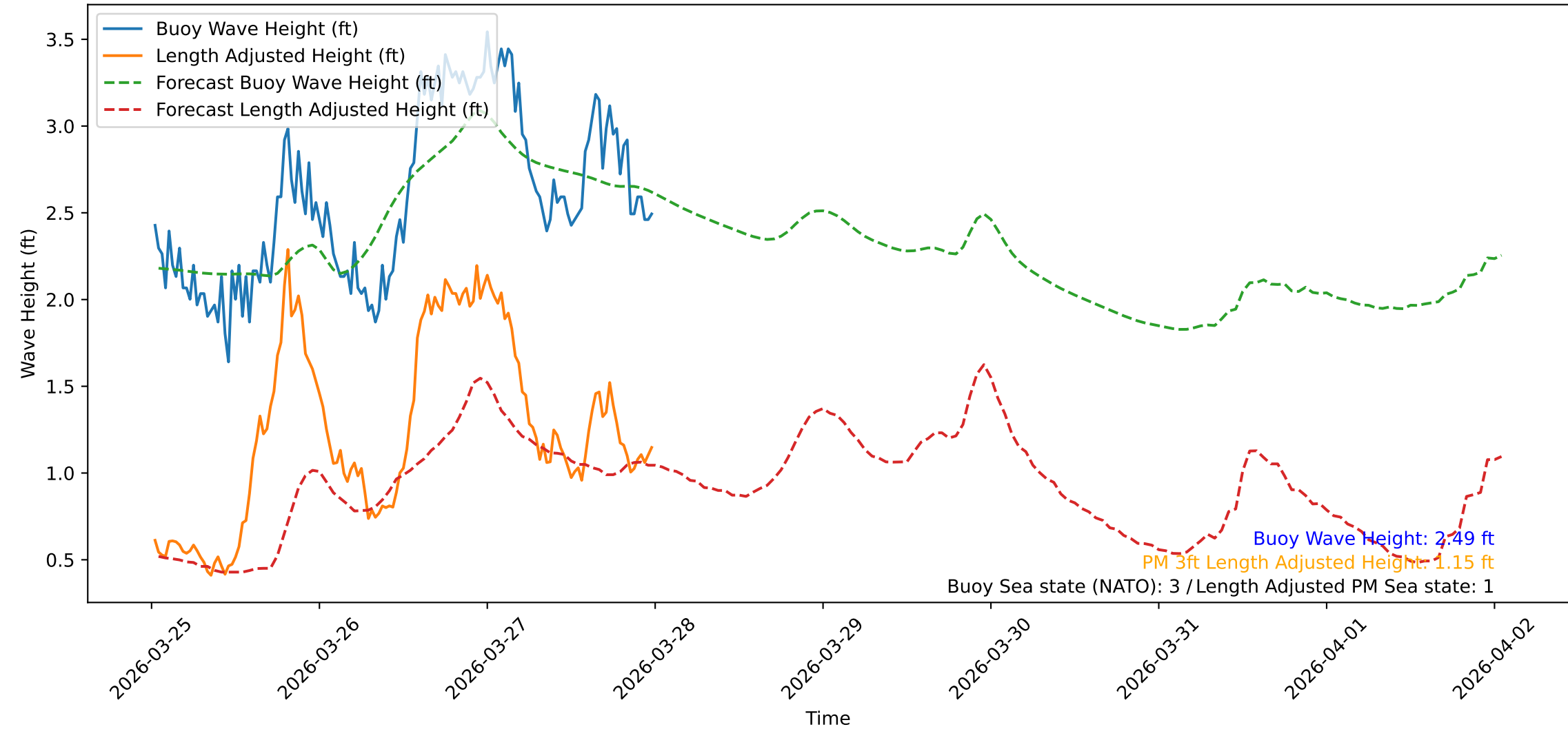
Wave Heights over Time for Green Beach at 2026-03-28 00:31:10
