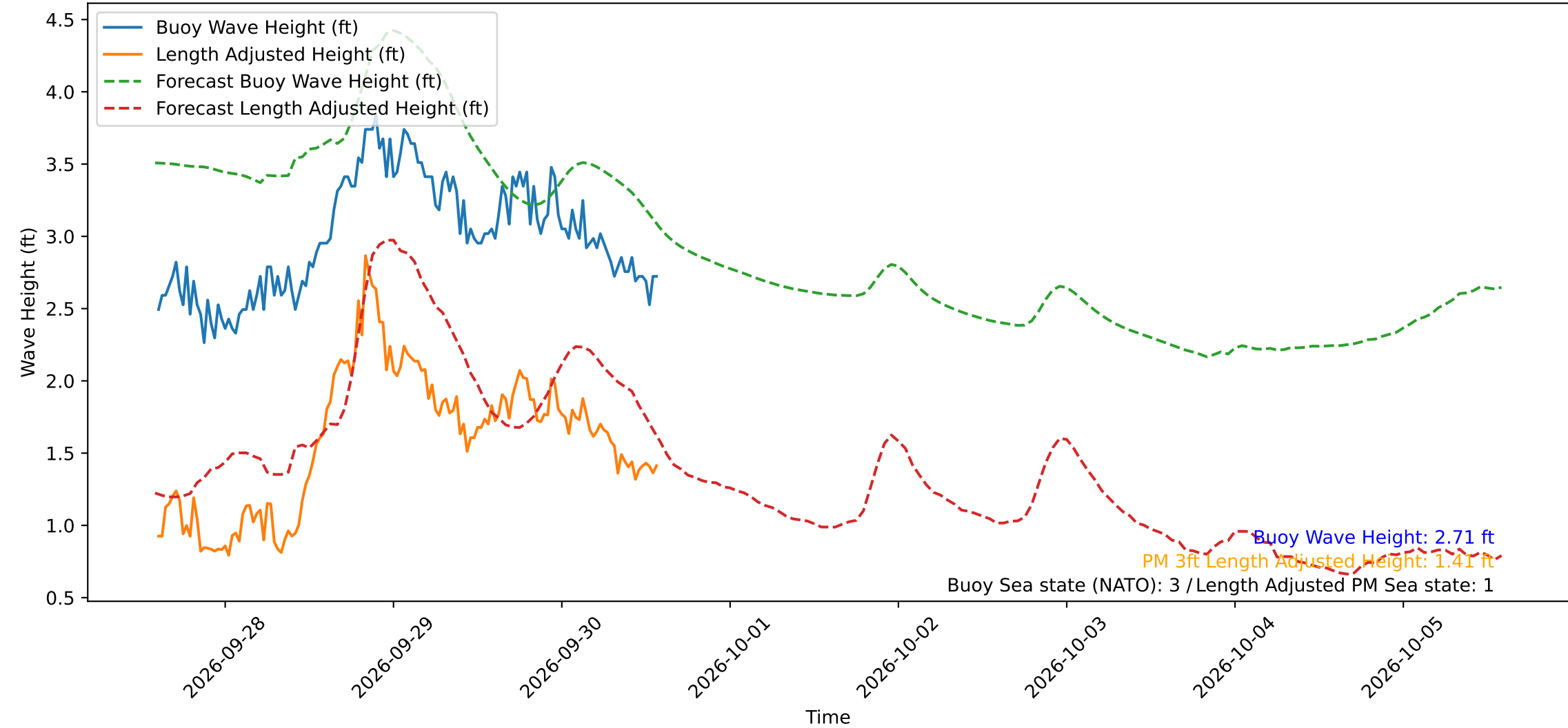
Wave Heights over Time for Red Beach at 2026-09-30 14:10:49
