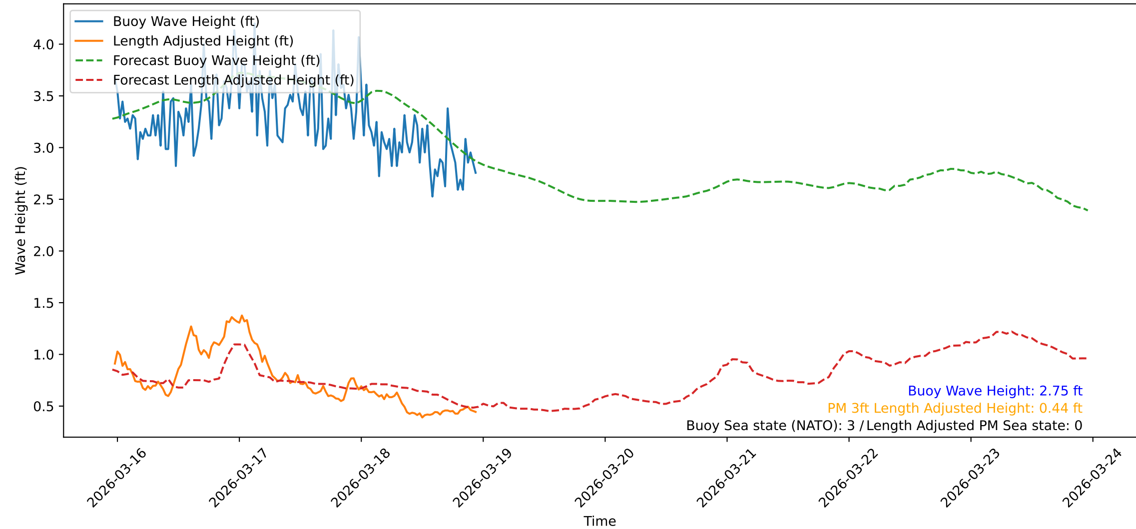
Wave Heights over Time for Green Beach at 2026-03-18 23:21:10
