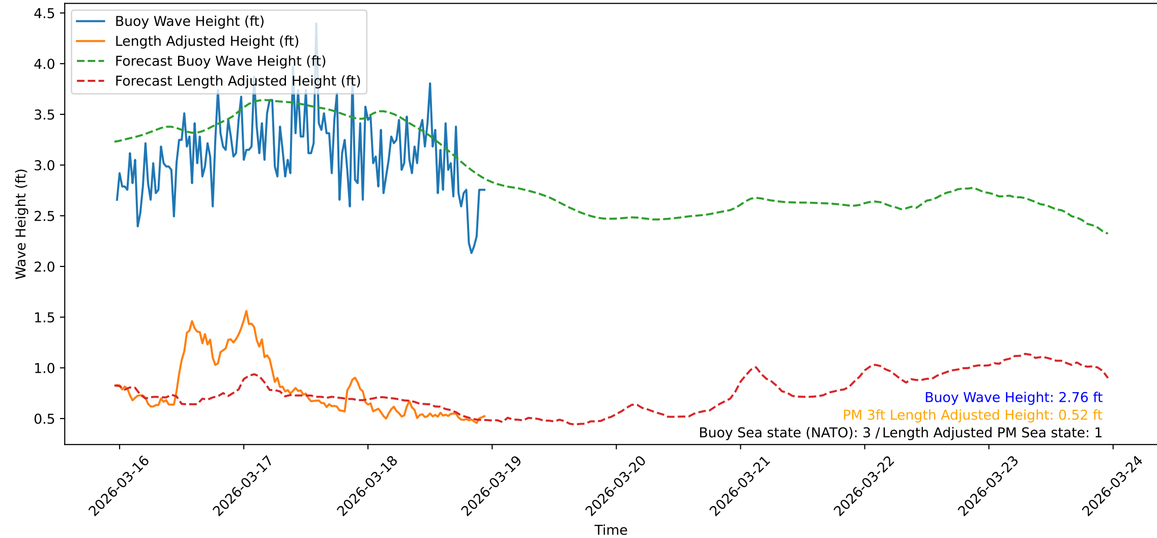
Wave Heights over Time for Oceanside Harbor at 2026-03-18 23:20:32
