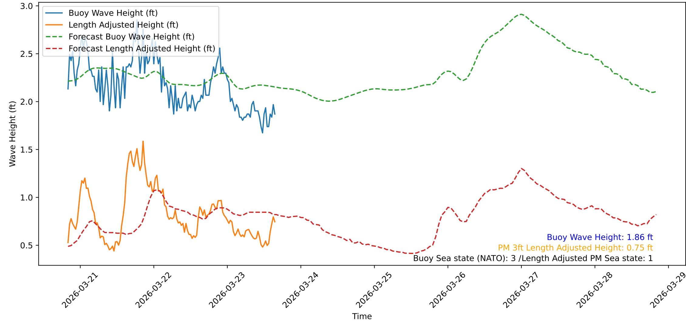
Wave Heights over Time for Red Beach at 2026-03-23 19:50:47
