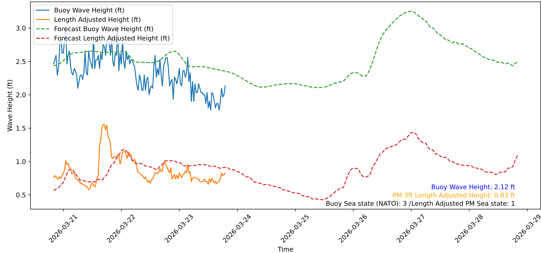
Wave Heights over Time for Oceanside Harbor at 2026-03-23 19:50:31
