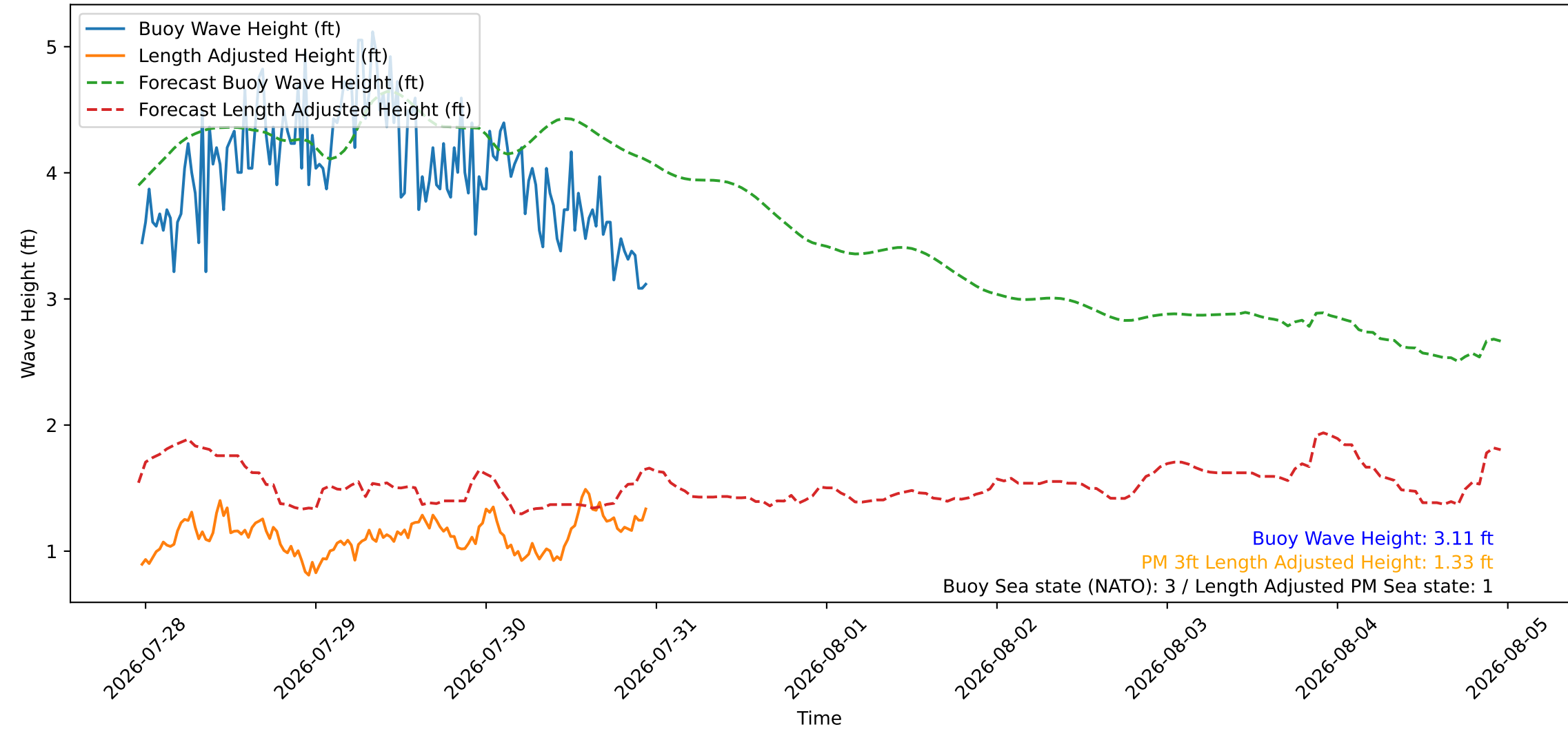
Wave Heights over Time for Red Beach at 2026-07-30 23:10:53
