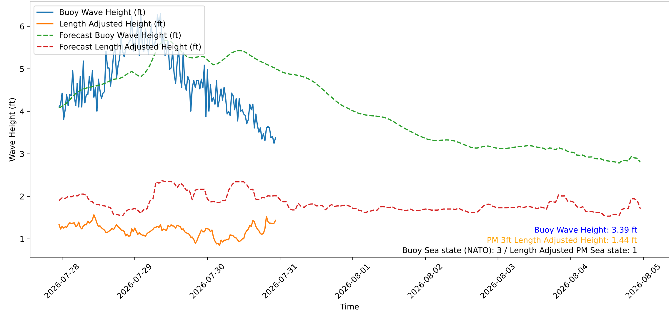
Wave Heights over Time for Green Beach at 2026-07-30 23:11:23
