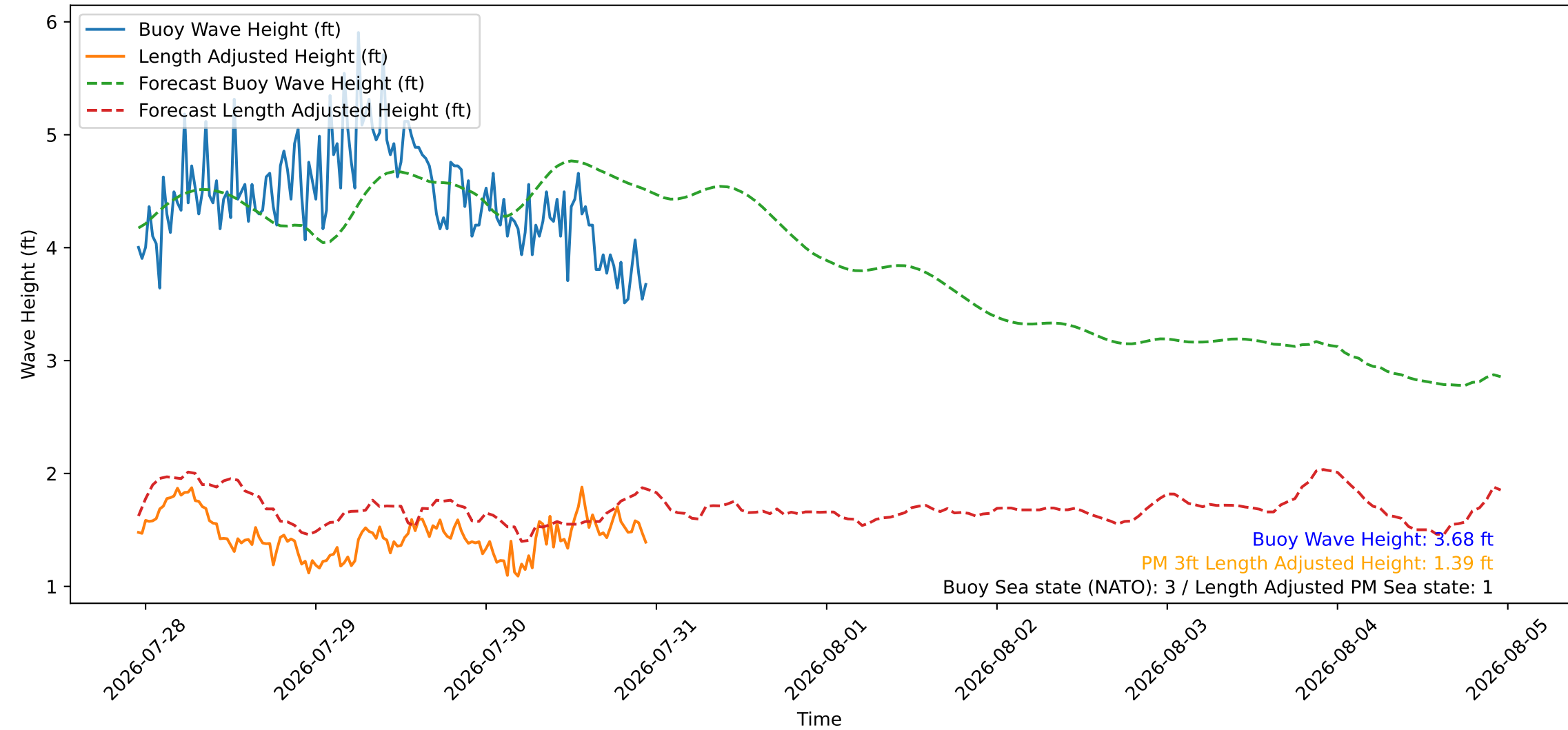
Wave Heights over Time for Oceanside Harbor at 2026-07-30 23:10:31
