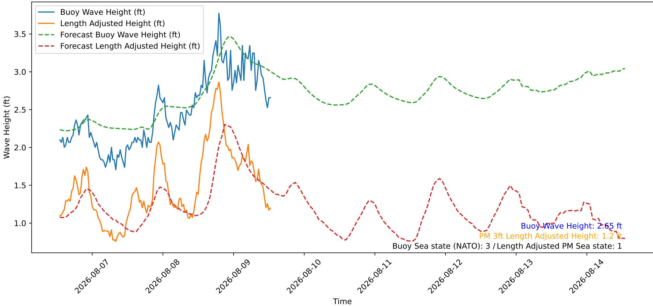
Wave Heights over Time for Green Beach at 2026-08-09 13:11:08
