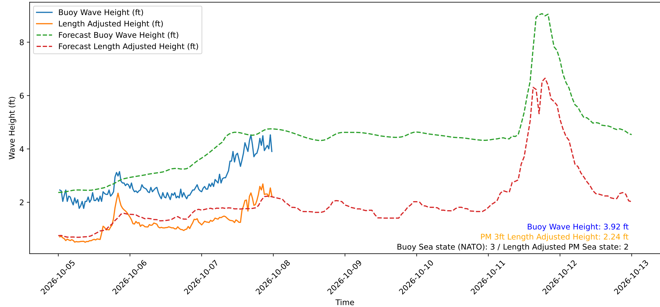
Wave Heights over Time for Green Beach at 2026-10-08 00:21:14
