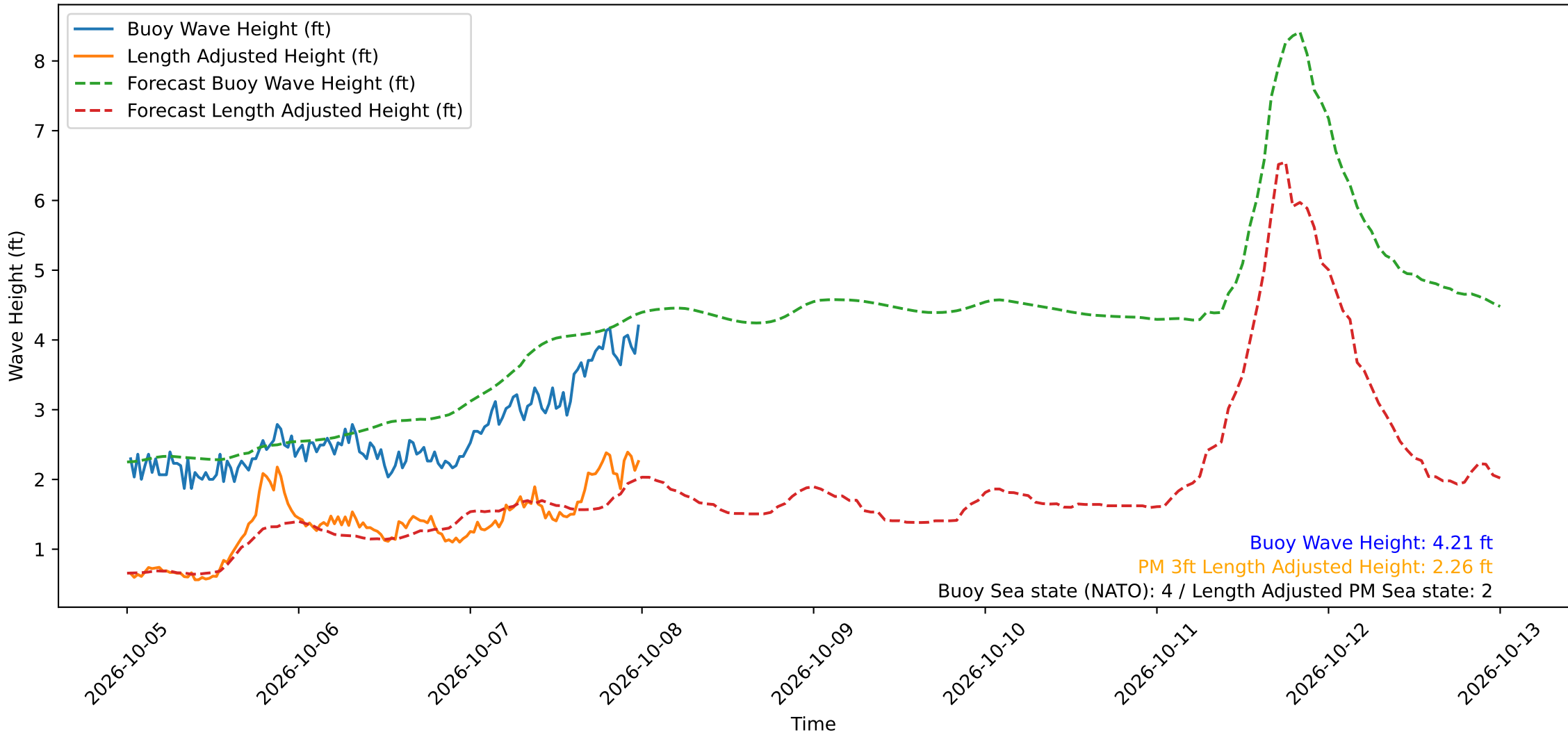
Wave Heights over Time for Oceanside Harbor at 2026-10-08 00:20:29
