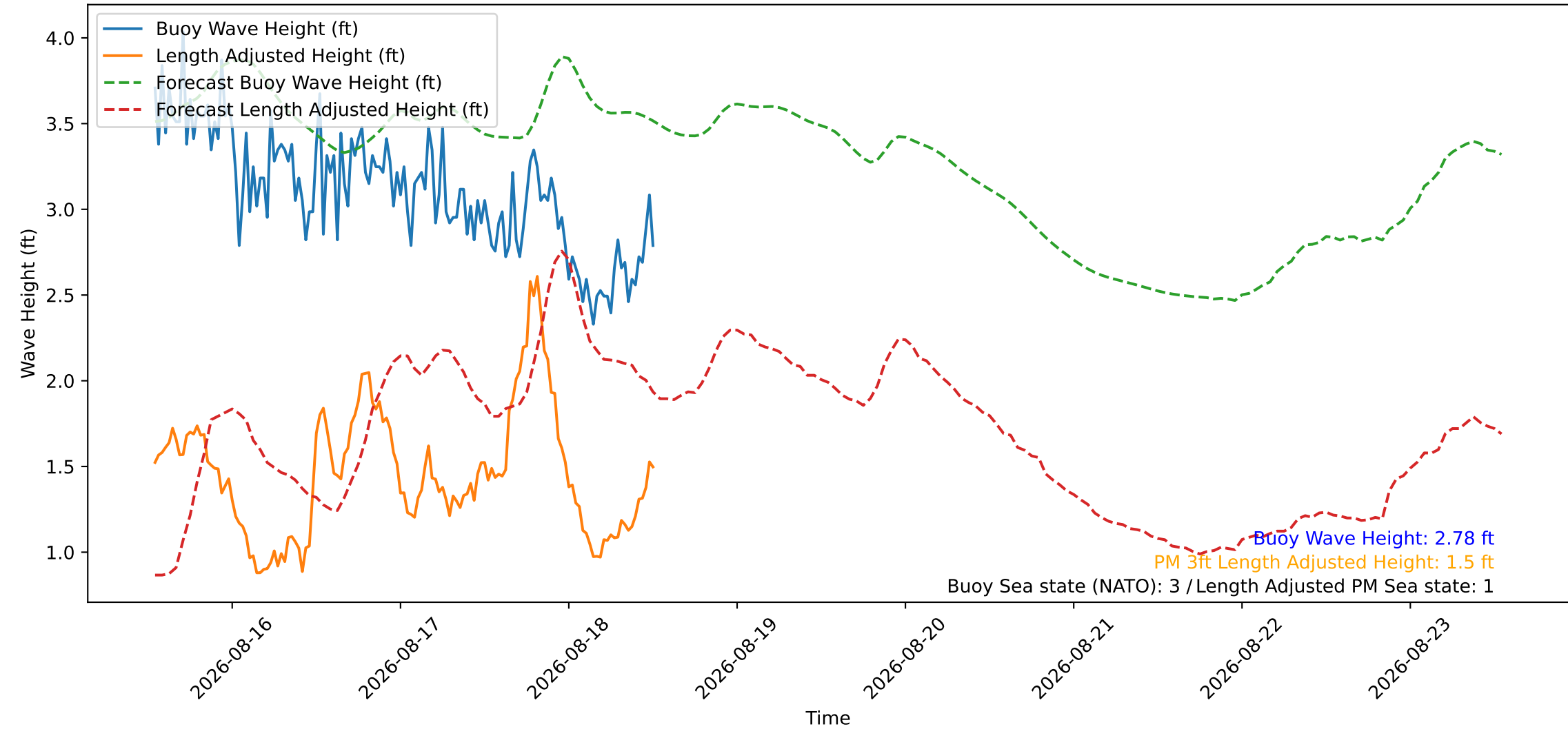
Wave Heights over Time for Red Beach at 2026-08-18 12:40:46
