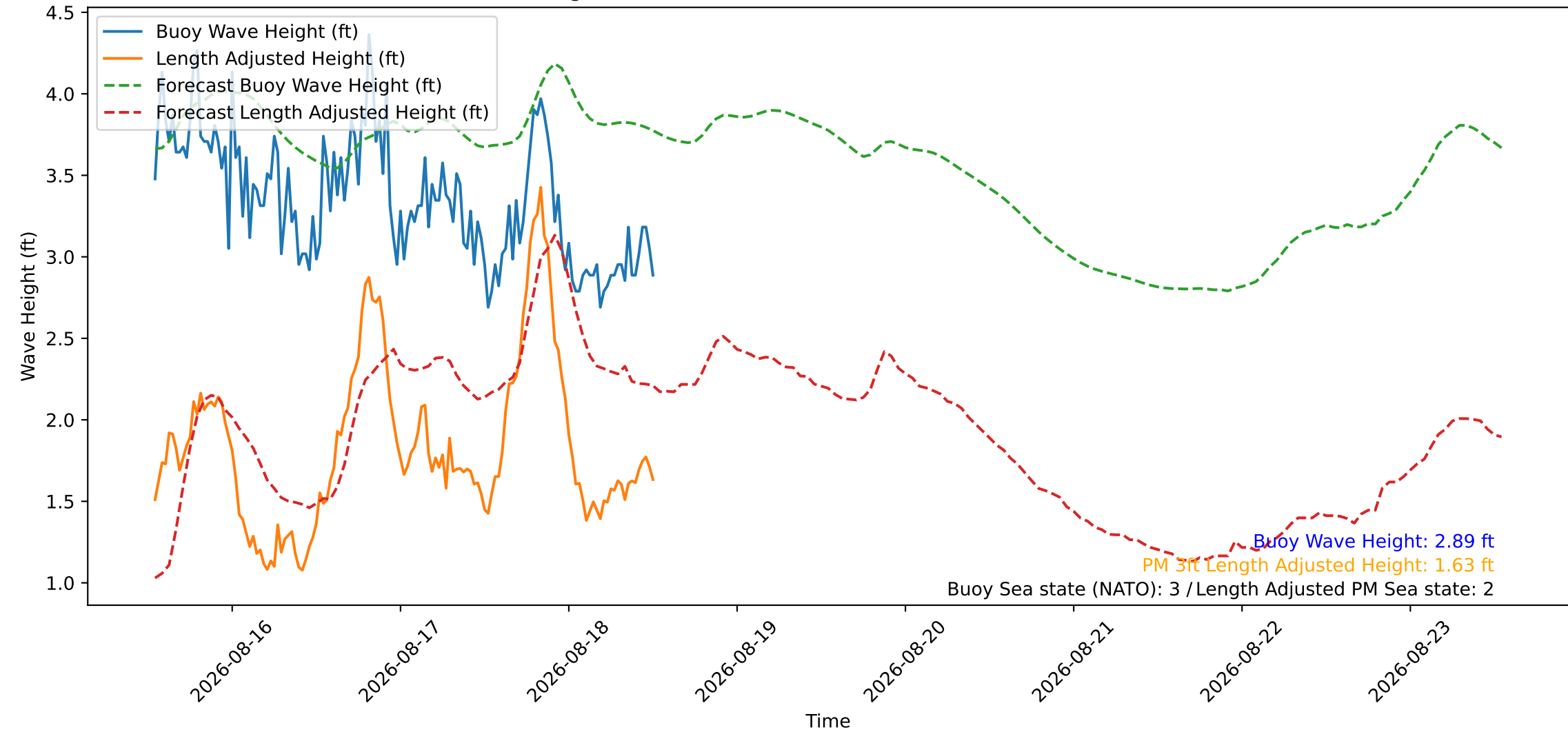
Wave Heights over Time for Green Beach at 2026-08-18 12:41:08
