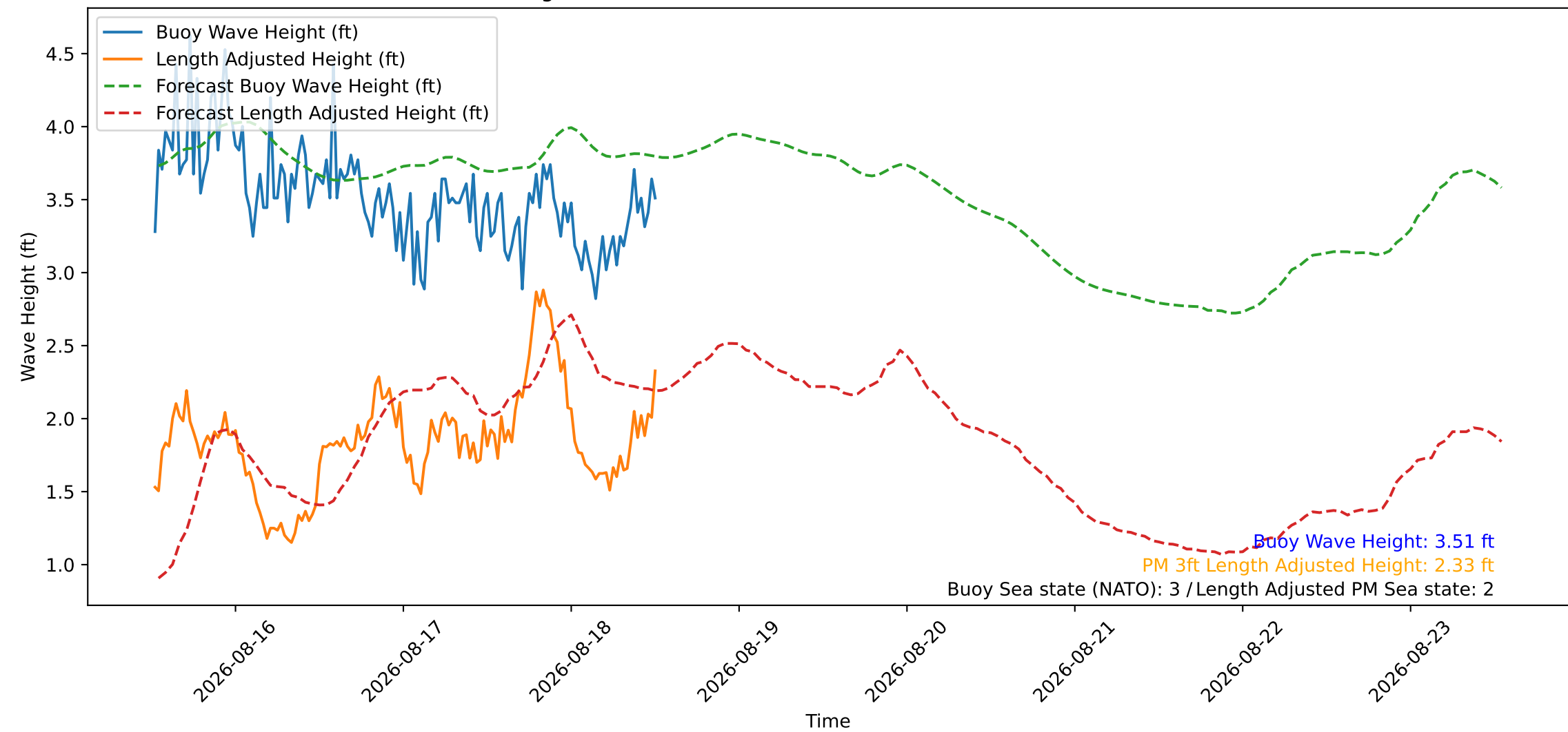
Wave Heights over Time for Oceanside Harbor at 2026-08-18 12:40:26
