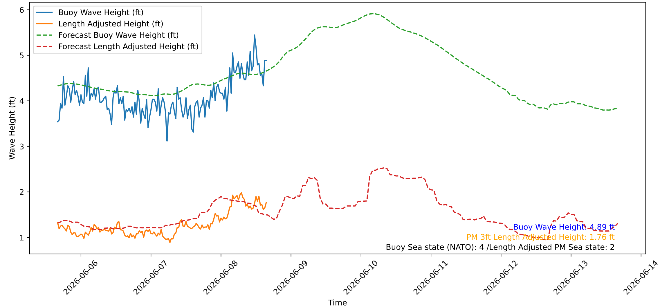
Wave Heights over Time for Green Beach at 2026-06-08 16:11:08
