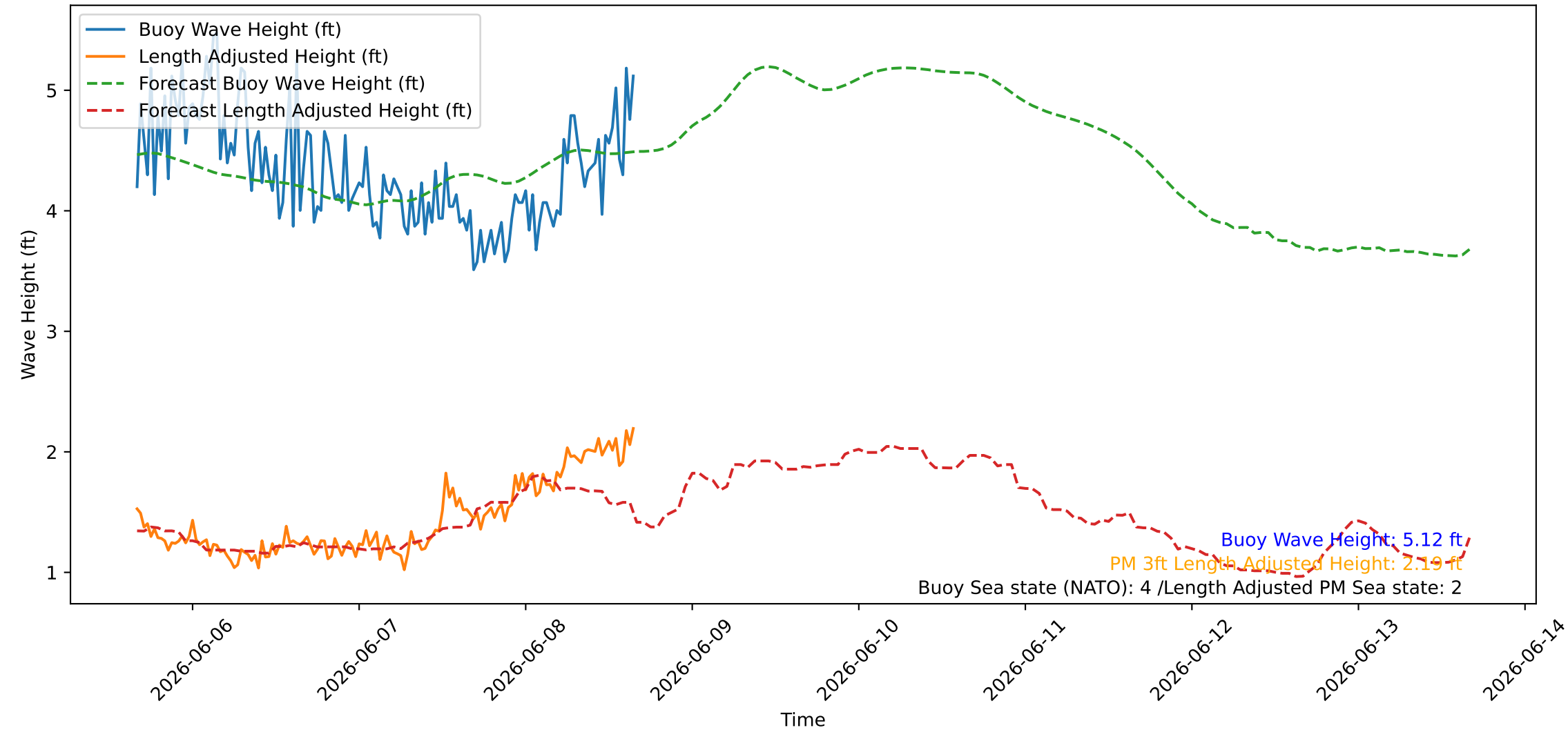
Wave Heights over Time for Oceanside Harbor at 2026-06-08 16:10:26
