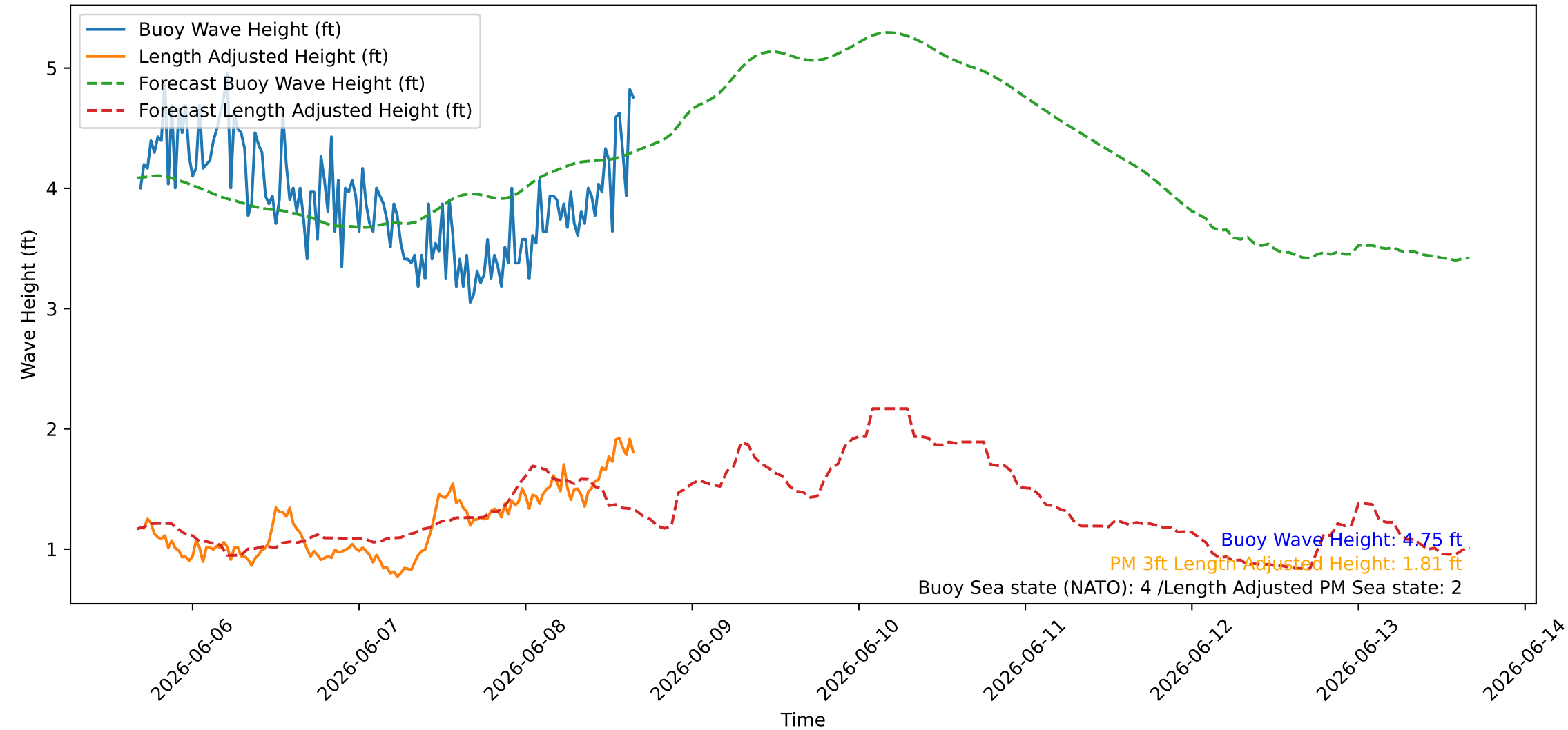
Wave Heights over Time for Red Beach at 2026-06-08 16:10:45
