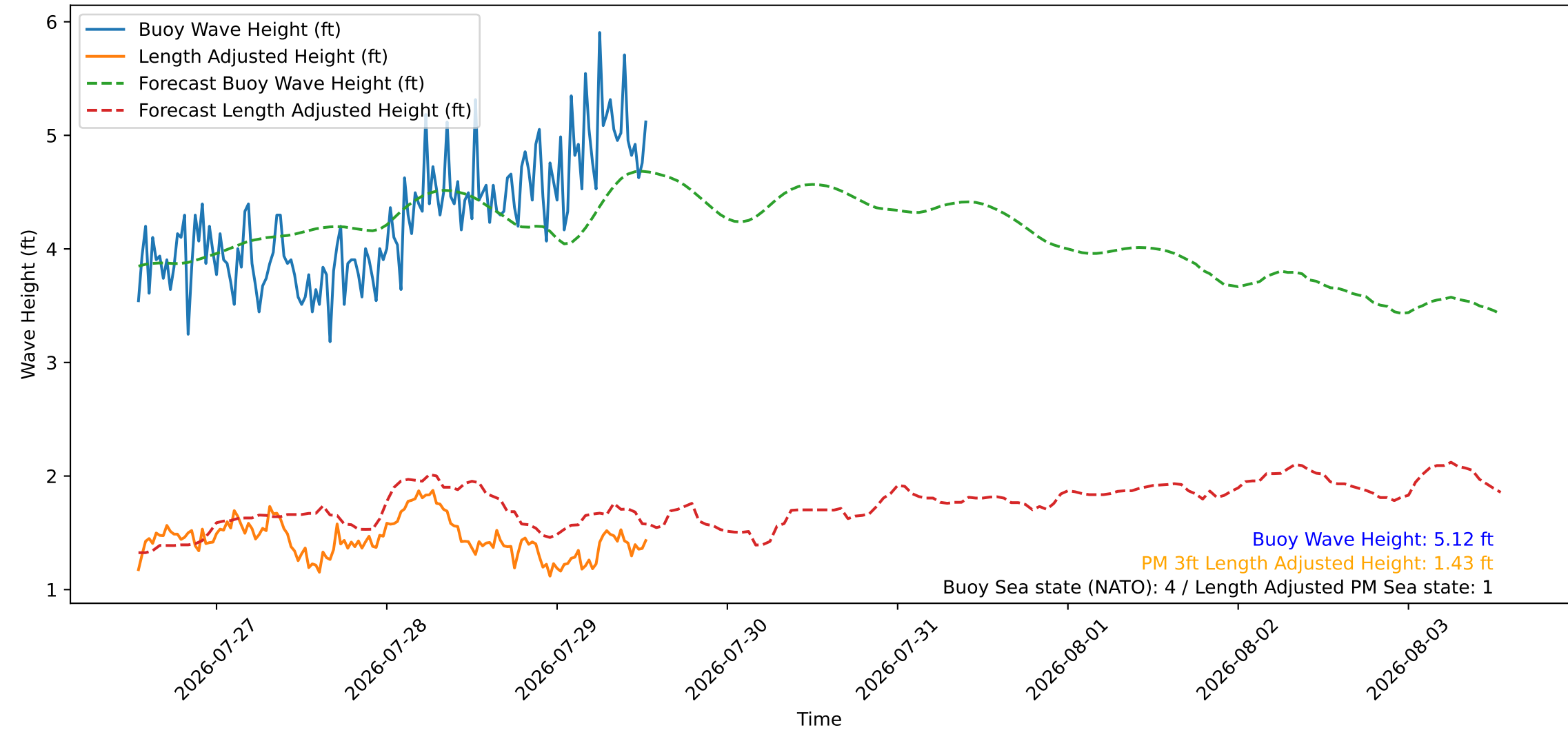
Wave Heights over Time for Oceanside Harbor at 2026-07-29 13:00:27
