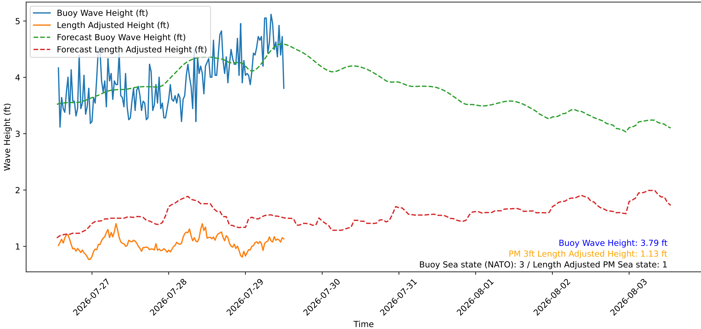
Wave Heights over Time for Red Beach at 2026-07-29 13:00:47
