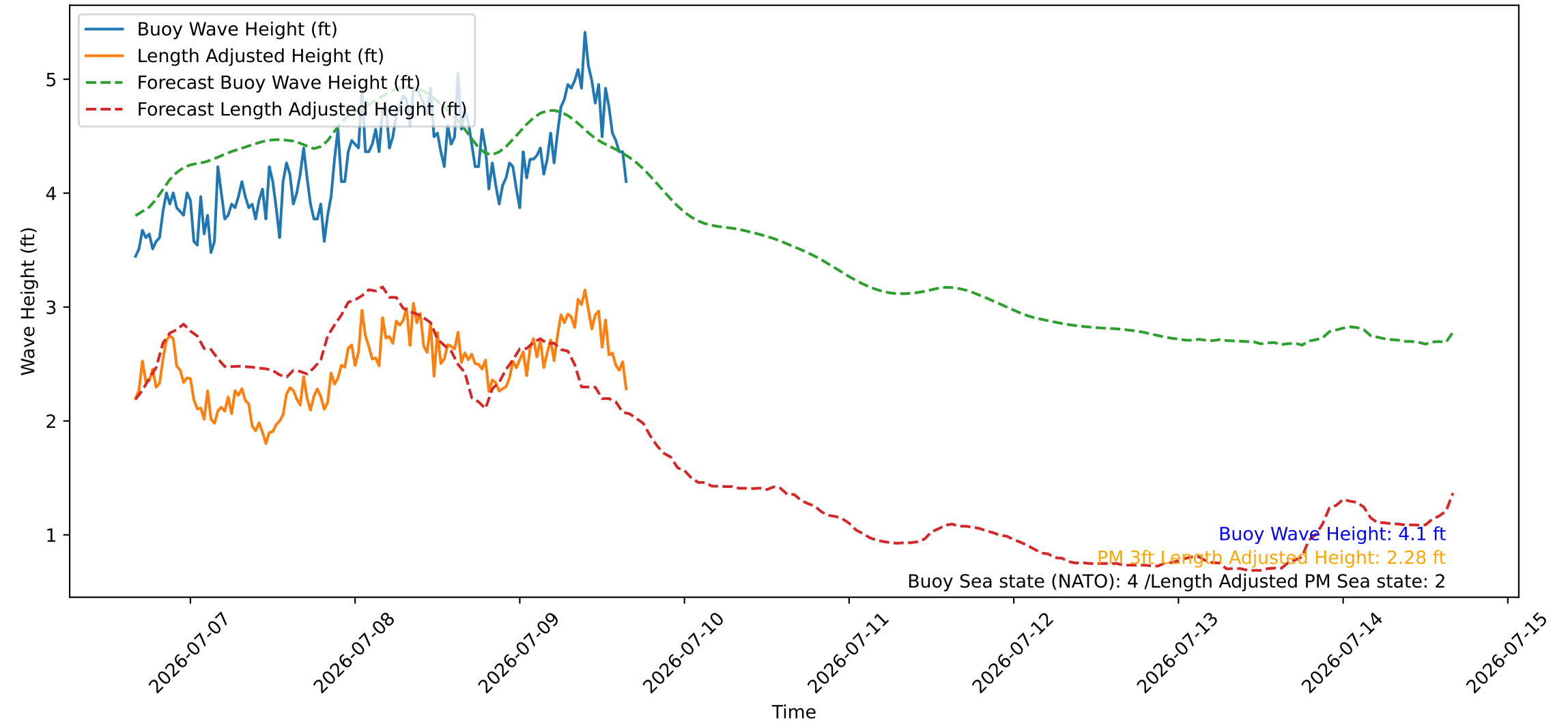
Wave Heights over Time for Oceanside Harbor at 2026-07-09 16:10:26
