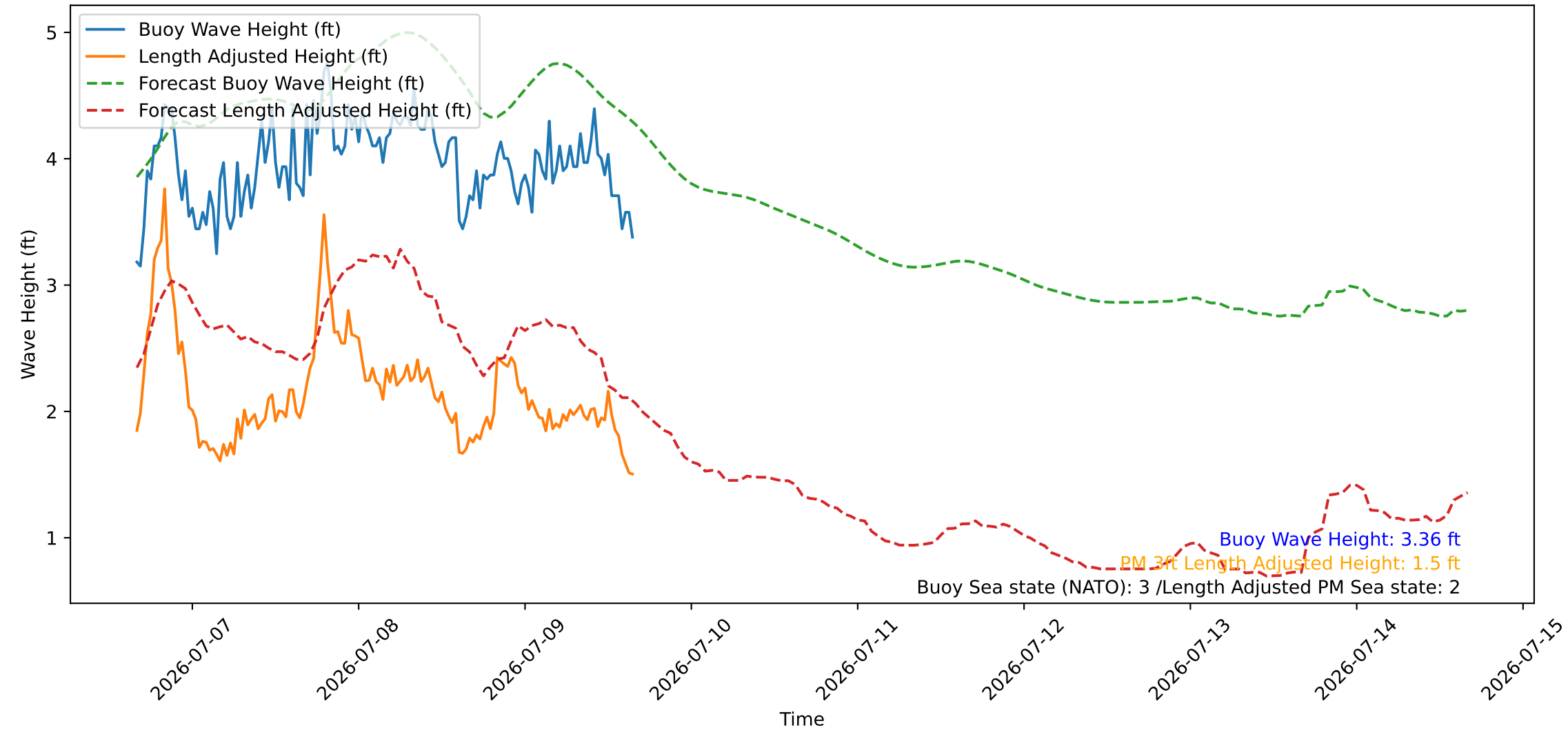
Wave Heights over Time for Green Beach at 2026-07-09 16:11:08
