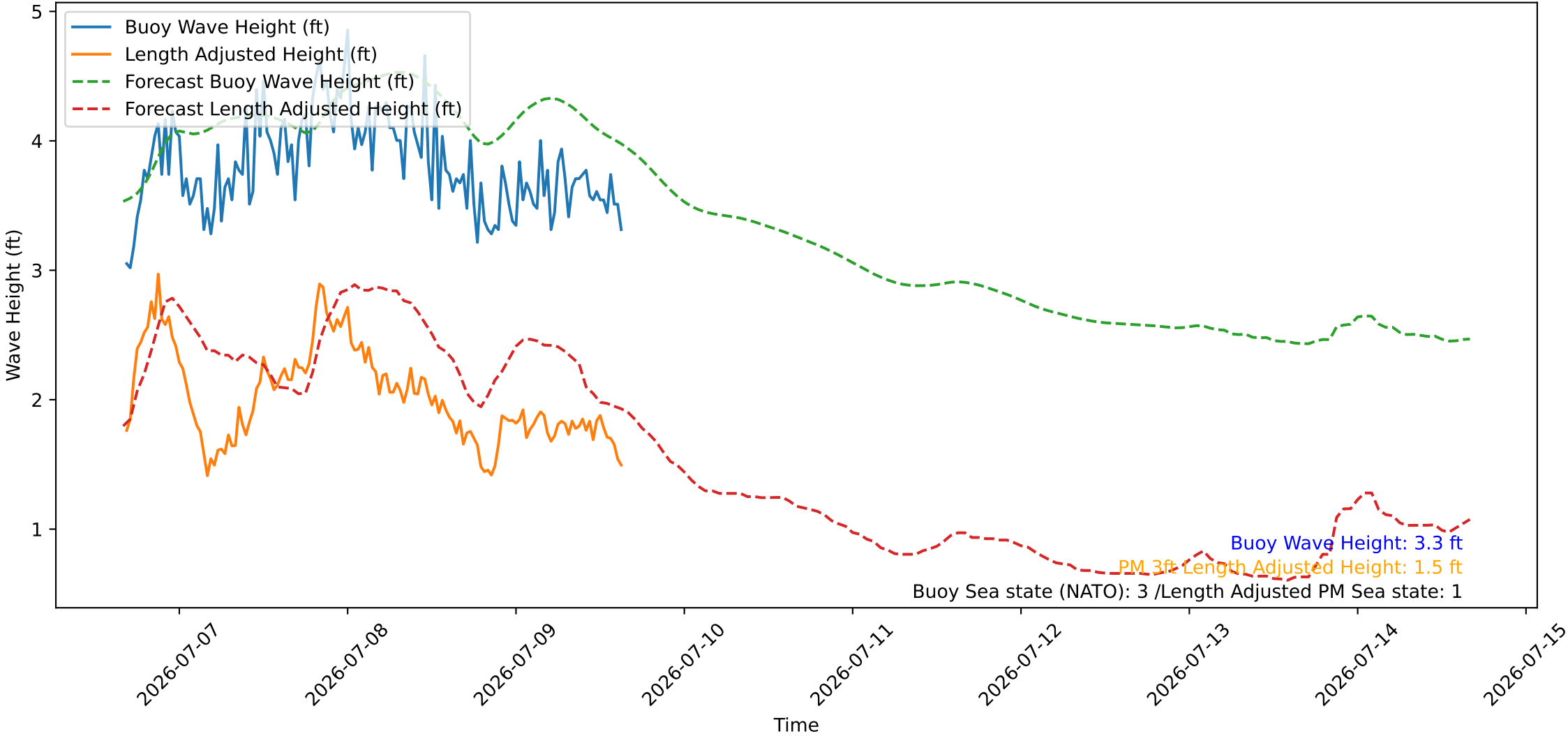
Wave Heights over Time for Red Beach at 2026-07-09 16:10:45
