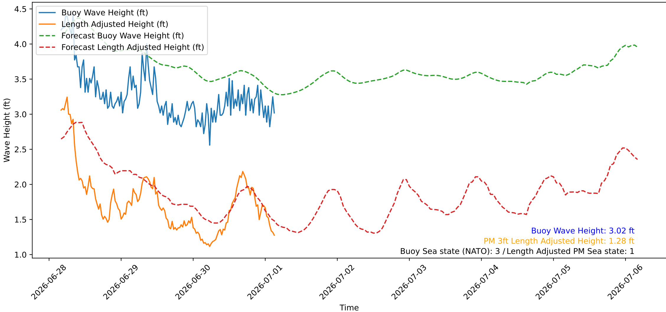
Wave Heights over Time for Oceanside Harbor at 2026-07-01 04:00:26
