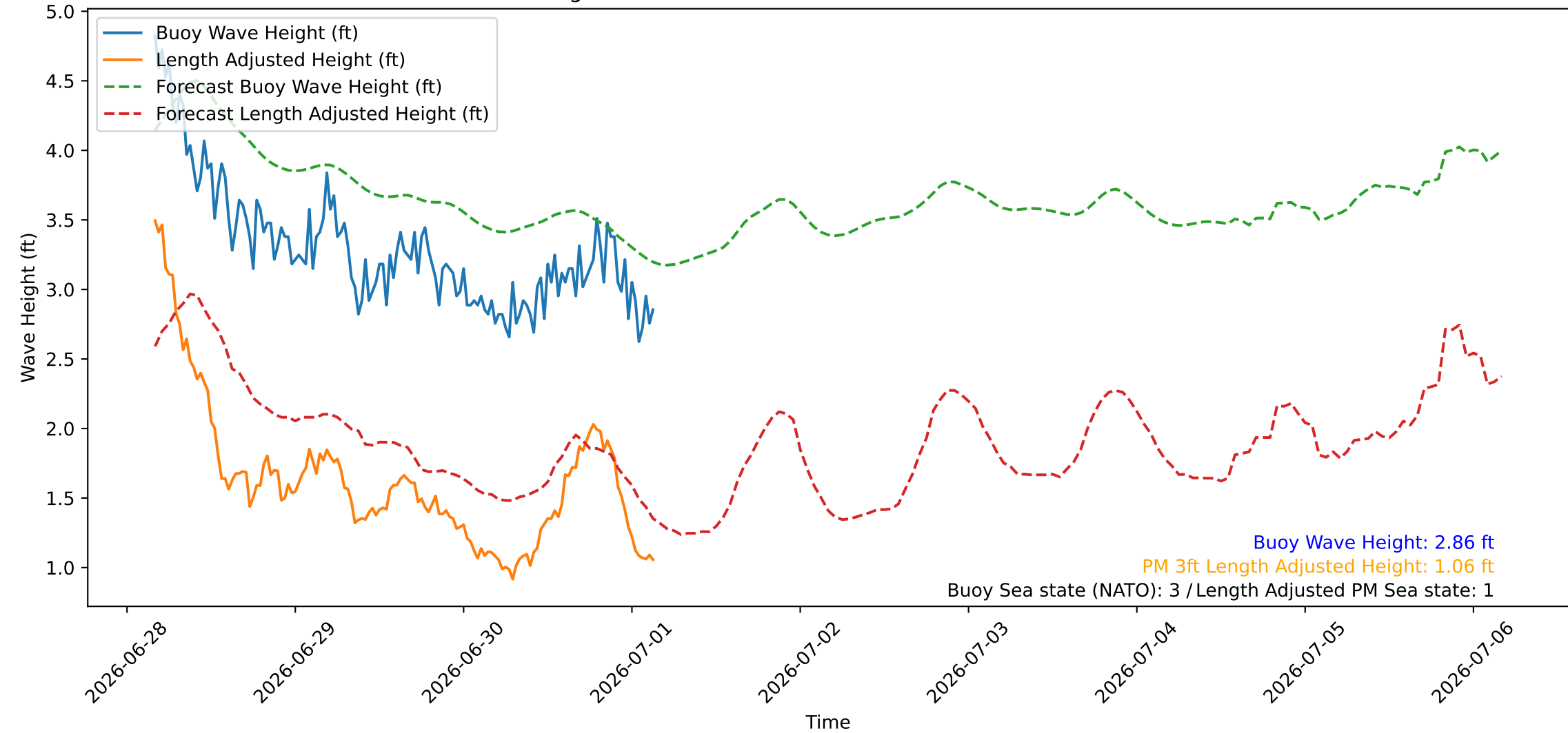
Wave Heights over Time for Green Beach at 2026-07-01 04:01:08
