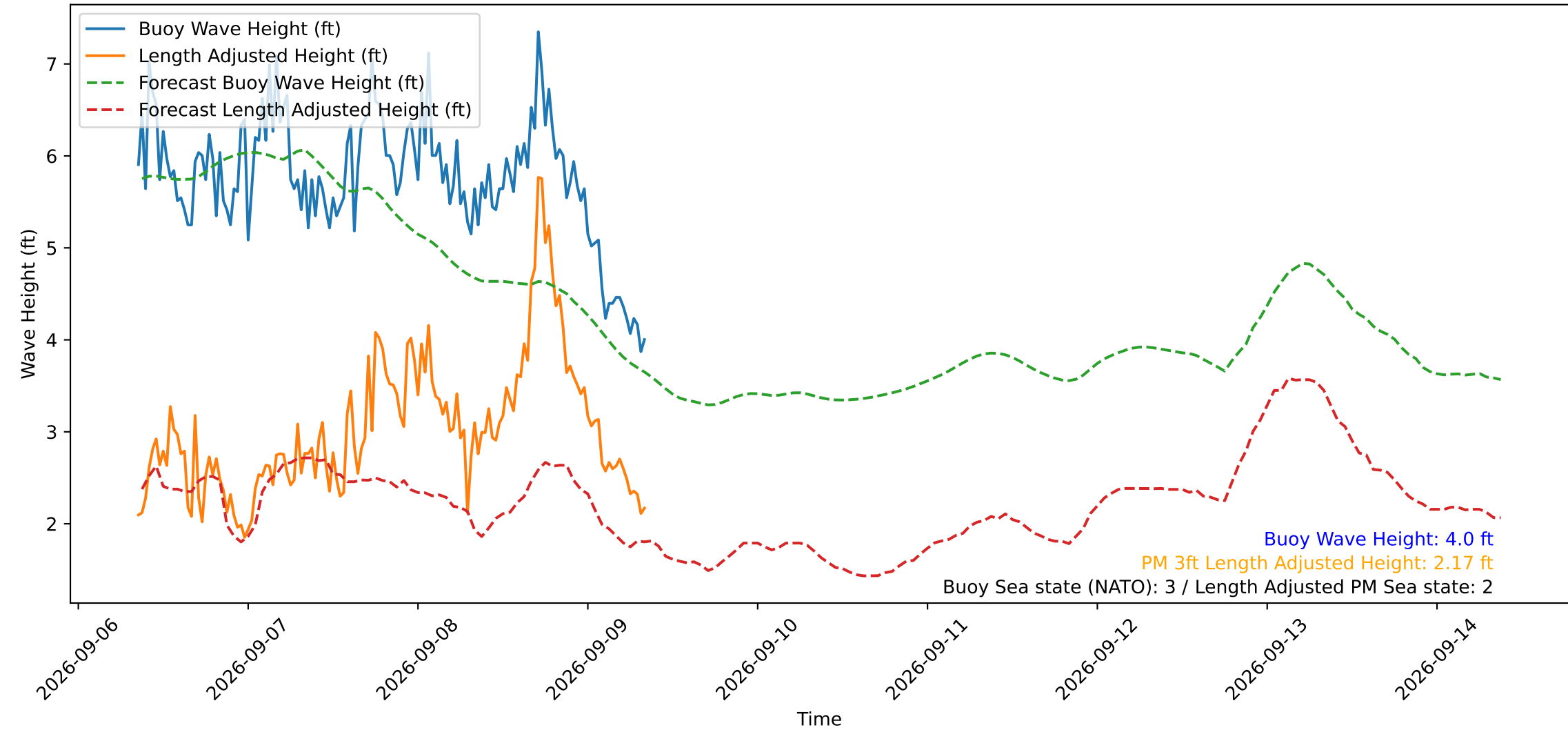
Wave Heights over Time for Oceanside Harbor at 2026-09-09 08:40:29
