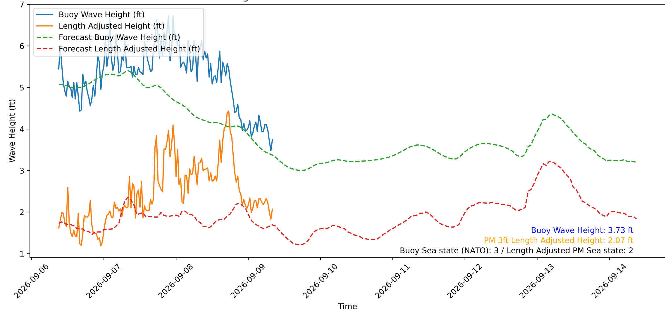
Wave Heights over Time for Red Beach at 2026-09-09 08:40:49
