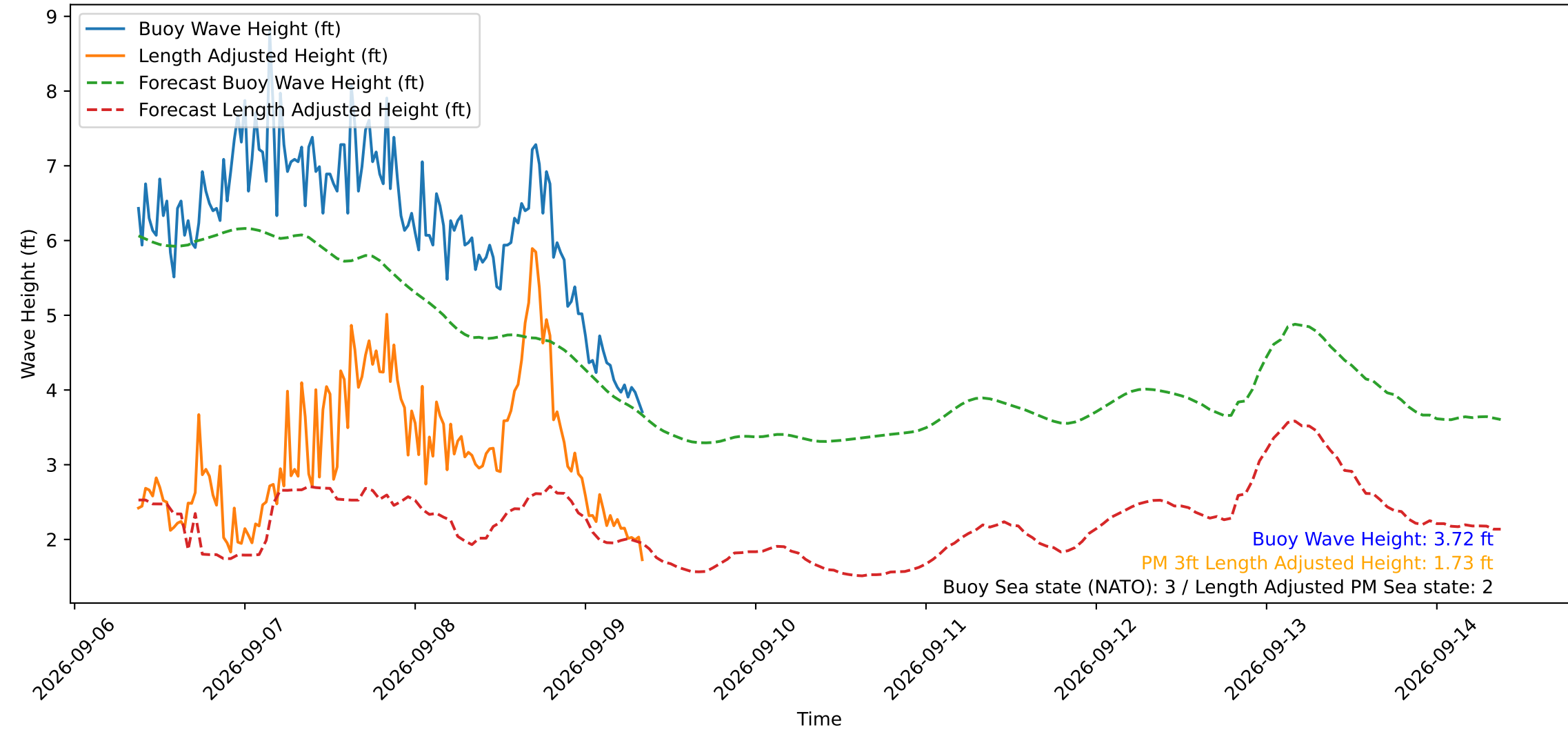
Wave Heights over Time for Green Beach at 2026-09-09 08:41:12
