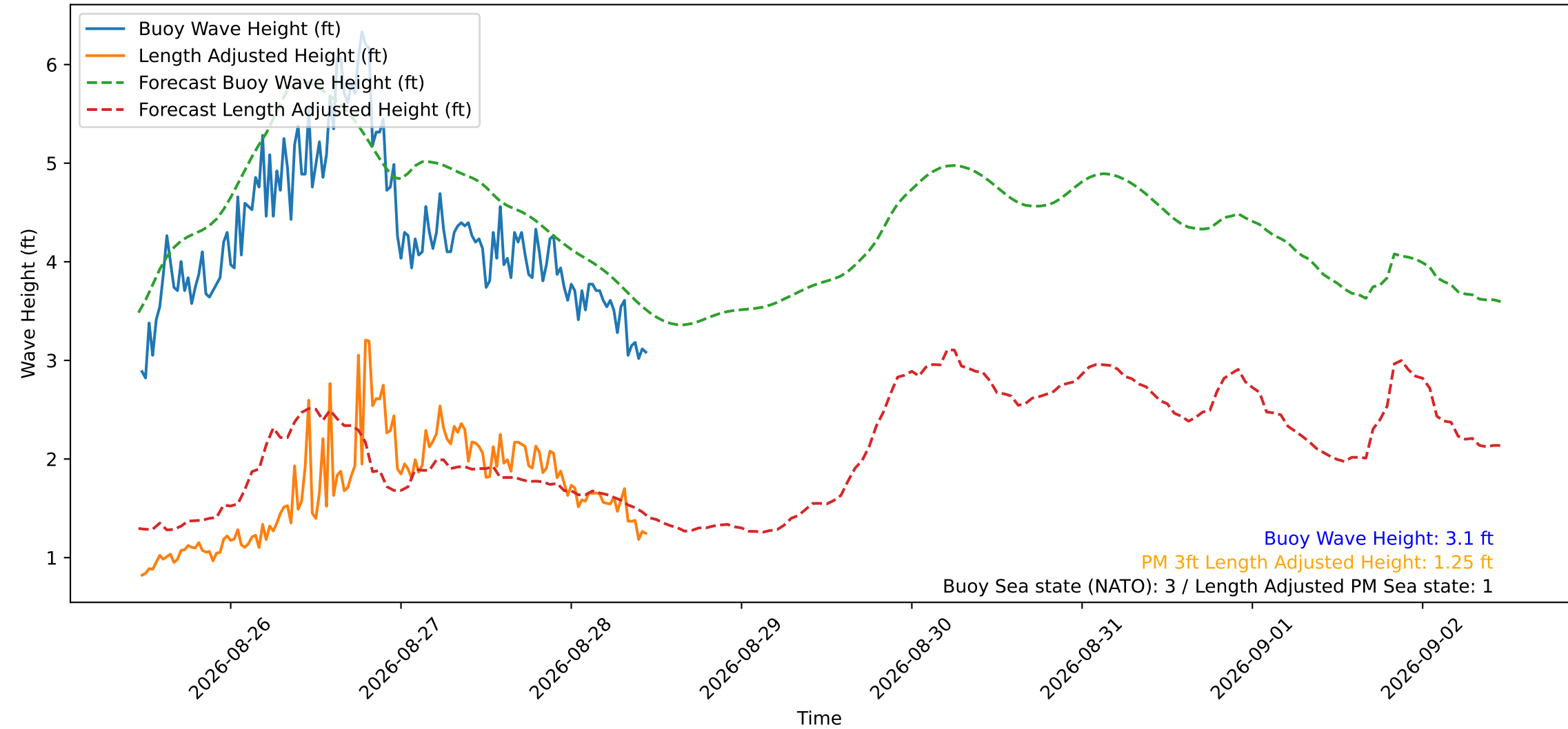
Wave Heights over Time for Green Beach at 2026-08-28 11:21:14
