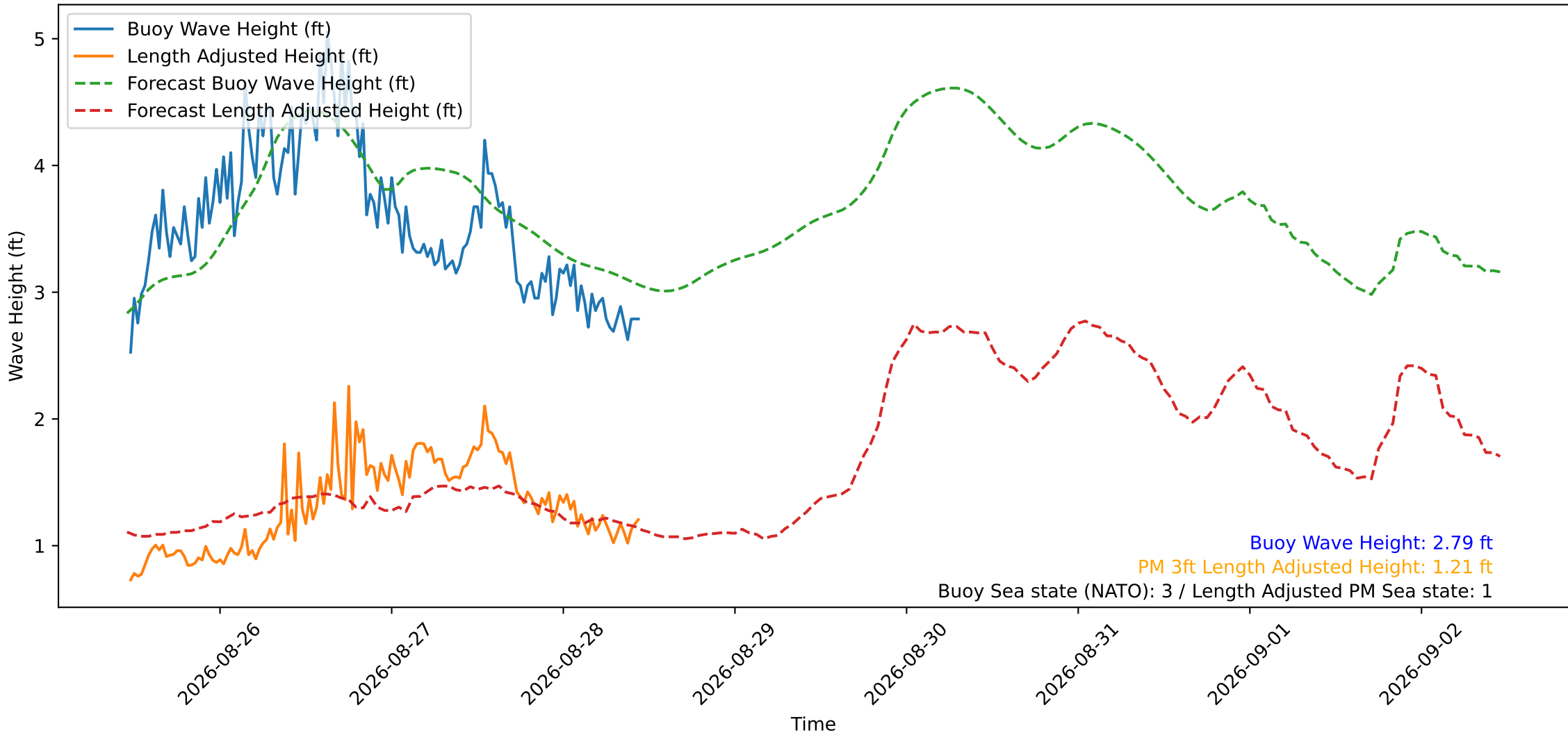
Wave Heights over Time for Red Beach at 2026-08-28 11:20:50
