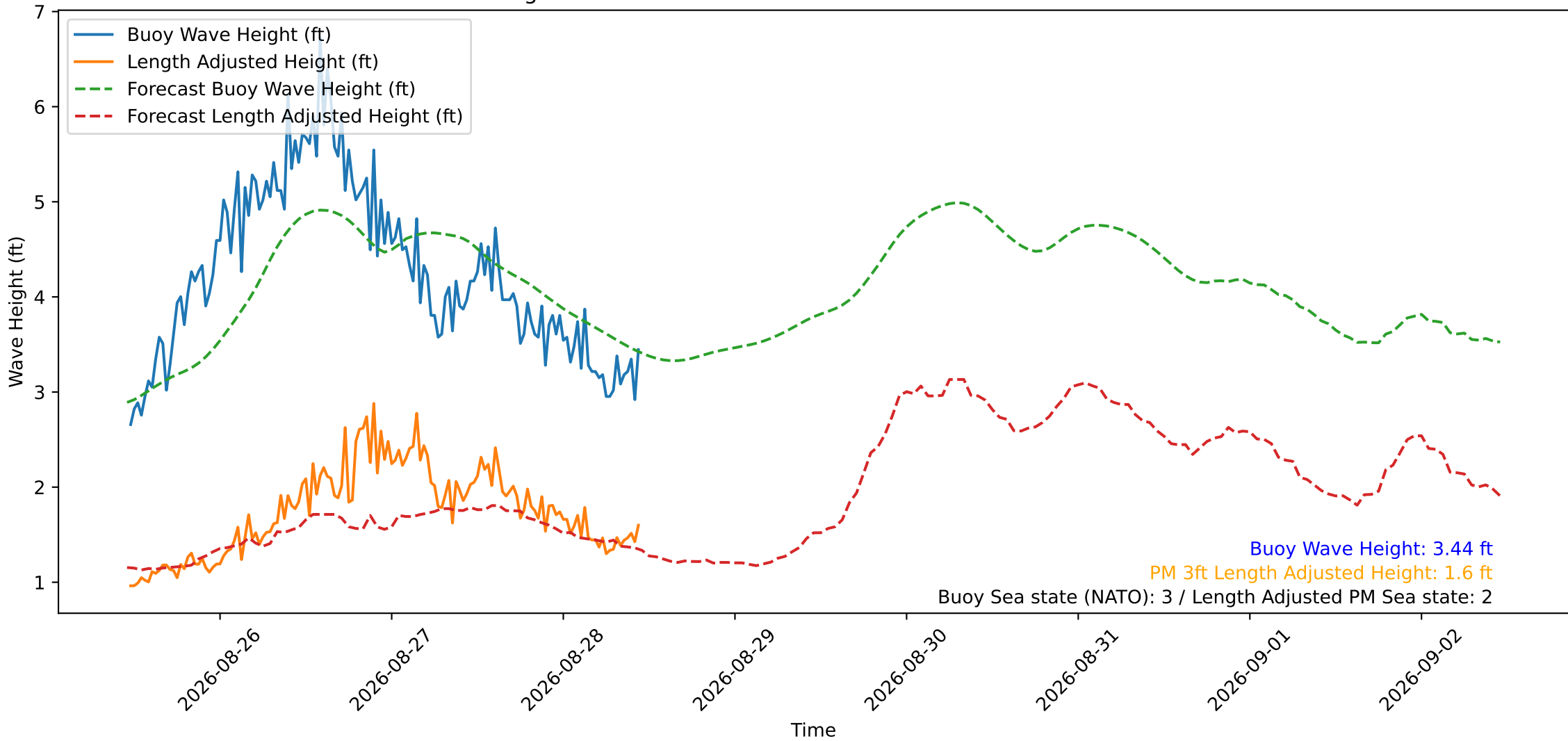
Wave Heights over Time for Oceanside Harbor at 2026-08-28 11:20:29
